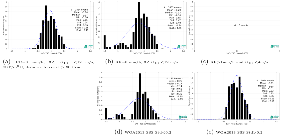
Figure 15: Normalized histogram of \Delta SSS (CCI SSS L4 Merged-OI v4.41 - 7-day running (ESA) - TSG (SAMOS)) for 5 different subdatasets corresponding to: RR=0 mm/h, 3 < U_{10} < 12 m/s, SST > 5°C, distance to coast > 800 km (a), RR=0 mm/h, 3 < U_{10} < 12 m/s (b), RR > 1mm/h and U_{10} < 4 m/s (c), WOA2013 SSS Std < 0.2 (d), WOA2013 SSS Std > 0.2 (e).
