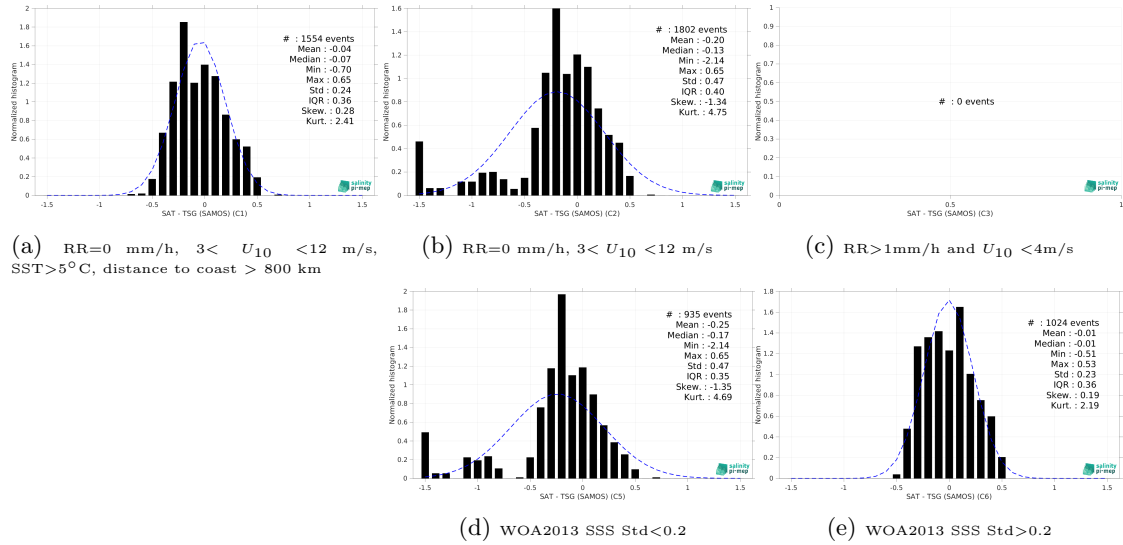
Figure 15: Normalized histogram of \Delta SSS (CCI SSS L4 Merged-OI v4.41 - 7-day running (ESA) - TSG (SAMOS)) for 5 different subdatasets corresponding to: RR=0 mm/h, 3 < U_{10} < 12 m/s, SST > 5°C, distance to coast > 800 km (a), RR=0 mm/h, 3 < U_{10} < 12 m/s (b), RR > 1mm/h and U_{10} < 4 m/s (c), WOA2013 SSS Std < 0.2 (d), WOA2013 SSS Std > 0.2 (e).
