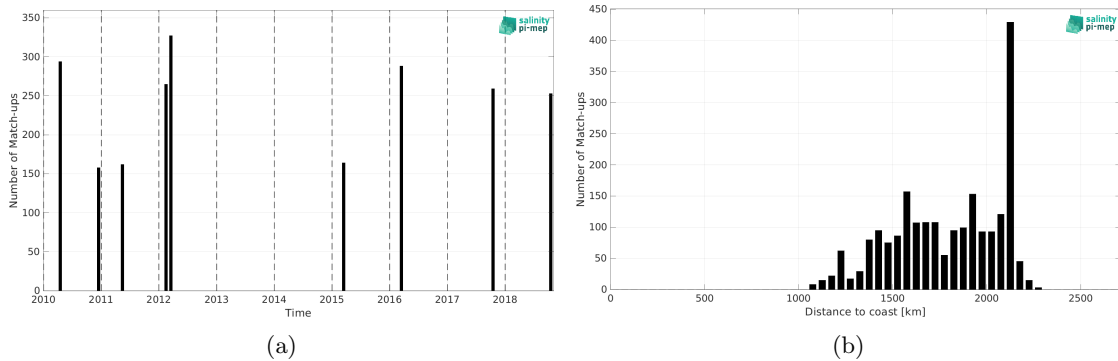
Figure 2: Number of match-ups between TSG (SAMOS) and CCI SSS L4 Merged-OI v4.41 - 7-day running (ESA) SSS as a function of time (a) and as function of the distance to coast (b) over the SPURS 2 Pi-MEP region and for the full satellite product period.
