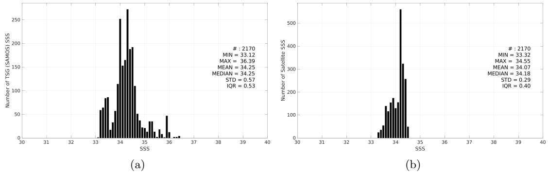
Figure 3: Histograms of SSS from TSG (SAMOS) (a) and CCI SSS L4 Merged-OI v4.41 - 7-day running (ESA) (b) considering all match-up pairs per bins of 0.1 over the SPURS 2 Pi-MEP region and for the full satellite product period.
