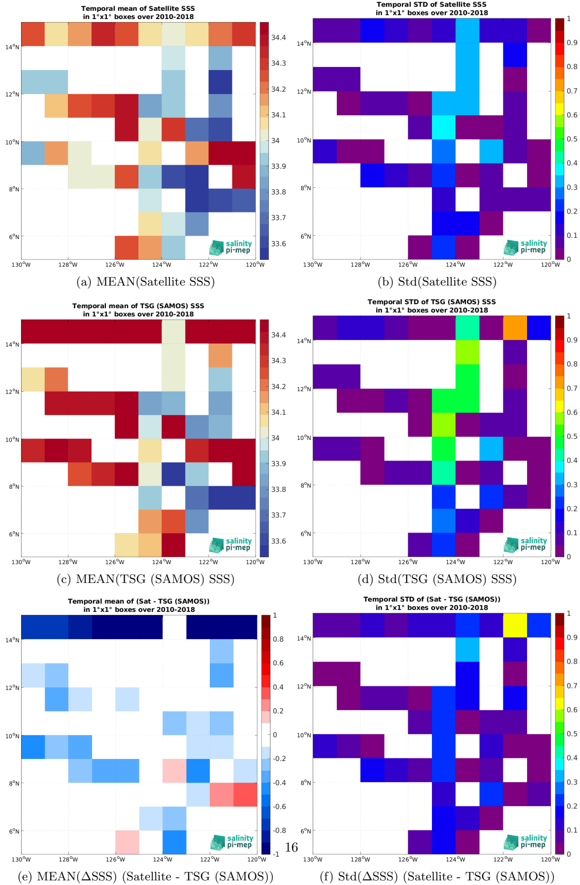
Figure 7: Temporal mean (left) and Std (right) of SSS from CCI SSS L4 Merged-OI v4.41 - 7-day running (ESA) (top), TSG (SAMOS) (middle), and of \Delta SSS (Satellite - TSG (SAMOS)). Only match-up pairs are used to generate these maps.
