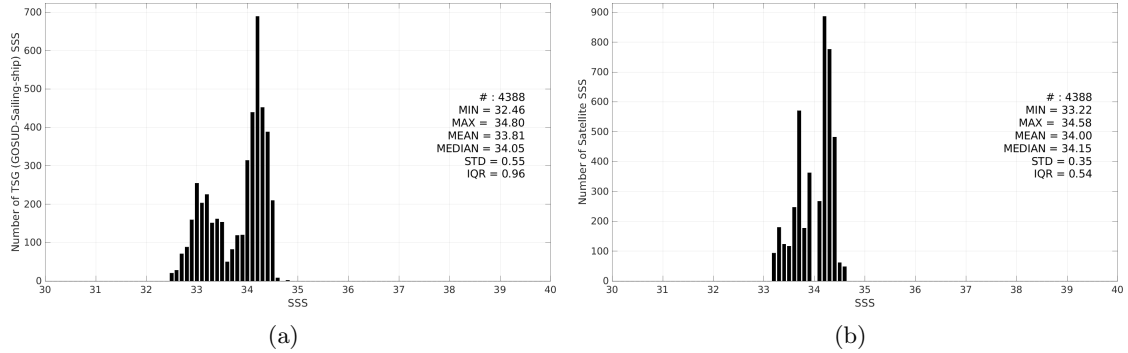
Figure 3: Histograms of SSS from TSG (GOSUD-Sailing-ship) (a) and CCI SSS L4 Merged-OI v4.41 - 7-day running (ESA) (b) considering all match-up pairs per bins of 0.1 over the SPURS 2 Pi-MEP region and for the full satellite product period.
