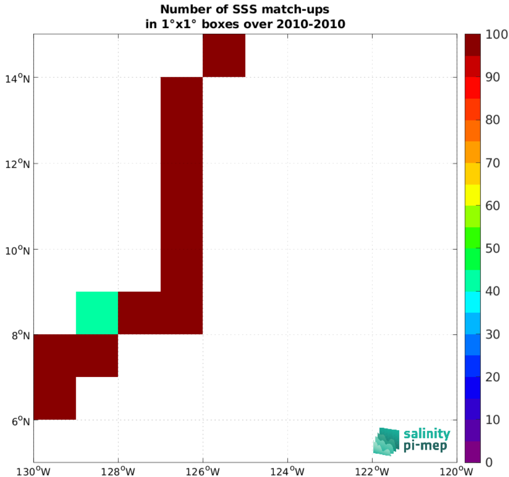
Figure 5: Number of SSS match-ups between TSG (GOSUD-Sailing-ship) SSS and the CCI SSS L4 Merged-OI v4.41 - 7-day running (ESA) SSS product for the SPURS 2 Pi-MEP region over 1^\circ \times 1^\circ boxes and for the full satellite product period.
