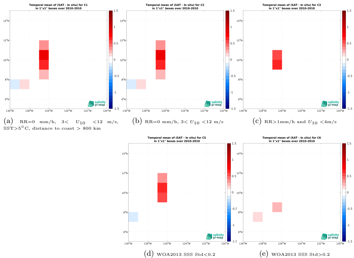
Figure 14: Temporal mean gridded over spatial boxes of size 1^\circ \times 1^\circ of \Delta\text{SSS} (CCI SSS L4 Merged-OI v4.41 - 7-day running (ESA) - TSG (GOSUD-Sailing-ship)) for 5 different subdatasets corresponding to:RR=0 mm/h, 3 < U_{10} < 12 m/s, SST >5^\circ\text{C} , distance to coast > 800 km (a), RR=0 mm/h, 3 < U_{10} < 12 m/s (b), RR >1 mm/h and U_{10} < 4 m/s (c), WOA2013 SSS Std <0.2 (d), WOA2013 SSS Std >0.2 (e).
