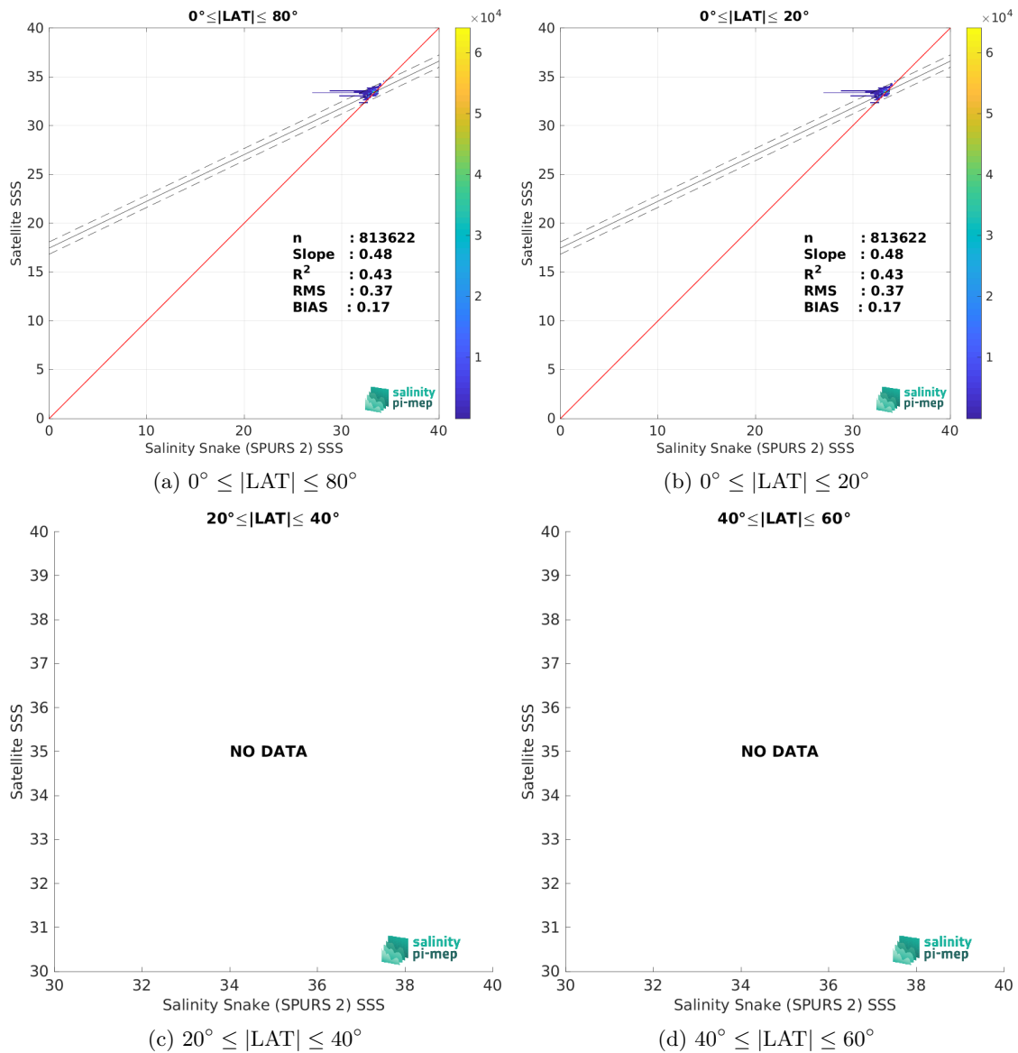
Figure 10: Contour maps of the concentration of CCI SSS L4 Merged-OI v4.41 - 7-day running (ESA) SSS (y-axis) versus Salinity Snake (SPURS 2) SSS (x-axis) at match-up pairs for different latitude bands. For each plot, the red line shows x=y . The black thin and dashed lines indicate a linear fit through the data cloud and the \pm 95\% confidence levels, respectively. The number match-up pairs n , the slope and R^2 coefficient of the linear fit, the root mean square (RMS) and the mean bias between satellite and in situ data are indicated for each latitude band in each plots.
