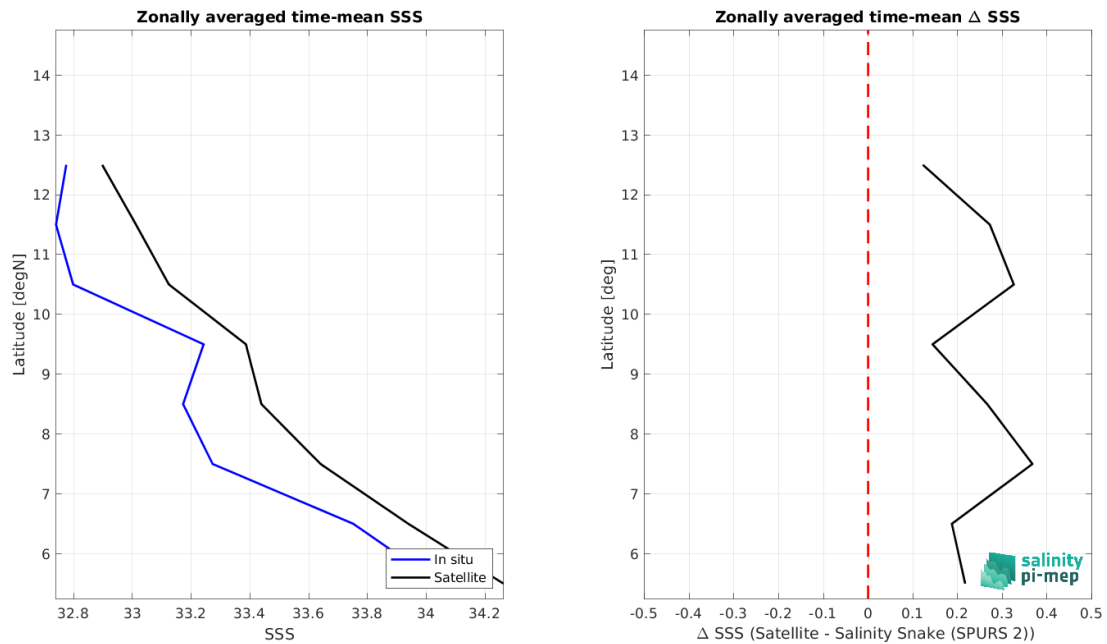
Figure 9: Left panel: Zonal mean SSS from CCI SSS L4 Merged-OI v4.41 - 7-day running (ESA) satellite product (black) and from Salinity Snake (SPURS 2) (blue). Right panel: Zonal mean of \Delta SSS (Satellite - Salinity Snake (SPURS 2)) for all the collected Pi-MEP match-up pairs estimated over the full satellite product period.
