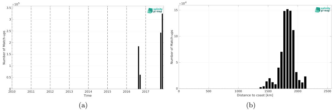
Figure 2: Number of match-ups between Salinity Snake (SPURS 2) and CCI SSS L4 Merged-OI v4.41 - 7-day running (ESA) SSS as a function of time (a) and as function of the distance to coast (b) over the SPURS 2 Pi-MEP region and for the full satellite product period.
