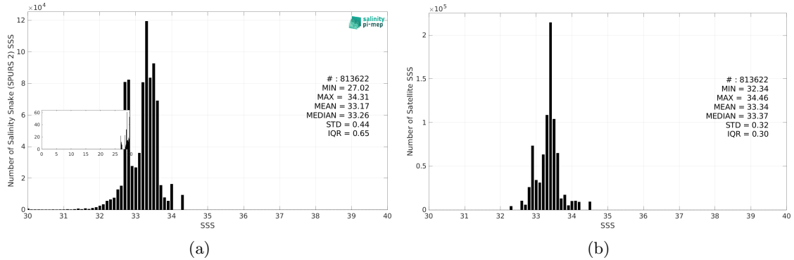
Figure 3: Histograms of SSS from Salinity Snake (SPURS 2) (a) and CCI SSS L4 Merged-OI v4.41 - 7-day running (ESA) (b) considering all match-up pairs per bins of 0.1 over the SPURS 2 Pi-MEP region and for the full satellite product period.
