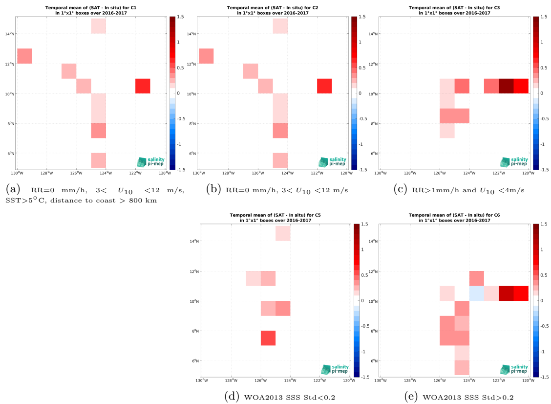
Figure 14: Temporal mean gridded over spatial boxes of size 1^\circ \times 1^\circ of \Delta SSS (CCI SSS L4 Merged-OI v4.41 - 7-day running (ESA) - Salinity Snake (SPURS 2)) for 5 different subdatasets corresponding to:RR=0 mm/h, 3 < U_{10} < 12 m/s, SST >5^\circ C, distance to coast > 800 km (a), RR=0 mm/h, 3 < U_{10} < 12 m/s (b), RR >1 mm/h and U_{10} < 4 m/s (c), WOA2013 SSS Std <0.2 (d), WOA2013 SSS Std >0.2 (e).
