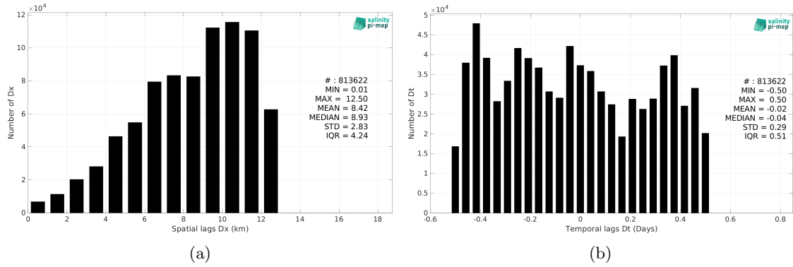
Figure 6: Histograms of the spatial (a) and temporal (b) lags between the location/time of the Salinity Snake (SPURS 2) measurement and the date of the corresponding CCI SSS L4 Merged-OI v4.41 - 7-day running (ESA) SSS pixel.
