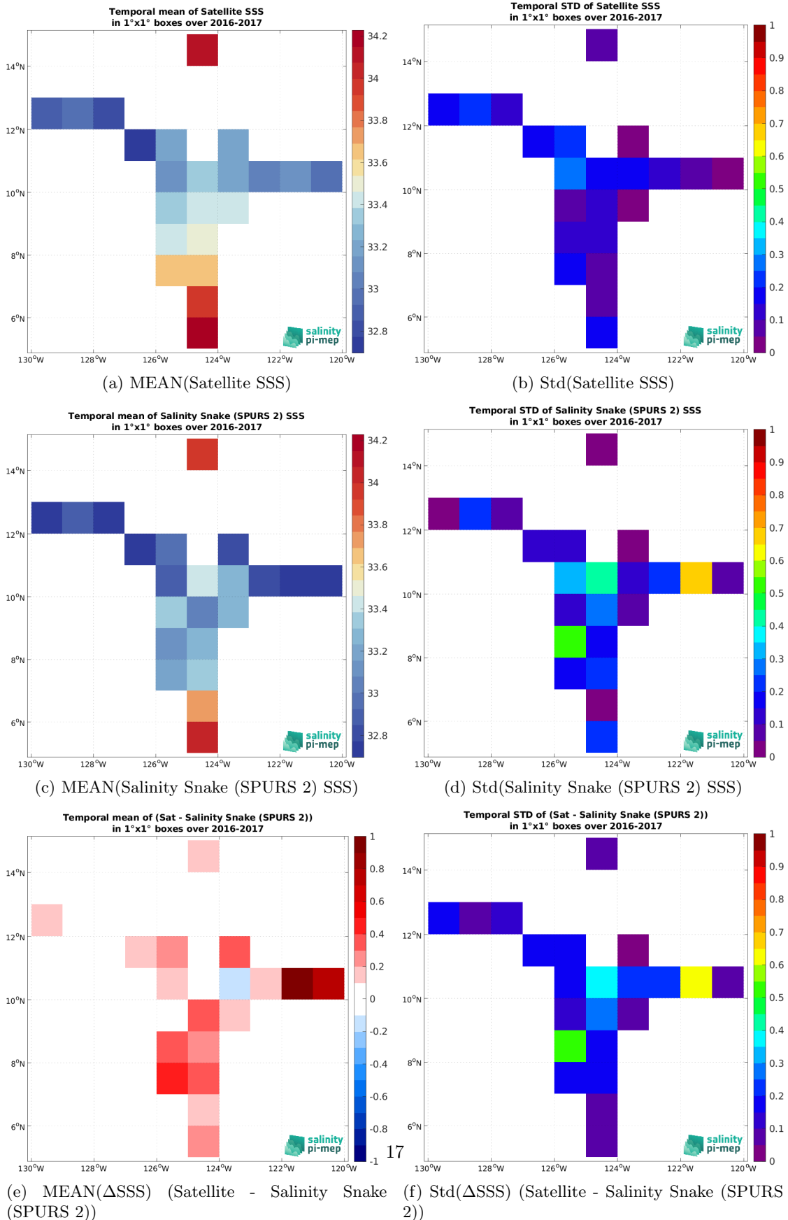
Figure 7: Temporal mean (left) and Std (right) of SSS from CCI SSS L4 Merged-OI v4.41 - 7-day running (ESA) (top), Salinity Snake (SPURS 2) (middle), and of \Delta SSS (Satellite - Salinity Snake (SPURS 2)). Only match-up pairs are used to generate these maps.
