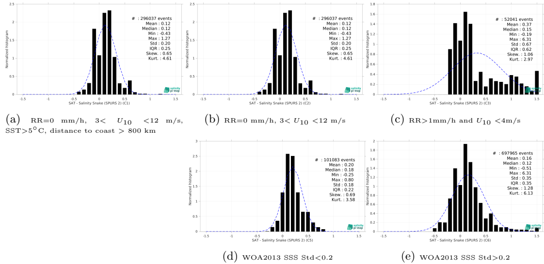
Figure 15: Normalized histogram of \Delta SSS (CCI SSS L4 Merged-OI v4.41 - 7-day running (ESA) - Salinity Snake (SPURS 2)) for 5 different subdatasets corresponding to: RR=0 mm/h, 3 < U_{10} < 12 m/s, SST > 5°C, distance to coast > 800 km (a), RR=0 mm/h, 3 < U_{10} < 12 m/s (b), RR > 1mm/h and U_{10} < 4 m/s (c), WOA2013 SSS Std < 0.2 (d), WOA2013 SSS Std > 0.2 (e).
