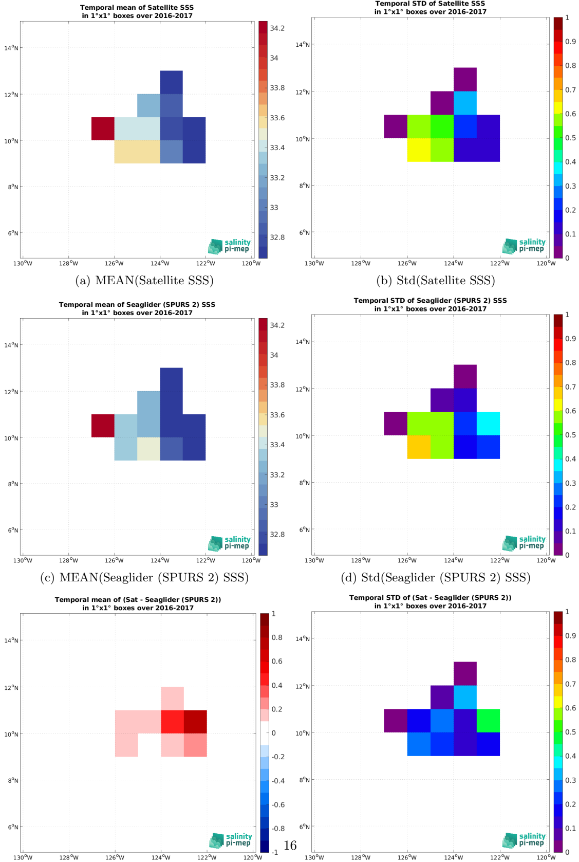
Figure 7: Temporal mean (left) and Std (right) of SSS from CCI SSS L4 Merged-OI v4.41 - 7-day running (ESA) (top), Seaglider (SPURS 2) (middle), and of \Delta SSS (Satellite - Seaglider (SPURS 2)). Only match-up pairs are used to generate these maps.
