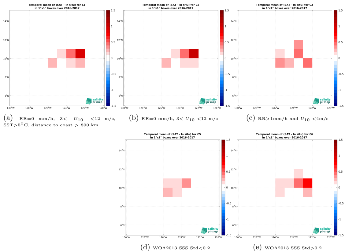
Figure 14: Temporal mean gridded over spatial boxes of size 1^\circ \times 1^\circ of \Delta\text{SSS} (CCI SSS L4 Merged-OI v4.41 - 7-day running (ESA) - Seaglider (SPURS 2)) for 5 different subdatasets corresponding to:RR=0 mm/h, 3 < U_{10} < 12 m/s, SST>5°C, distance to coast > 800 km (a), RR=0 mm/h, 3 < U_{10} < 12 m/s (b), RR>1mm/h and U_{10} < 4 m/s (c), WOA2013 SSS Std<0.2 (d), WOA2013 SSS Std>0.2 (e).
