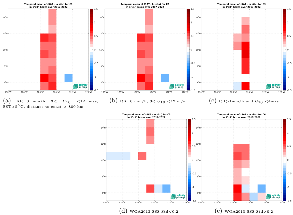
Figure 14: Temporal mean gridded over spatial boxes of size 1^\circ \times 1^\circ of \Delta\text{SSS} (CCI SSS L4 Merged-OI v4.41 - 7-day running (ESA) - Saildrone) for 5 different subdatasets corresponding to:RR=0 mm/h, 3 < U_{10} < 12 m/s, SST>5°C, distance to coast > 800 km (a), RR=0 mm/h, 3 < U_{10} < 12 m/s (b), RR>1mm/h and U_{10} < 4 m/s (c), WOA2013 SSS Std<0.2 (d), WOA2013 SSS Std>0.2 (e).
