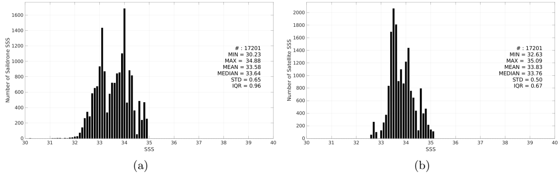
Figure 3: Histograms of SSS from Saildrone (a) and CCI SSS L4 Merged-OI v4.41 - 7-day running (ESA) (b) considering all match-up pairs per bins of 0.1 over the SPURS 2 Pi-MEP region and for the full satellite product period.
