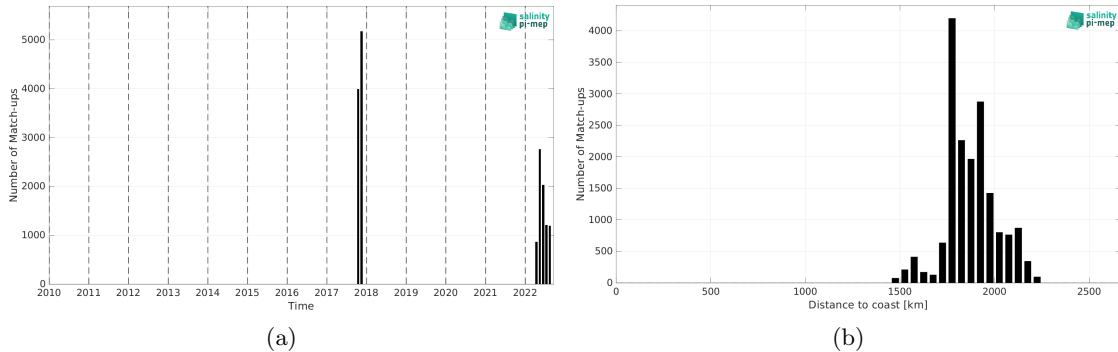
Figure 2: Number of match-ups between Saildrone and CCI SSS L4 Merged-OI v4.41 - 7-day running (ESA) SSS as a function of time (a) and as function of the distance to coast (b) over the SPURS 2 Pi-MEP region and for the full satellite product period.
