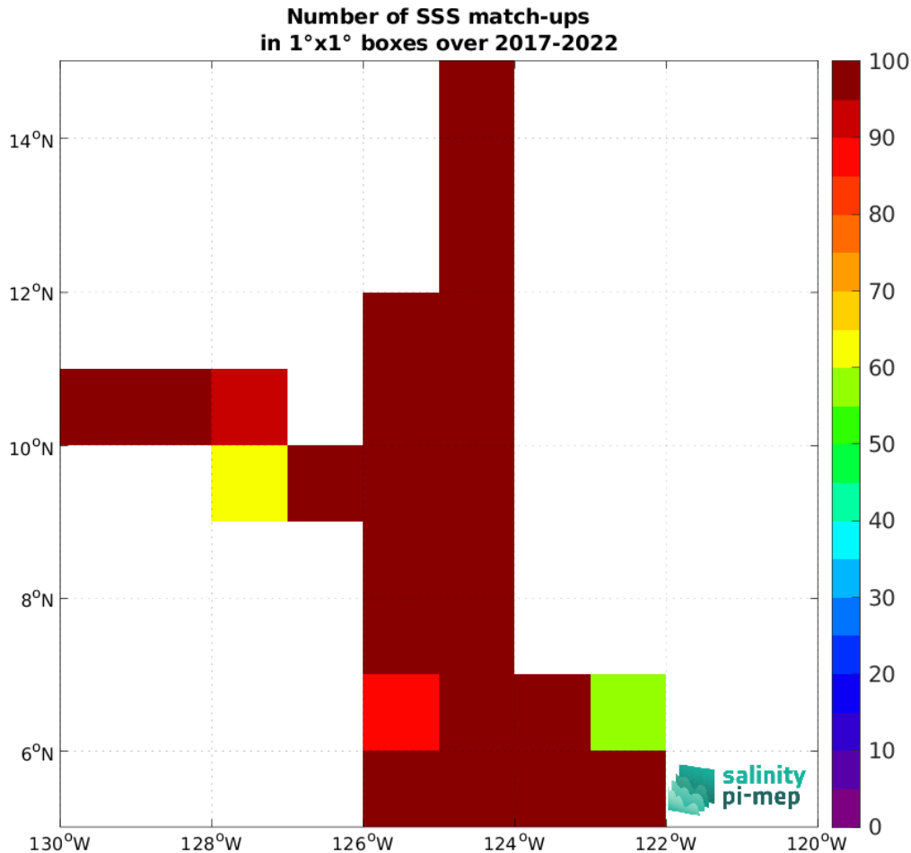
Figure 5: Number of SSS match-ups between Saildrone SSS and the CCI SSS L4 Merged-OI v4.41 - 7-day running (ESA) SSS product for the SPURS 2 Pi-MEP region over 1^\circ \times 1^\circ boxes and for the full satellite product period.
