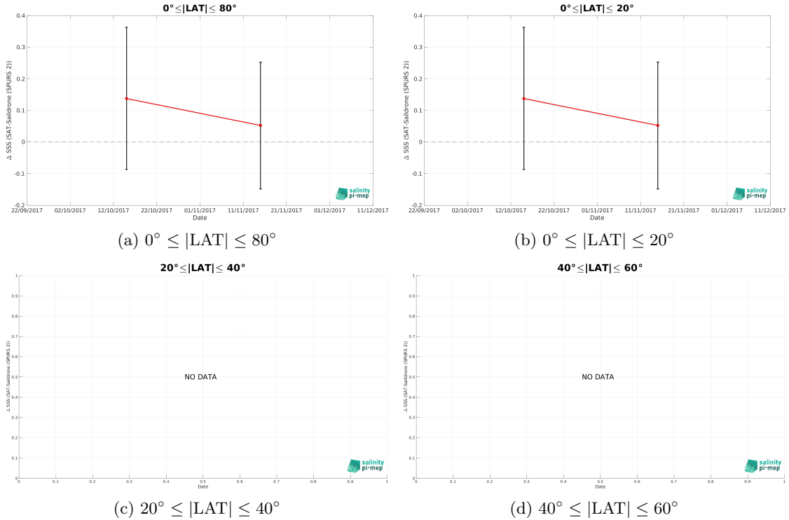
Figure 11: Monthly median (red curves) of \Delta SSS (Satellite - Sairdron (SPURS 2)) and \pm 1 Std (black vertical thick bars) as function of time for all the collected Pi-MEP match-up pairs estimated over the SPURS 2 Pi-MEP region and for the full satellite product period are shown for different latitude bands: (a) 80^\circ\text{S}-80^\circ\text{N} , (b) 20^\circ\text{S}-20^\circ\text{N} , (c) 40^\circ\text{S}-20^\circ\text{S} and 20^\circ\text{N}-40^\circ\text{N} and (d) 60^\circ\text{S}-40^\circ\text{S} and 40^\circ\text{N}-60^\circ\text{N} .
