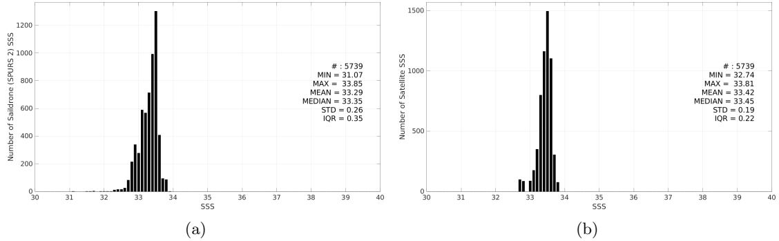
Figure 3: Histograms of SSS from Saildrone (SPURS 2) (a) and CCI SSS L4 Merged-OI v4.41 - 7-day running (ESA) (b) considering all match-up pairs per bins of 0.1 over the SPURS 2 Pi-MEP region and for the full satellite product period.
