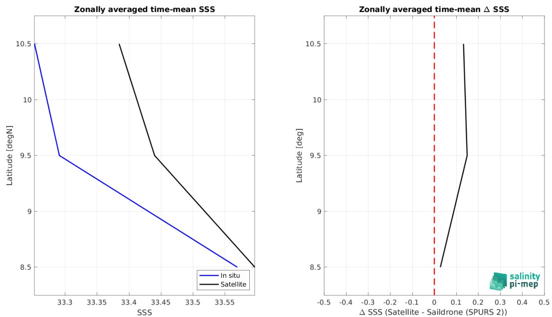
Figure 9: Left panel: Zonal mean SSS from CCI SSS L4 Merged-OI v4.41 - 7-day running (ESA) satellite product (black) and from Sairdron (SPURS 2) (blue). Right panel: Zonal mean of \Delta SSS (Satellite - Sairdron (SPURS 2)) for all the collected Pi-MEP match-up pairs estimated over the full satellite product period.
