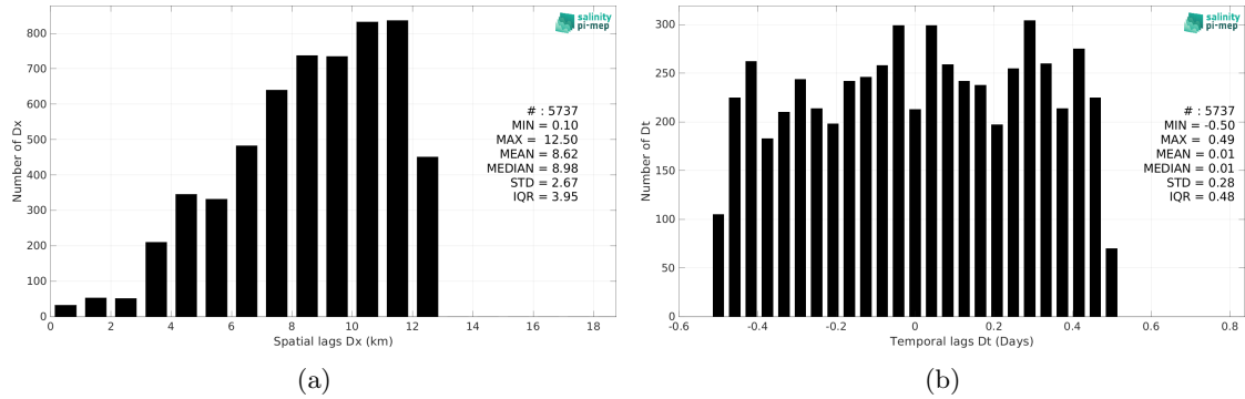
Figure 6: Histograms of the spatial (a) and temporal (b) lags between the location/time of the Saildrone (SPURS 2) measurement and the date of the corresponding CCI SSS L4 Merged-OI v4.41 - 7-day running (ESA) SSS pixel.
