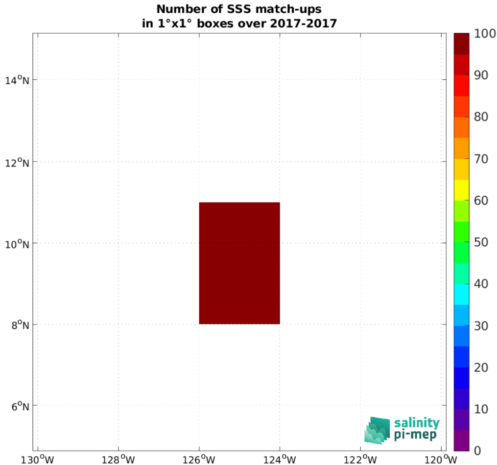
Figure 5: Number of SSS match-ups between Saildrone (SPURS 2) SSS and the CCI SSS L4 Merged-OI v4.41 - 7-day running (ESA) SSS product for the SPURS 2 Pi-MEP region over 1^\circ \times 1^\circ boxes and for the full satellite product period.
