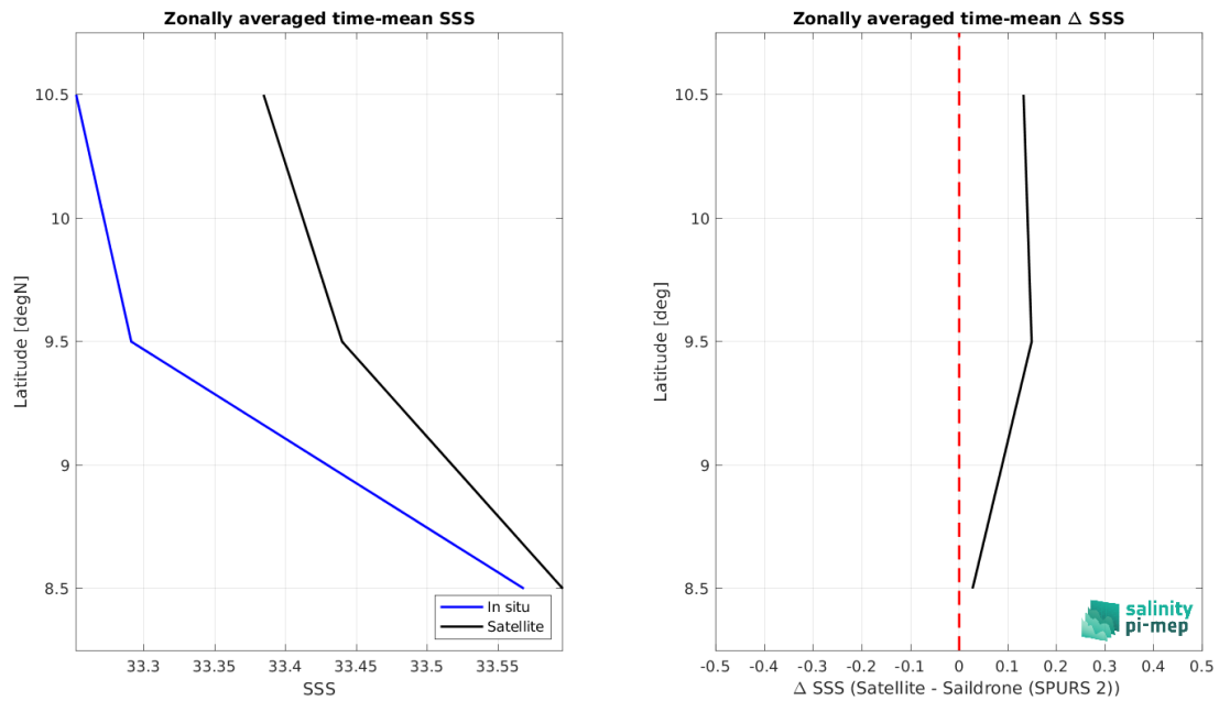
Figure 9: Left panel: Zonal mean SSS from CCI SSS L4 Merged-OI v4.41 - 7-day running (ESA) satellite product (black) and from Sairdrone (SPURS 2) (blue). Right panel: Zonal mean of \Delta SSS (Satellite - Sairdrone (SPURS 2)) for all the collected Pi-MEP match-up pairs estimated over the full satellite product period.
