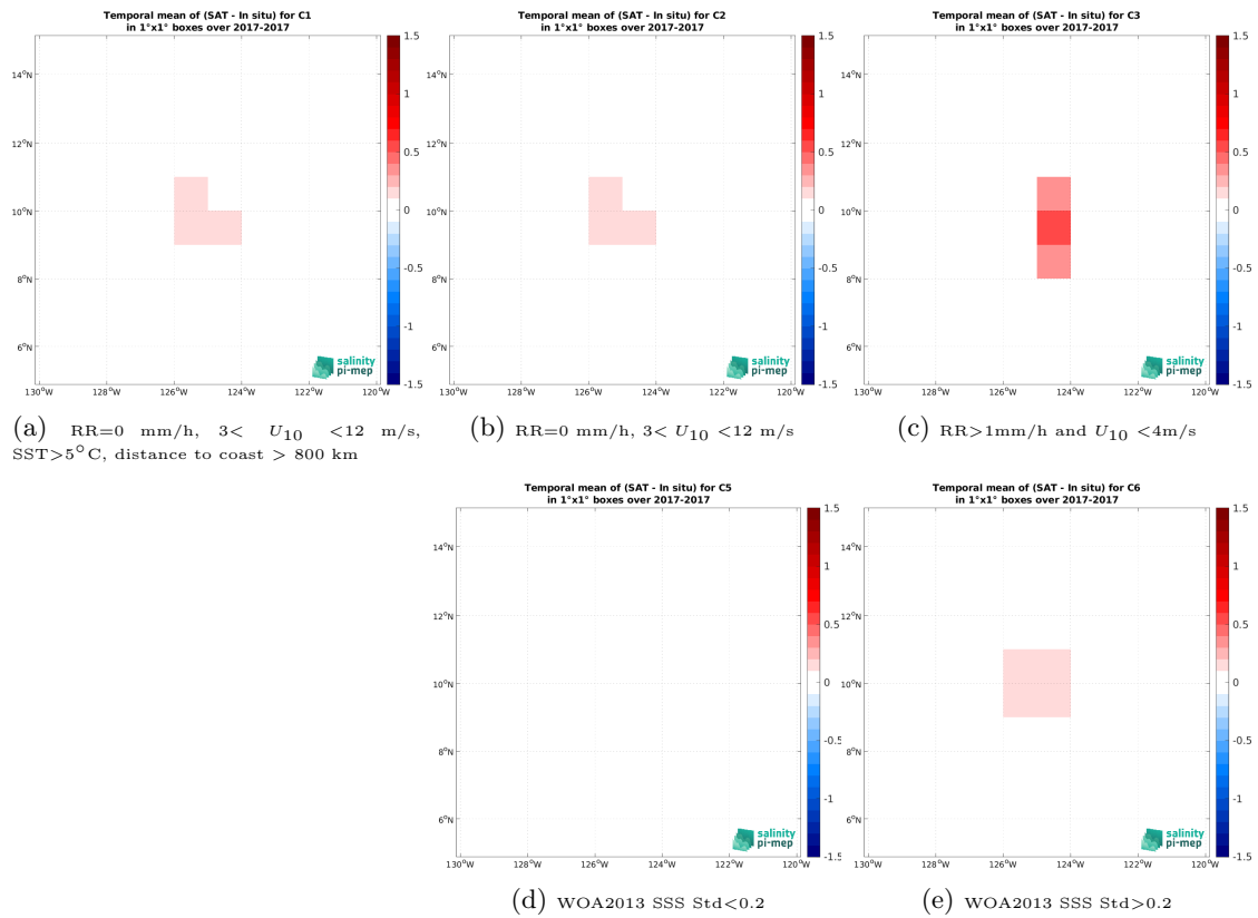
Figure 14: Temporal mean gridded over spatial boxes of size 1^\circ \times 1^\circ of \Delta\text{SSS} (CCI SSS L4 Merged-OI v4.41 - 7-day running (ESA) - Saildrone (SPURS 2)) for 5 different subdatasets corresponding to:RR=0 mm/h, 3 < U_{10} < 12 m/s, SST>5°C, distance to coast > 800 km (a), RR=0 mm/h, 3 < U_{10} < 12 m/s (b), RR>1mm/h and U_{10} < 4 m/s (c), WOA2013 SSS Std<0.2 (d), WOA2013 SSS Std>0.2 (e).
