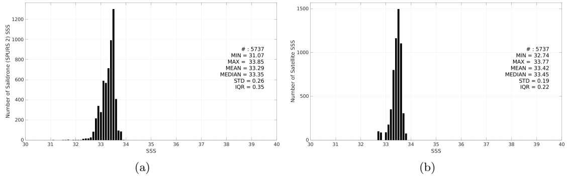
Figure 3: Histograms of SSS from Sairdrone (SPURS 2) (a) and CCI SSS L4 Merged-OI v4.41 - 7-day running (ESA) (b) considering all match-up pairs per bins of 0.1 over the SPURS 2 Pi-MEP region and for the full satellite product period.
