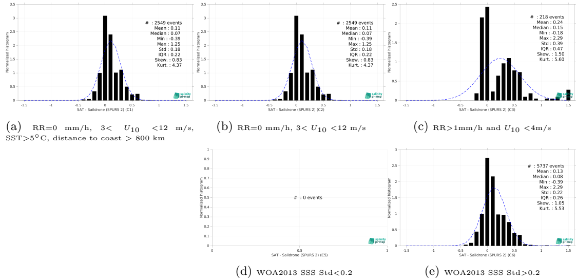
Figure 15: Normalized histogram of \Delta SSS (CCI SSS L4 Merged-OI v4.41 - 7-day running (ESA) - Saildrone (SPURS 2)) for 5 different subdatasets corresponding to: RR=0 mm/h, 3 < U_{10} < 12 m/s, SST>5°C, distance to coast > 800 km (a), RR=0 mm/h, 3 < U_{10} < 12 m/s (b), RR>1mm/h and U_{10} < 4 m/s (c), WOA2013 SSS Std<0.2 (d), WOA2013 SSS Std>0.2 (e).
