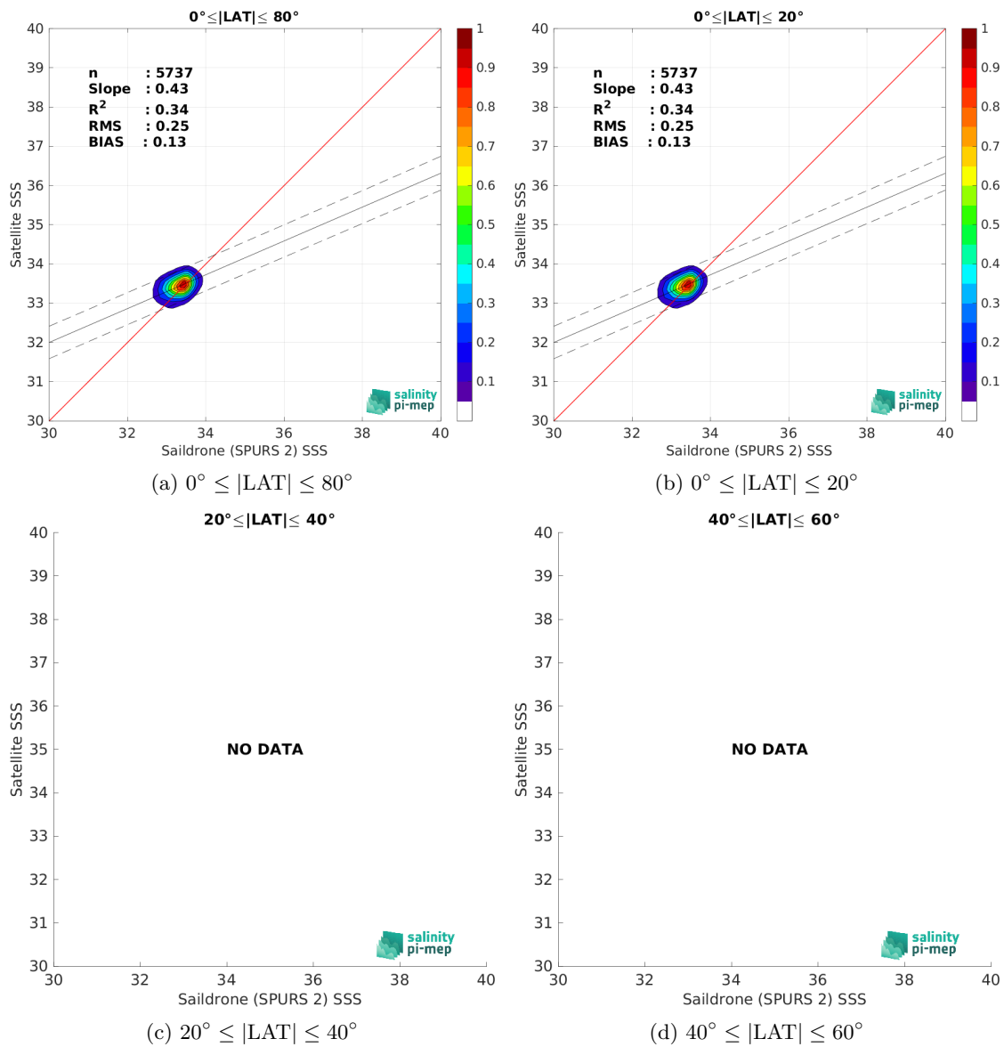
Figure 10: Contour maps of the concentration of CCI SSS L4 Merged-OI v4.41 - 7-day running (ESA) SSS (y-axis) versus Saildrone (SPURS 2) SSS (x-axis) at match-up pairs for different latitude bands. For each plot, the red line shows x=y . The black thin and dashed lines indicate a linear fit through the data cloud and the \pm 95\% confidence levels, respectively. The number match-up pairs n , the slope and R^2 coefficient of the linear fit, the root mean square (RMS) and the mean bias between satellite and in situ data are indicated for each latitude band in each plots.
