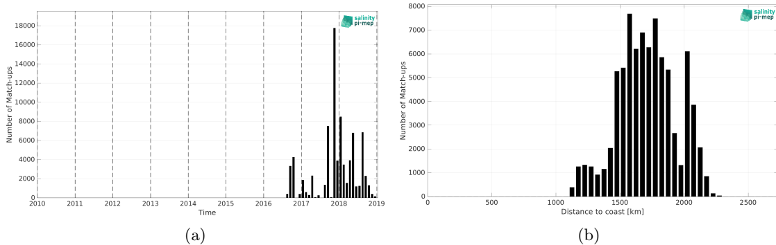
Figure 2: Number of match-ups between Surface drifters and CCI SSS L4 Merged-OI v4.41 - 7-day running (ESA) SSS as a function of time (a) and as function of the distance to coast (b) over the SPURS 2 Pi-MEP region and for the full satellite product period.
