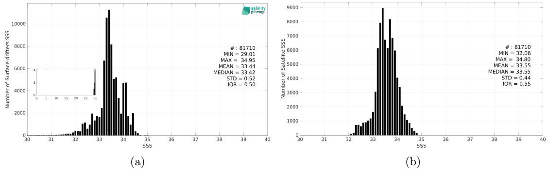
Figure 3: Histograms of SSS from Surface drifters (a) and CCI SSS L4 Merged-OI v4.41 - 7-day running (ESA) (b) considering all match-up pairs per bins of 0.1 over the SPURS 2 Pi-MEP region and for the full satellite product period.
