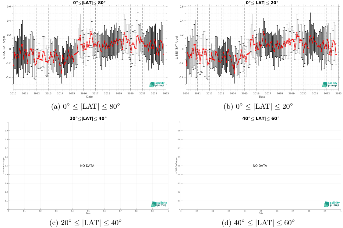
Figure 11: Monthly median (red curves) of \Delta SSS (Satellite - Argo) and \pm 1 Std (black vertical thick bars) as function of time for all the collected Pi-MEP match-up pairs estimated over the SPURS 2 Pi-MEP region and for the full satellite product period are shown for different latitude bands: (a) 80°S-80°N, (b) 20°S-20°N, (c) 40°S-20°S and 20°N-40°N and (d) 60°S-40°S and 40°N-60°N.
