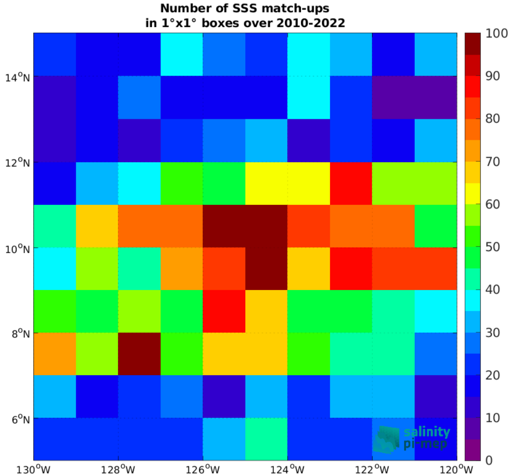
Figure 5: Number of SSS match-ups between Argo SSS and the CCI SSS L4 Merged-OI v4.41 - 7-day running (ESA) SSS product for the SPURS 2 Pi-MEP region over 1^\circ \times 1^\circ boxes and for the full satellite product period.
