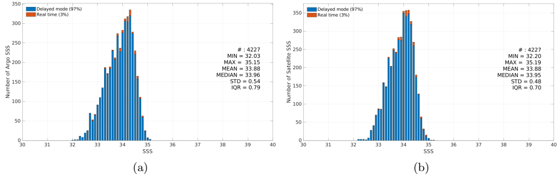
Figure 3: Histograms of SSS from Argo (a) and CCI SSS L4 Merged-OI v4.41 - 7-day running (ESA) (b) considering all match-up pairs per bins of 0.1 over the SPURS 2 Pi-MEP region and for the full satellite product period.
