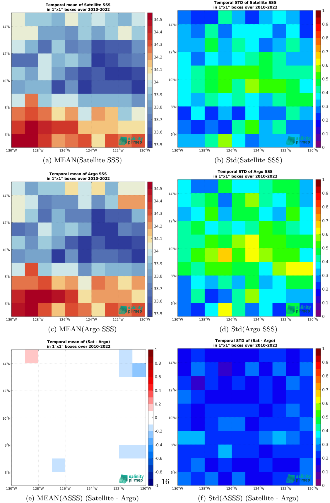
Figure 7: Temporal mean (left) and Std (right) of SSS from CCI SSS L4 Merged-OI v4.41 - 7-day running (ESA) (top), Argo (middle), and of \Delta SSS (Satellite - Argo). Only match-up pairs are used to generate these maps.
