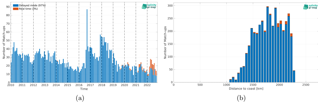
Figure 2: Number of match-ups between Argo and CCI SSS L4 Merged-OI v4.41 - 7-day running (ESA) SSS as a function of time (a) and as function of the distance to coast (b) over the SPURS 2 Pi-MEP region and for the full satellite product period.
