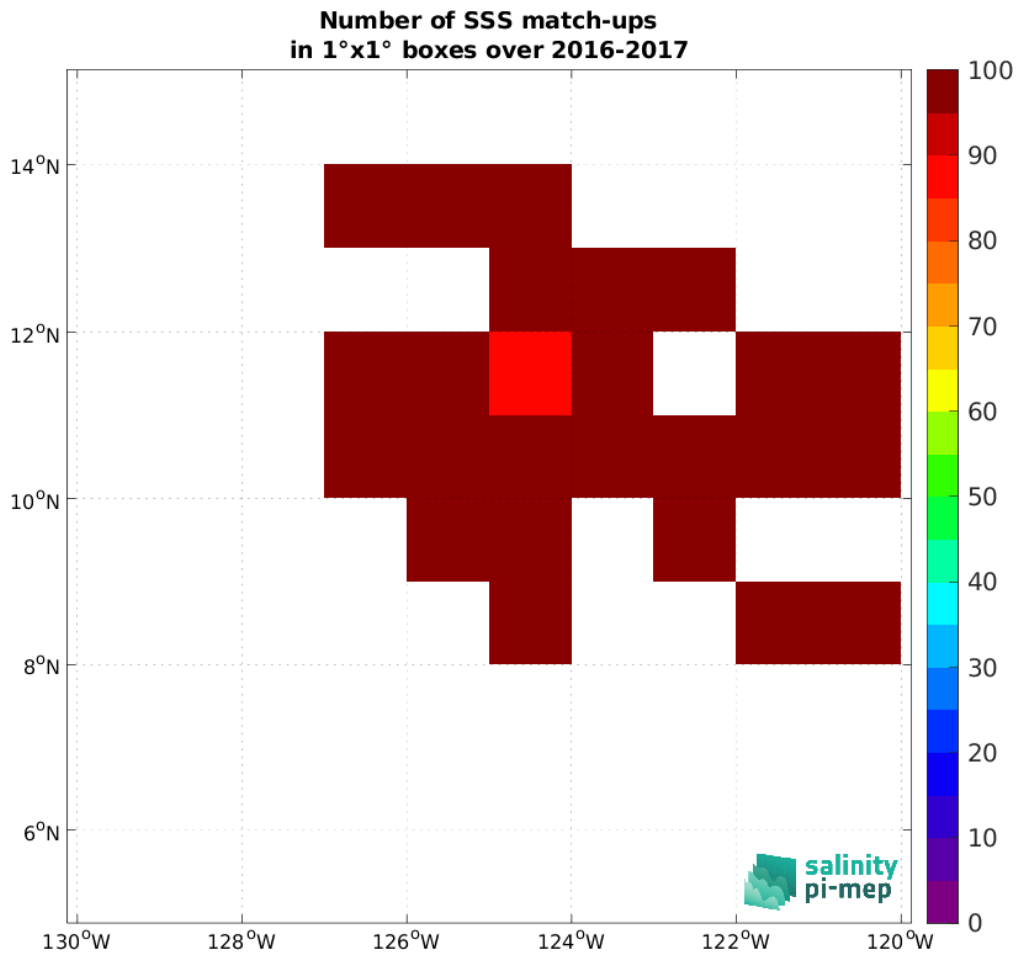
Figure 5: Number of SSS match-ups between Waveglider (SPURS 2) SSS and the CCI SSS L4 Merged-OI v4.41 - 30-day running (ESA) SSS product for the SPURS 2 Pi-MEP region over 1^\circ \times 1^\circ boxes and for the full satellite product period.
