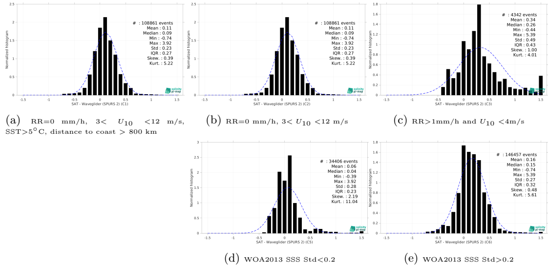
Figure 15: Normalized histogram of \Delta SSS (CCI SSS L4 Merged-OI v4.41 - 30-day running (ESA) - Waveglider (SPURS 2)) for 5 different subdatasets corresponding to: RR=0 mm/h, 3 < U_{10} < 12 m/s, SST>5°C, distance to coast > 800 km (a), RR=0 mm/h, 3 < U_{10} < 12 m/s (b), RR>1mm/h and U_{10} < 4 m/s (c), WOA2013 SSS Std<0.2 (d), WOA2013 SSS Std>0.2 (e).
