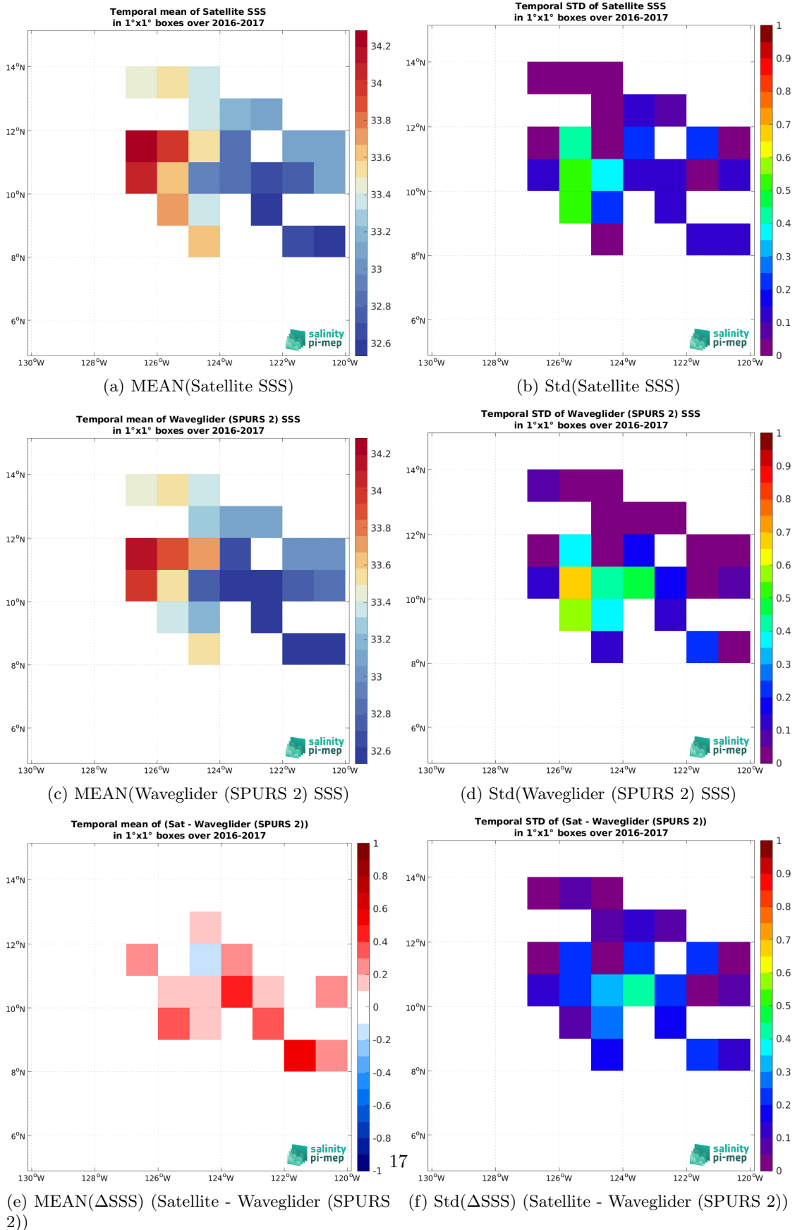
Figure 7: Temporal mean (left) and Std (right) of SSS from CCI SSS L4 Merged-OI v4.41 - 30-day running (ESA) (top), Waveglider (SPURS 2) (middle), and of \Delta SSS (Satellite - Waveglider (SPURS 2)). Only match-up pairs are used to generate these maps.
