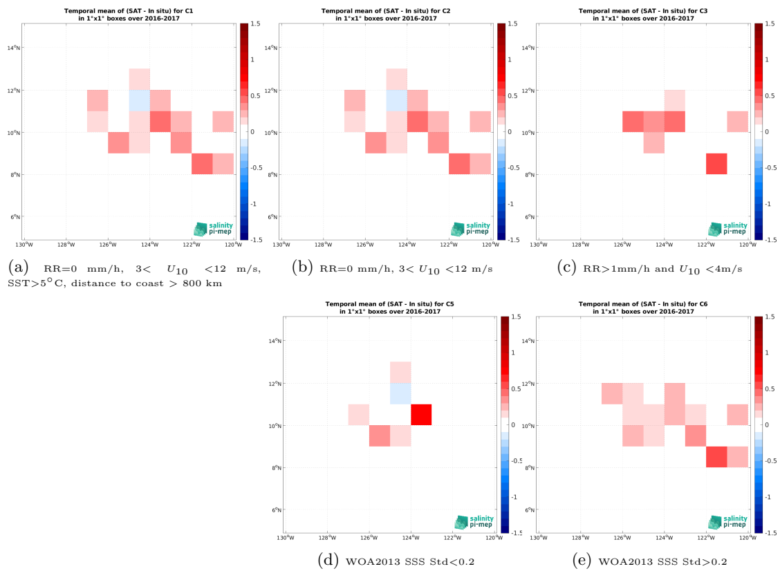
Figure 14: Temporal mean gridded over spatial boxes of size 1^\circ \times 1^\circ of \Delta SSS (CCI SSS L4 Merged-OI v4.41 - 30-day running (ESA) - Waveglider (SPURS 2)) for 5 different subdatasets corresponding to:RR=0 mm/h, 3 < U_{10} < 12 m/s, SST >5^\circ C, distance to coast > 800 km (a), RR=0 mm/h, 3 < U_{10} < 12 m/s (b), RR >1 mm/h and U_{10} < 4 m/s (c), WOA2013 SSS Std <0.2 (d), WOA2013 SSS Std >0.2 (e).
