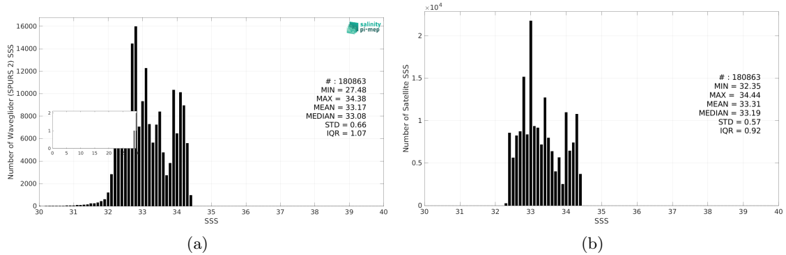
Figure 3: Histograms of SSS from Waveglider (SPURS 2) (a) and CCI SSS L4 Merged-OI v4.41 - 30-day running (ESA) (b) considering all match-up pairs per bins of 0.1 over the SPURS 2 Pi-MEP region and for the full satellite product period.
