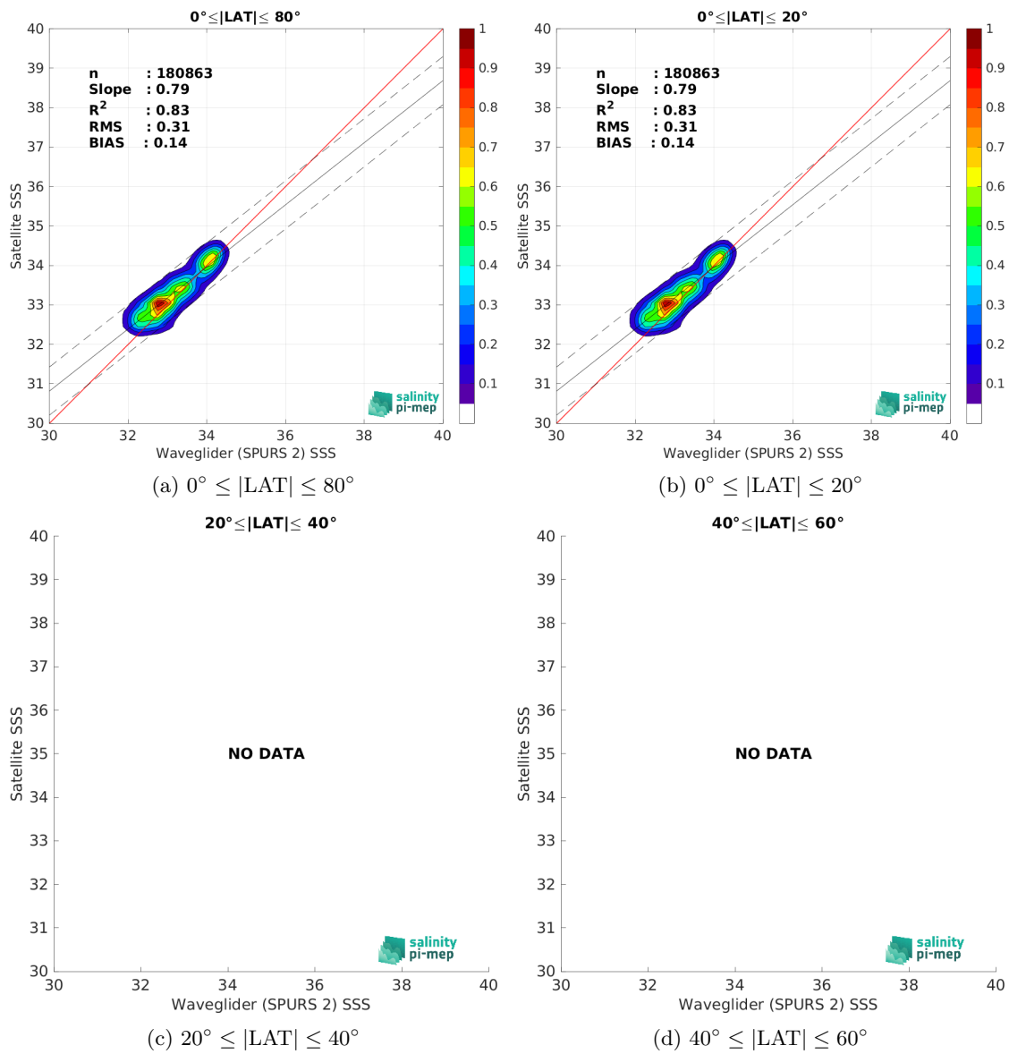
Figure 10: Contour maps of the concentration of CCI SSS L4 Merged-OI v4.41 - 30-day running (ESA) SSS (y-axis) versus Waveglider (SPURS 2) SSS (x-axis) at match-up pairs for different latitude bands. For each plot, the red line shows x=y . The black thin and dashed lines indicate a linear fit through the data cloud and the \pm 95\% confidence levels, respectively. The number match-up pairs n , the slope and R^2 coefficient of the linear fit, the root mean square (RMS) and the mean bias between satellite and in situ data are indicated for each latitude band in each plots.
