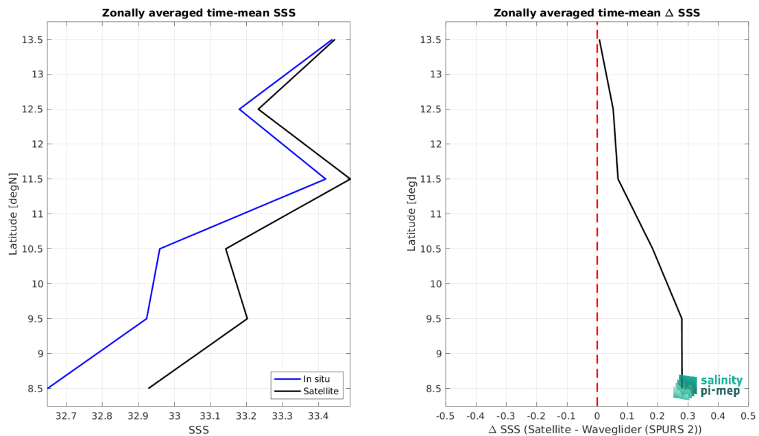
Figure 9: Left panel: Zonal mean SSS from CCI SSS L4 Merged-OI v4.41 - 30-day running (ESA) satellite product (black) and from Waveglider (SPURS 2) (blue). Right panel: Zonal mean of \Delta SSS (Satellite - Waveglider (SPURS 2)) for all the collected Pi-MEP match-up pairs estimated over the full satellite product period.
