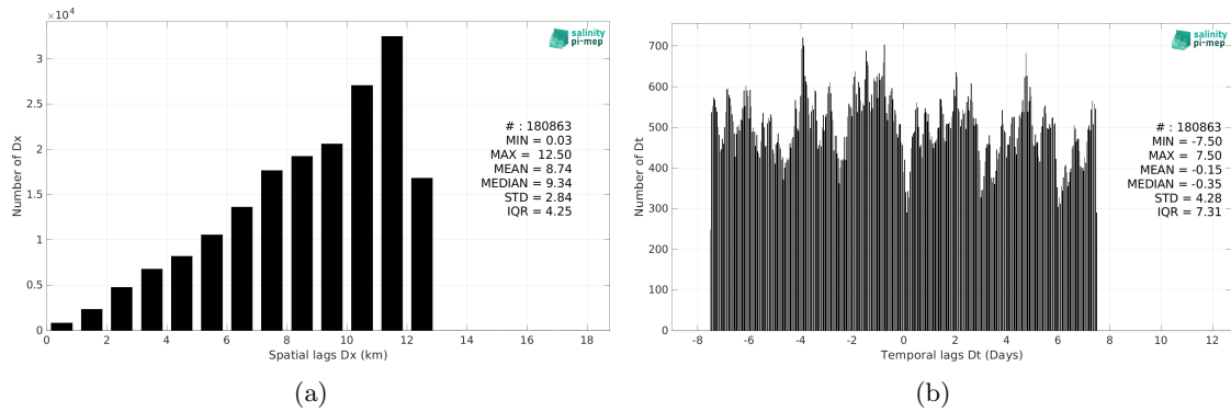
Figure 6: Histograms of the spatial (a) and temporal (b) lags between the location/time of the Waveglider (SPURS 2) measurement and the date of the corresponding CCI SSS L4 Merged-OI v4.41 - 30-day running (ESA) SSS pixel.
