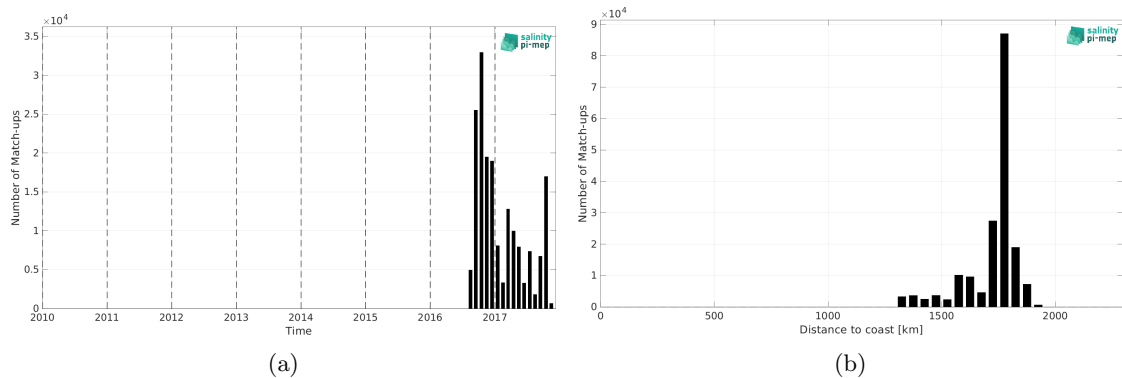
Figure 2: Number of match-ups between Waveglider (SPURS 2) and CCI SSS L4 Merged-OI v4.41 - 30-day running (ESA) SSS as a function of time (a) and as function of the distance to coast (b) over the SPURS 2 Pi-MEP region and for the full satellite product period.
