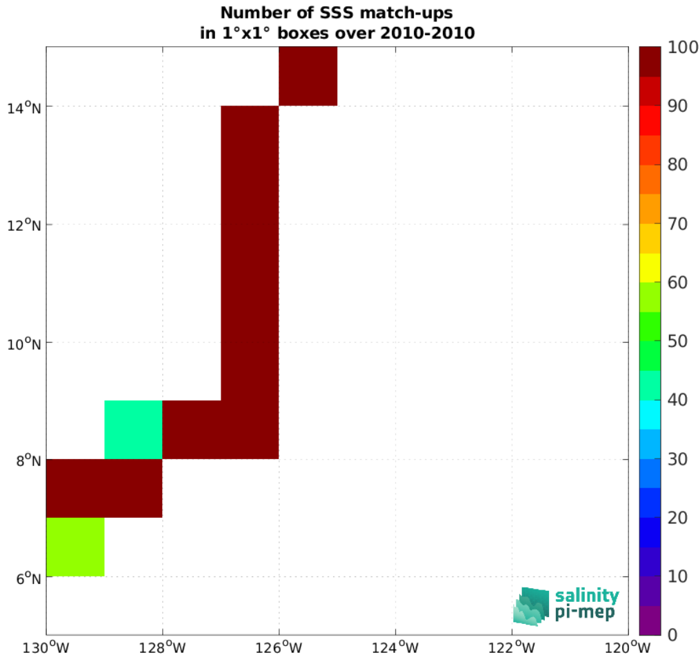
Figure 5: Number of SSS match-ups between TSG (GOSUD-Sailing-ship) SSS and the CCI SSS L4 Merged-OI v4.41 - 30-day running (ESA) SSS product for the SPURS 2 Pi-MEP region over 1^\circ \times 1^\circ boxes and for the full satellite product period.
