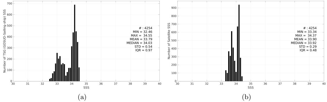
Figure 3: Histograms of SSS from TSG (GOSUD-Sailing-ship) (a) and CCI SSS L4 Merged-OI v4.41 - 30-day running (ESA) (b) considering all match-up pairs per bins of 0.1 over the SPURS 2 Pi-MEP region and for the full satellite product period.
