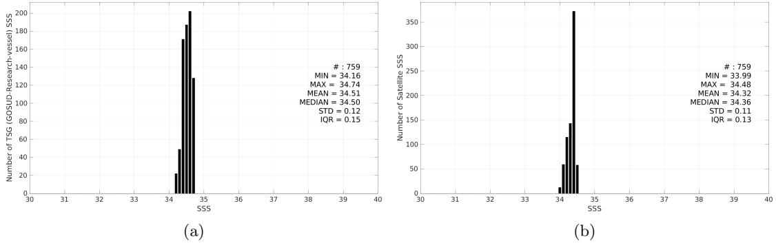
Figure 3: Histograms of SSS from TSG (GOSUD-Research-vessel) (a) and CCI SSS L4 Merged-OI v4.41 - 30-day running (ESA) (b) considering all match-up pairs per bins of 0.1 over the SPURS 2 Pi-MEP region and for the full satellite product period.
