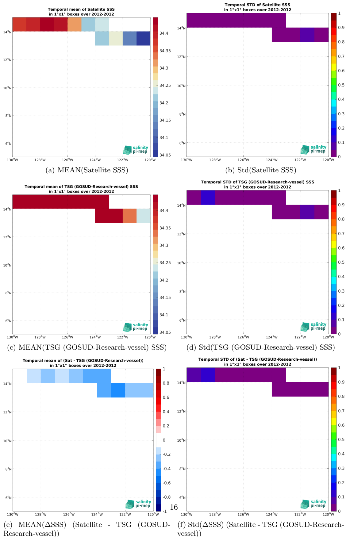
Figure 7: Temporal mean (left) and Std (right) of SSS from CCI SSS L4 Merged-OI v4.41 - 30-day running (ESA) (top), TSG (GOSUD-Research-vessel) (middle), and of \Delta SSS (Satellite - TSG (GOSUD-Research-vessel)). Only match-up pairs are used to generate these maps.
