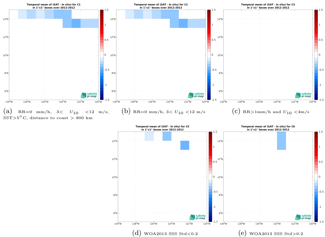
Figure 14: Temporal mean gridded over spatial boxes of size 1^\circ \times 1^\circ of \Delta SSS (CCI SSS L4 Merged-OI v4.41 - 30-day running (ESA) - TSG (GOSUD-Research-vessel)) for 5 different subdatasets corresponding to:RR=0 mm/h, 3 < U_{10} < 12 m/s, SST >5^\circ C, distance to coast > 800 km (a), RR=0 mm/h, 3 < U_{10} < 12 m/s (b), RR >1 mm/h and U_{10} < 4 m/s (c), WOA2013 SSS Std <0.2 (d), WOA2013 SSS Std >0.2 (e).
