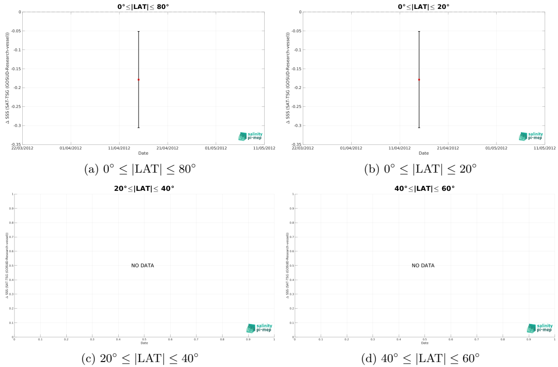
Figure 11: Monthly median (red curves) of \Delta SSS (Satellite - in situ TSG (GOSUD-Research-vessel)) and \pm 1 Std (black vertical thick bars) as function of time for all the collected Pi-MEP match-up pairs estimated over the SPURS 2 Pi-MEP region and for the full satellite product period are shown for different latitude bands: (a) 80^\circ\text{S}-80^\circ\text{N} , (b) 20^\circ\text{S}-20^\circ\text{N} , (c) 40^\circ\text{S}-20^\circ\text{S} and 20^\circ\text{N}-40^\circ\text{N} and (d) 60^\circ\text{S}-40^\circ\text{S} and 40^\circ\text{N}-60^\circ\text{N} .
