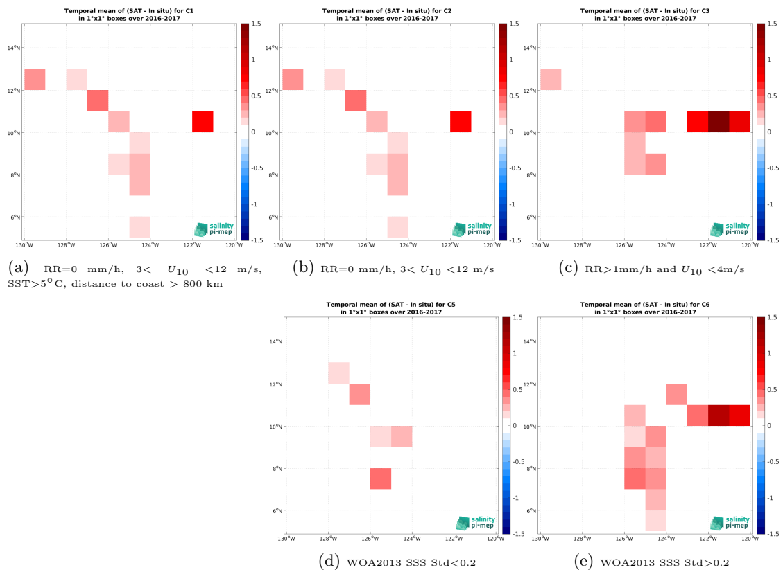
Figure 14: Temporal mean gridded over spatial boxes of size 1^\circ \times 1^\circ of \Delta SSS (CCI SSS L4 Merged-OI v4.41 - 30-day running (ESA) - Salinity Snake (SPURS 2)) for 5 different subdatasets corresponding to:RR=0 mm/h, 3 < U_{10} < 12 m/s, SST >5^\circ C, distance to coast > 800 km (a), RR=0 mm/h, 3 < U_{10} < 12 m/s (b), RR >1 mm/h and U_{10} < 4 m/s (c), WOA2013 SSS Std <0.2 (d), WOA2013 SSS Std >0.2 (e).
