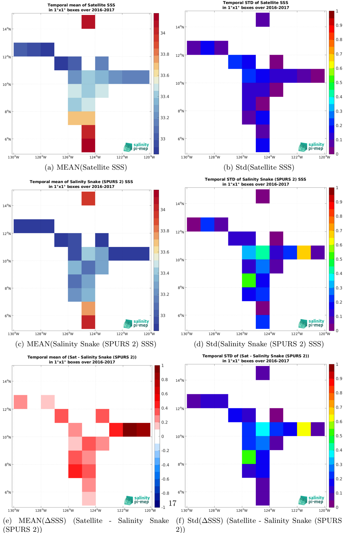
Figure 7: Temporal mean (left) and Std (right) of SSS from CCI SSS L4 Merged-OI v4.41 - 30-day running (ESA) (top), Salinity Snake (SPURS 2) (middle), and of \Delta SSS (Satellite - Salinity Snake (SPURS 2)). Only match-up pairs are used to generate these maps.
