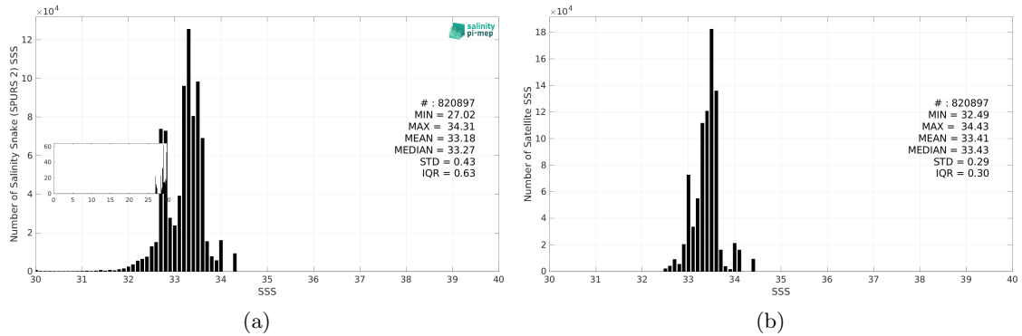
Figure 3: Histograms of SSS from Salinity Snake (SPURS 2) (a) and CCI SSS L4 Merged-OI v4.41 - 30-day running (ESA) (b) considering all match-up pairs per bins of 0.1 over the SPURS 2 Pi-MEP region and for the full satellite product period.
