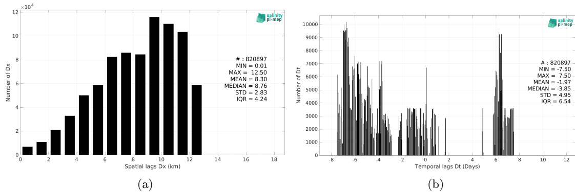
Figure 6: Histograms of the spatial (a) and temporal (b) lags between the location/time of the Salinity Snake (SPURS 2) measurement and the date of the corresponding CCI SSS L4 Merged-OI v4.41 - 30-day running (ESA) SSS pixel.
