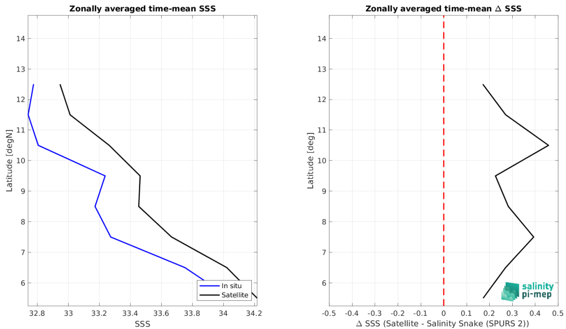
Figure 9: Left panel: Zonal mean SSS from CCI SSS L4 Merged-OI v4.41 - 30-day running (ESA) satellite product (black) and from Salinity Snake (SPURS 2) (blue). Right panel: Zonal mean of \Delta SSS (Satellite - Salinity Snake (SPURS 2)) for all the collected Pi-MEP match-up pairs estimated over the full satellite product period.
