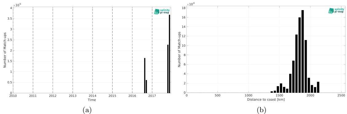
Figure 2: Number of match-ups between Salinity Snake (SPURS 2) and CCI SSS L4 Merged-OI v4.41 - 30-day running (ESA) SSS as a function of time (a) and as function of the distance to coast (b) over the SPURS 2 Pi-MEP region and for the full satellite product period.
