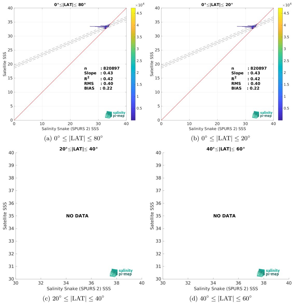
Figure 10: Contour maps of the concentration of CCI SSS L4 Merged-OI v4.41 - 30-day running (ESA) SSS (y-axis) versus Salinity Snake (SPURS 2) SSS (x-axis) at match-up pairs for different latitude bands. For each plot, the red line shows x=y . The black thin and dashed lines indicate a linear fit through the data cloud and the \pm 95\% confidence levels, respectively. The number match-up pairs n , the slope and R^2 coefficient of the linear fit, the root mean square (RMS) and the mean bias between satellite and in situ data are indicated for each latitude band in each plots.
