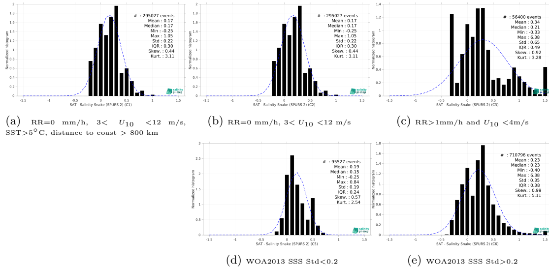
Figure 15: Normalized histogram of \Delta SSS (CCI SSS L4 Merged-OI v4.41 - 30-day running (ESA) - Salinity Snake (SPURS 2)) for 5 different subdatasets corresponding to: RR=0 mm/h, 3 < U_{10} < 12 m/s, SST > 5°C, distance to coast > 800 km (a), RR=0 mm/h, 3 < U_{10} < 12 m/s (b), RR > 1mm/h and U_{10} < 4 m/s (c), WOA2013 SSS Std < 0.2 (d), WOA2013 SSS Std > 0.2 (e).
