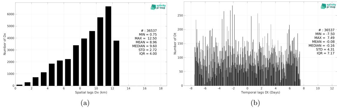
Figure 6: Histograms of the spatial (a) and temporal (b) lags between the location/time of the Seaglider (SPURS 2) measurement and the date of the corresponding CCI SSS L4 Merged-OI v4.41 - 30-day running (ESA) SSS pixel.
