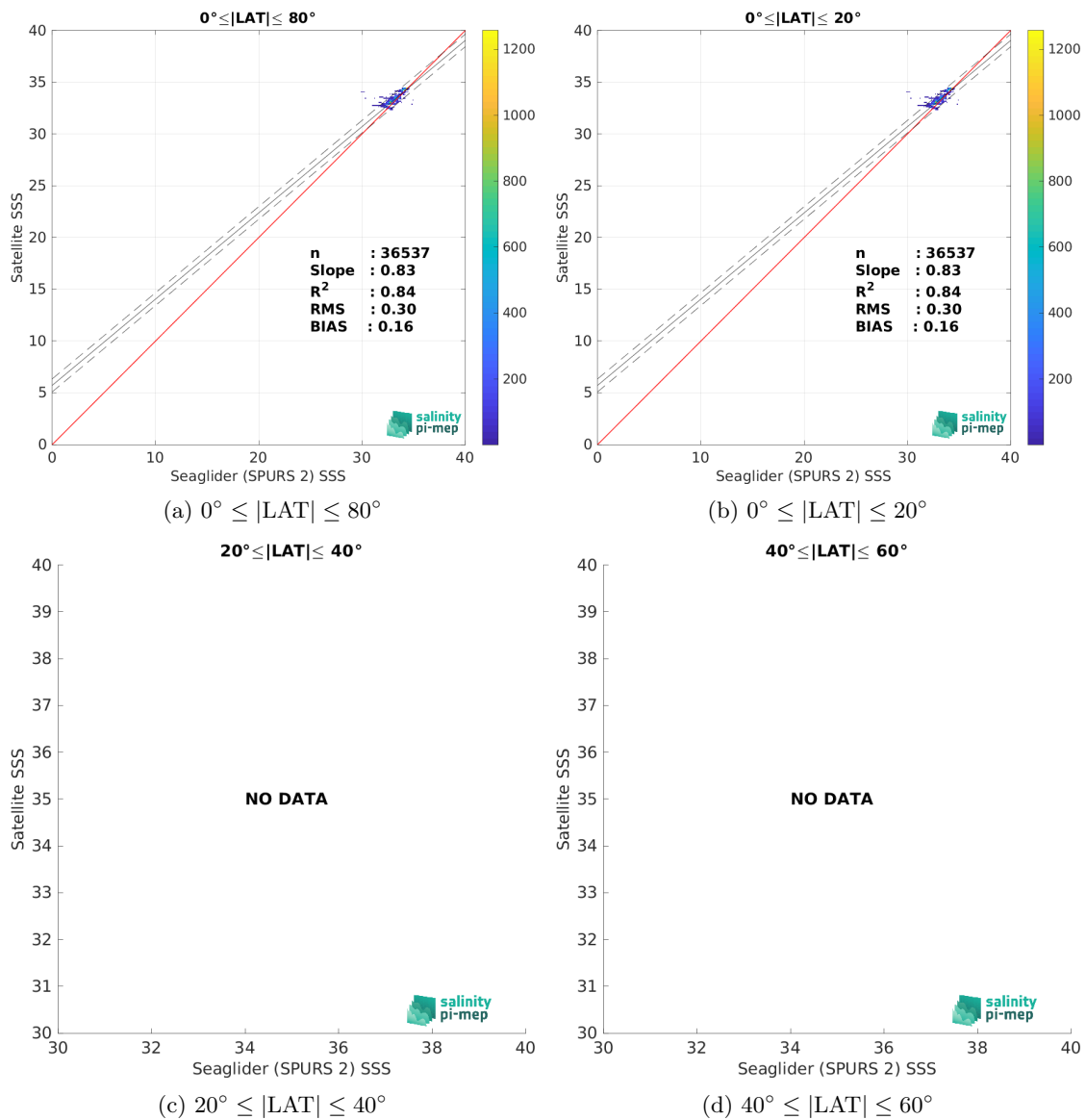
Figure 10: Contour maps of the concentration of CCI SSS L4 Merged-OI v4.41 - 30-day running (ESA) SSS (y-axis) versus Seaglider (SPURS 2) SSS (x-axis) at match-up pairs for different latitude bands. For each plot, the red line shows x=y . The black thin and dashed lines indicate a linear fit through the data cloud and the \pm 95\% confidence levels, respectively. The number match-up pairs n , the slope and R^2 coefficient of the linear fit, the root mean square (RMS) and the mean bias between satellite and in situ data are indicated for each latitude band in each plots.
