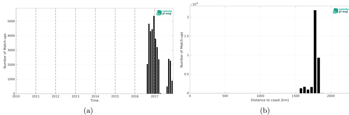
Figure 2: Number of match-ups between Seaglider (SPURS 2) and CCI SSS L4 Merged-OI v4.41 - 30-day running (ESA) SSS as a function of time (a) and as function of the distance to coast (b) over the SPURS 2 Pi-MEP region and for the full satellite product period.
