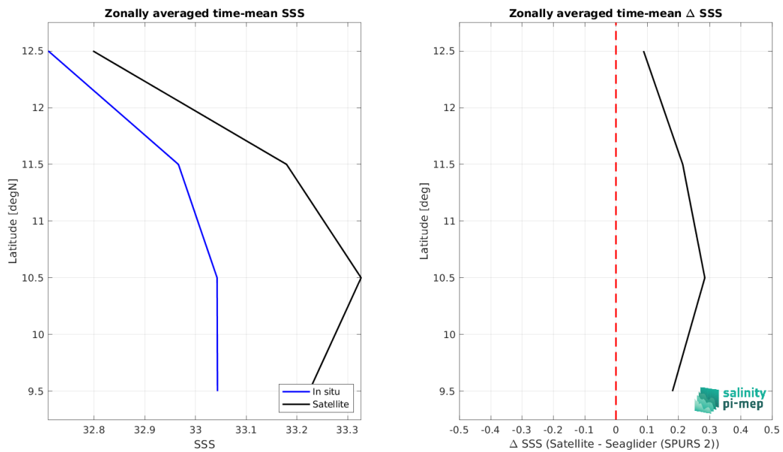
Figure 9: Left panel: Zonal mean SSS from CCI SSS L4 Merged-OI v4.41 - 30-day running (ESA) satellite product (black) and from Seaglider (SPURS 2) (blue). Right panel: Zonal mean of \Delta SSS (Satellite - Seaglider (SPURS 2)) for all the collected Pi-MEP match-up pairs estimated over the full satellite product period.
