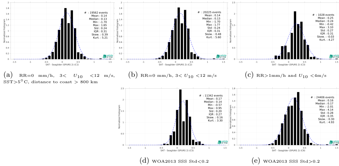
Figure 15: Normalized histogram of \Delta SSS (CCI SSS L4 Merged-OI v4.41 - 30-day running (ESA) - Seaglider (SPURS 2)) for 5 different subdatasets corresponding to: RR=0 mm/h, 3 < U_{10} < 12 m/s, SST > 5°C, distance to coast > 800 km (a), RR=0 mm/h, 3 < U_{10} < 12 m/s (b), RR > 1mm/h and U_{10} < 4 m/s (c), WOA2013 SSS Std < 0.2 (d), WOA2013 SSS Std > 0.2 (e).
