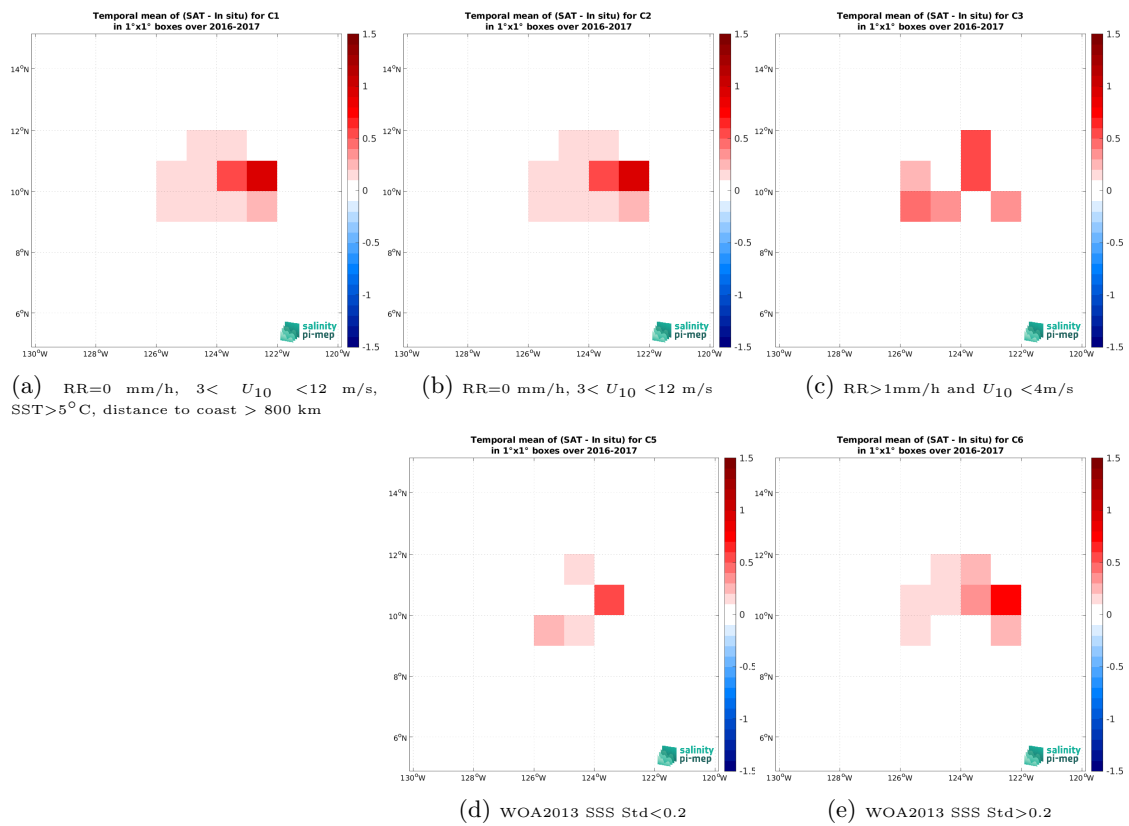
Figure 14: Temporal mean gridded over spatial boxes of size 1^\circ \times 1^\circ of \Delta\text{SSS} (CCI SSS L4 Merged-OI v4.41 - 30-day running (ESA) - Seaglider (SPURS 2)) for 5 different subdatasets corresponding to:RR=0 mm/h, 3 < U_{10} < 12 m/s, SST >5^\circ\text{C} , distance to coast > 800 km (a), RR=0 mm/h, 3 < U_{10} < 12 m/s (b), RR >1 mm/h and U_{10} < 4 m/s (c), WOA2013 SSS Std <0.2 (d), WOA2013 SSS Std >0.2 (e).
