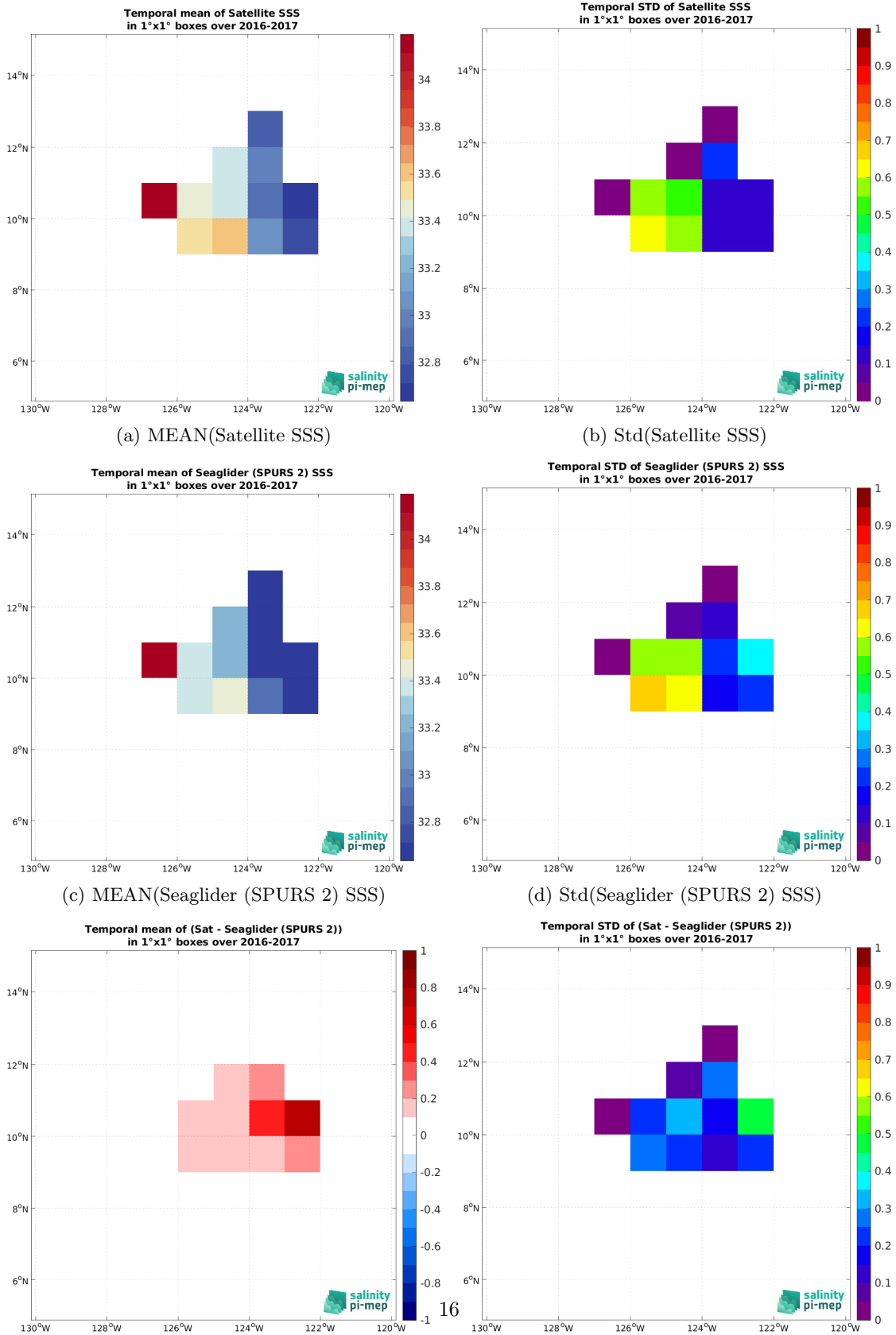
Figure 7: Temporal mean (left) and Std (right) of SSS from CCI SSS L4 Merged-OI v4.41 - 30-day running (ESA) (top), Seaglider (SPURS 2) (middle), and of \Delta SSS (Satellite - Seaglider (SPURS 2)). Only match-up pairs are used to generate these maps.
