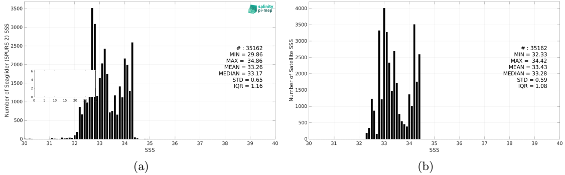
Figure 3: Histograms of SSS from Seaglider (SPURS 2) (a) and CCI SSS L4 Merged-OI v4.41 - 30-day running (ESA) (b) considering all match-up pairs per bins of 0.1 over the SPURS 2 Pi-MEP region and for the full satellite product period.
