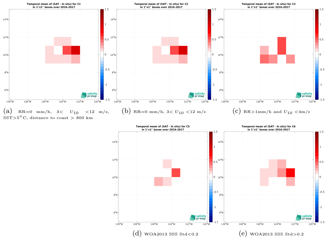
Figure 14: Temporal mean gridded over spatial boxes of size 1^\circ \times 1^\circ of \Delta SSS (CCI SSS L4 Merged-OI v4.41 - 30-day running (ESA) - Seaglider (SPURS 2)) for 5 different subdatasets corresponding to:RR=0 mm/h, 3 < U_{10} < 12 m/s, SST >5^\circ C, distance to coast > 800 km (a), RR=0 mm/h, 3 < U_{10} < 12 m/s (b), RR >1 mm/h and U_{10} < 4 m/s (c), WOA2013 SSS Std <0.2 (d), WOA2013 SSS Std >0.2 (e).
