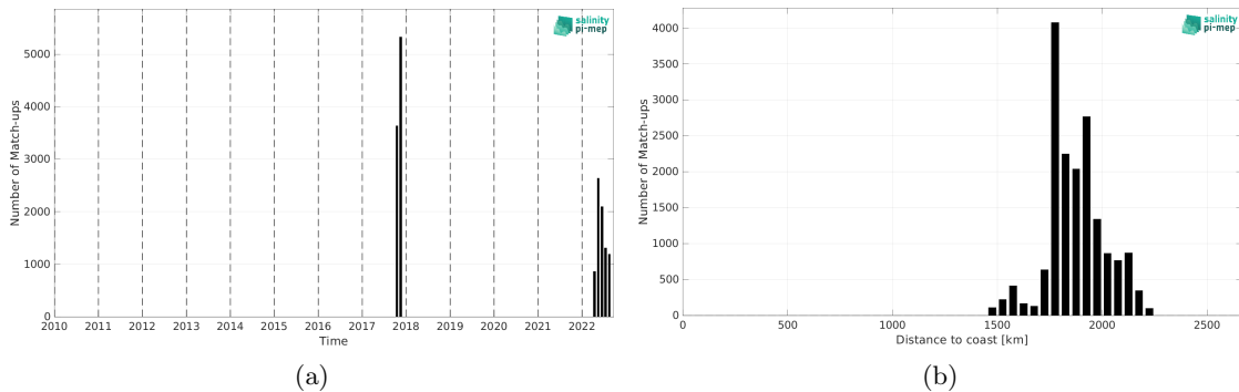
Figure 2: Number of match-ups between Saildrone and CCI SSS L4 Merged-OI v4.41 - 30-day running (ESA) SSS as a function of time (a) and as function of the distance to coast (b) over the SPURS 2 Pi-MEP region and for the full satellite product period.
