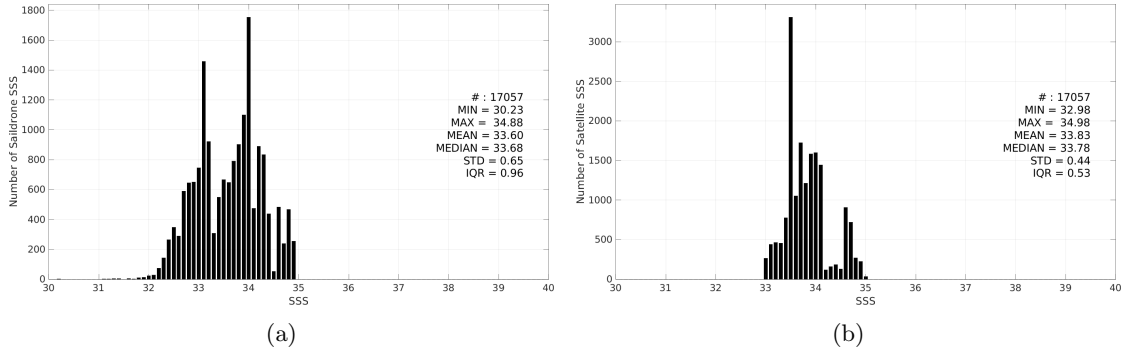
Figure 3: Histograms of SSS from Saildrone (a) and CCI SSS L4 Merged-OI v4.41 - 30-day running (ESA) (b) considering all match-up pairs per bins of 0.1 over the SPURS 2 Pi-MEP region and for the full satellite product period.
