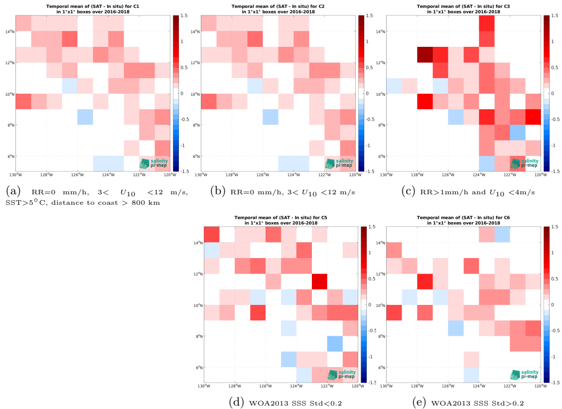
Figure 13: Temporal mean gridded over spatial boxes of size 1^\circ \times 1^\circ of \Delta\text{SSS} (CCI SSS L4 Merged-OI v4.41 - 30-day running (ESA) - Surface drifters) for 5 different subdatasets corresponding to:RR=0 mm/h, 3 < U_{10} < 12 m/s, SST >5^\circ\text{C} , distance to coast > 800 km (a), RR=0 mm/h, 3 < U_{10} < 12 m/s (b), RR >1 mm/h and U_{10} < 4 m/s (c), WOA2013 SSS Std <0.2 (d), WOA2013 SSS Std >0.2 (e).
