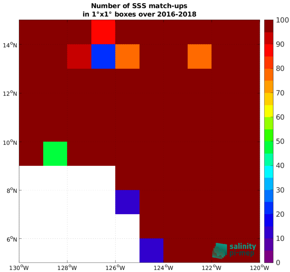
Figure 4: Number of SSS match-ups between Surface drifters SSS and the CCI SSS L4 Merged-OI v4.41 - 30-day running (ESA) SSS product for the SPURS 2 Pi-MEP region over 1^\circ \times 1^\circ boxes and for the full satellite product period.
