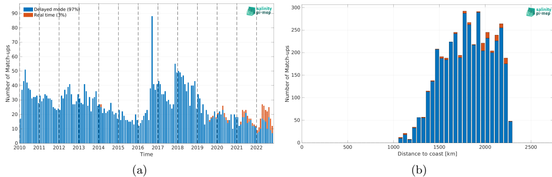
Figure 2: Number of match-ups between Argo and CCI SSS L4 Merged-OI v4.41 - 30-day running (ESA) SSS as a function of time (a) and as function of the distance to coast (b) over the SPURS 2 Pi-MEP region and for the full satellite product period.
