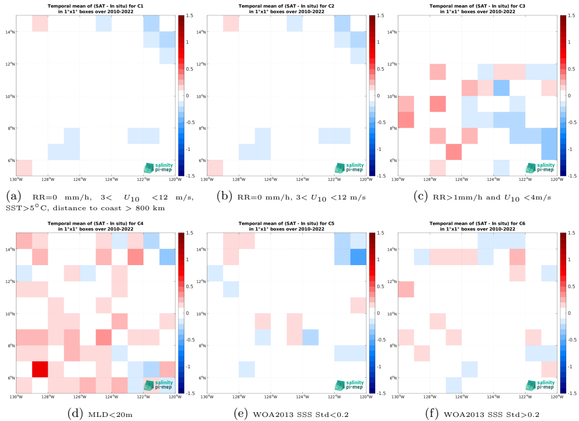
Figure 14: Temporal mean gridded over spatial boxes of size 1^\circ \times 1^\circ of \Delta\text{SSS} (CCI SSS L4 Merged-OI v4.41 - 30-day running (ESA) - Argo) for 6 different subdatasets corresponding to:RR=0 mm/h, 3 < U_{10} < 12 m/s, SST>5°C, distance to coast > 800 km (a), RR=0 mm/h, 3 < U_{10} < 12 m/s (b), RR>1mm/h and U_{10} < 4 m/s (c),MLD<20m (d),WOA2013 SSS Std<0.2 (e),WOA2013 SSS Std>0.2 (f).
