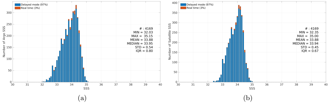
Figure 3: Histograms of SSS from Argo (a) and CCI SSS L4 Merged-OI v4.41 - 30-day running (ESA) (b) considering all match-up pairs per bins of 0.1 over the SPURS 2 Pi-MEP region and for the full satellite product period.
