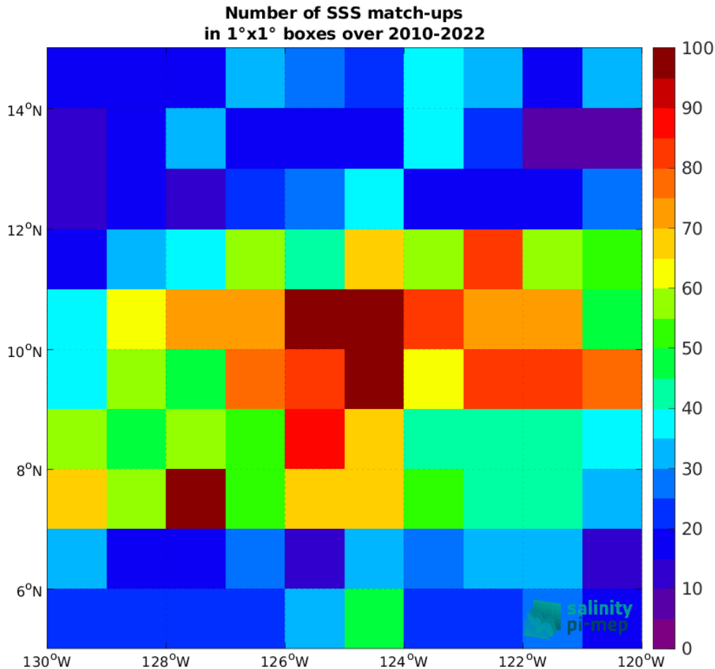
Figure 5: Number of SSS match-ups between Argo SSS and the CCI SSS L4 Merged-OI v4.41 - 30-day running (ESA) SSS product for the SPURS 2 Pi-MEP region over 1^\circ \times 1^\circ boxes and for the full satellite product period.
