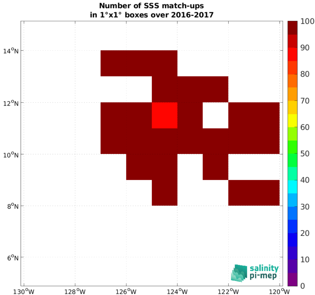
Figure 4: Number of SSS match-ups between Waveglider (SPURS 2) SSS and the CCI SSS L4 Merged-OI v4.4 - 7-day running (ESA) SSS product for the SPURS 2 Pi-MEP region over 1^\circ \times 1^\circ boxes and for the full satellite product period.
