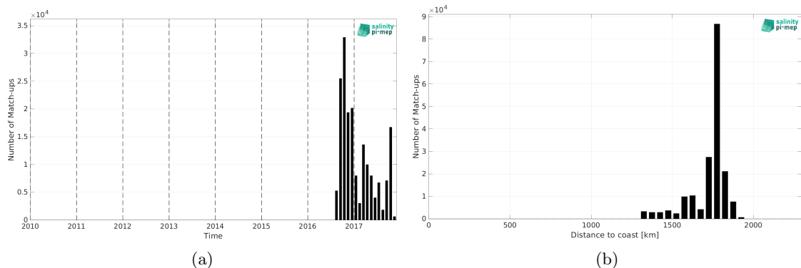
Figure 1: Number of match-ups between Waveglider (SPURS 2) and CCI SSS L4 Merged-OI v4.4 - 7-day running (ESA) SSS as a function of time (a) and as function of the distance to coast (b) over the SPURS 2 Pi-MEP region and for the full satellite product period.
