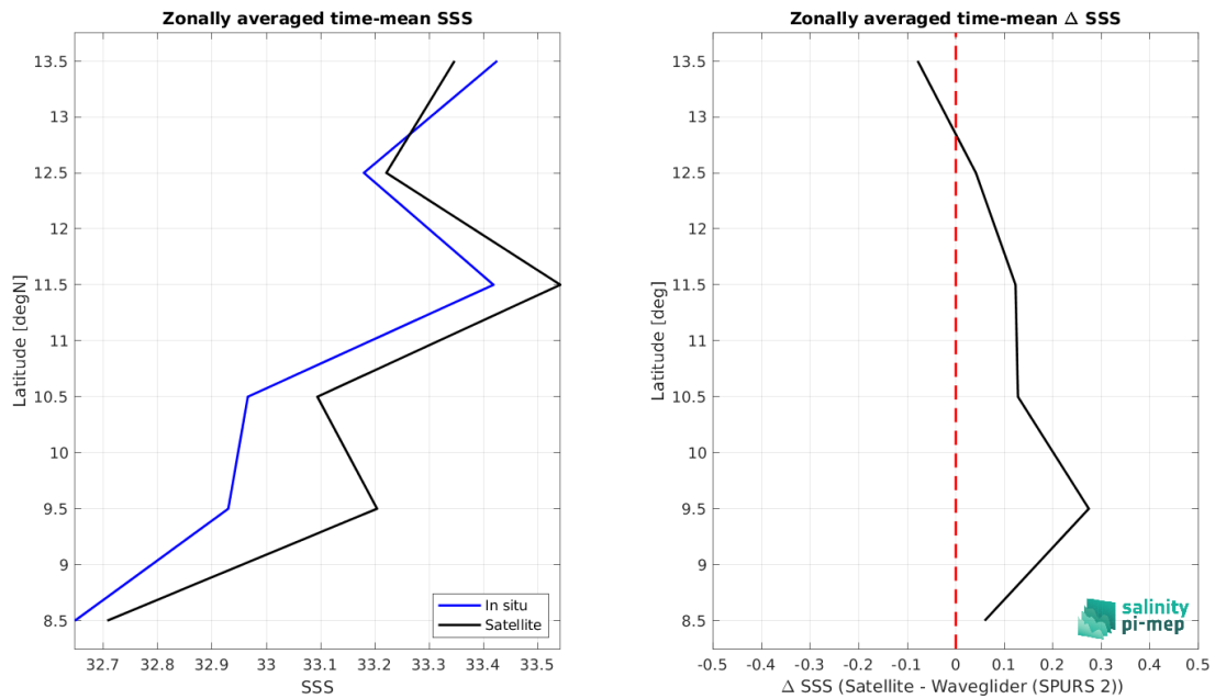
Figure 8: Left panel: Zonal mean SSS from CCI SSS L4 Merged-OI v4.4 - 7-day running (ESA) satellite product (black) and from Waveglider (SPURS 2) (blue). Right panel: Zonal mean of \Delta SSS (Satellite - Waveglider (SPURS 2)) for all the collected Pi-MEP match-up pairs estimated over the full satellite product period.
