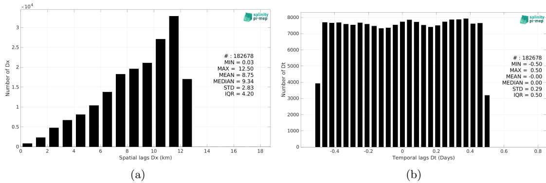
Figure 5: Histograms of the spatial (a) and temporal (b) lags between the location/time of the Waveglider (SPURS 2) measurement and the date of the corresponding CCI SSS L4 Merged-OI v4.4 - 7-day running (ESA) SSS pixel.
