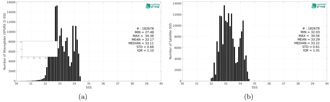
Figure 2: Histograms of SSS from Waveglider (SPURS 2) (a) and CCI SSS L4 Merged-OI v4.4 - 7-day running (ESA) (b) considering all match-up pairs per bins of 0.1 over the SPURS 2 Pi-MEP region and for the full satellite product period.
