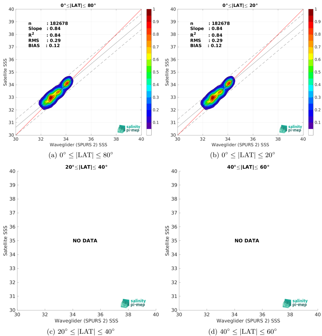
Figure 9: Contour maps of the concentration of CCI SSS L4 Merged-OI v4.4 - 7-day running (ESA) SSS (y-axis) versus Waveglider (SPURS 2) SSS (x-axis) at match-up pairs for different latitude bands. For each plot, the red line shows x=y . The black thin and dashed lines indicate a linear fit through the data cloud and the \pm 95\% confidence levels, respectively. The number match-up pairs n , the slope and R^2 coefficient of the linear fit, the root mean square (RMS) and the mean bias between satellite and in situ data are indicated for each latitude band in each plots.
