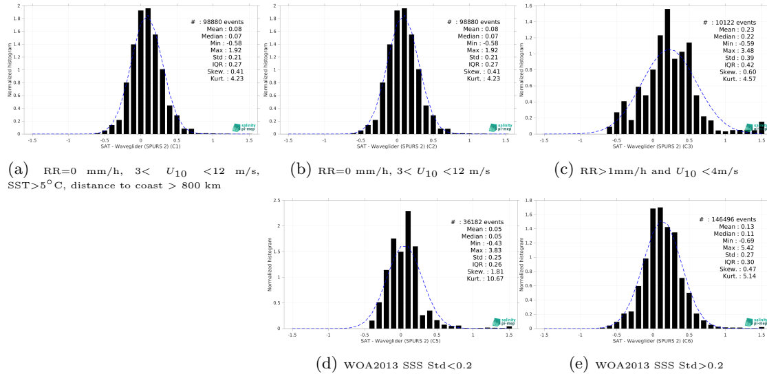
Figure 13: Normalized histogram of \Delta SSS (CCI SSS L4 Merged-OI v4.4 - 7-day running (ESA) - Waveglider (SPURS 2)) for 5 different subdatasets corresponding to: RR=0 mm/h, 3 < U_{10} < 12 m/s, SST>5°C, distance to coast > 800 km (a), RR=0 mm/h, 3 < U_{10} < 12 m/s (b), RR>1mm/h and U_{10} < 4 m/s (c), WOA2013 SSS Std<0.2 (d), WOA2013 SSS Std>0.2 (e).
