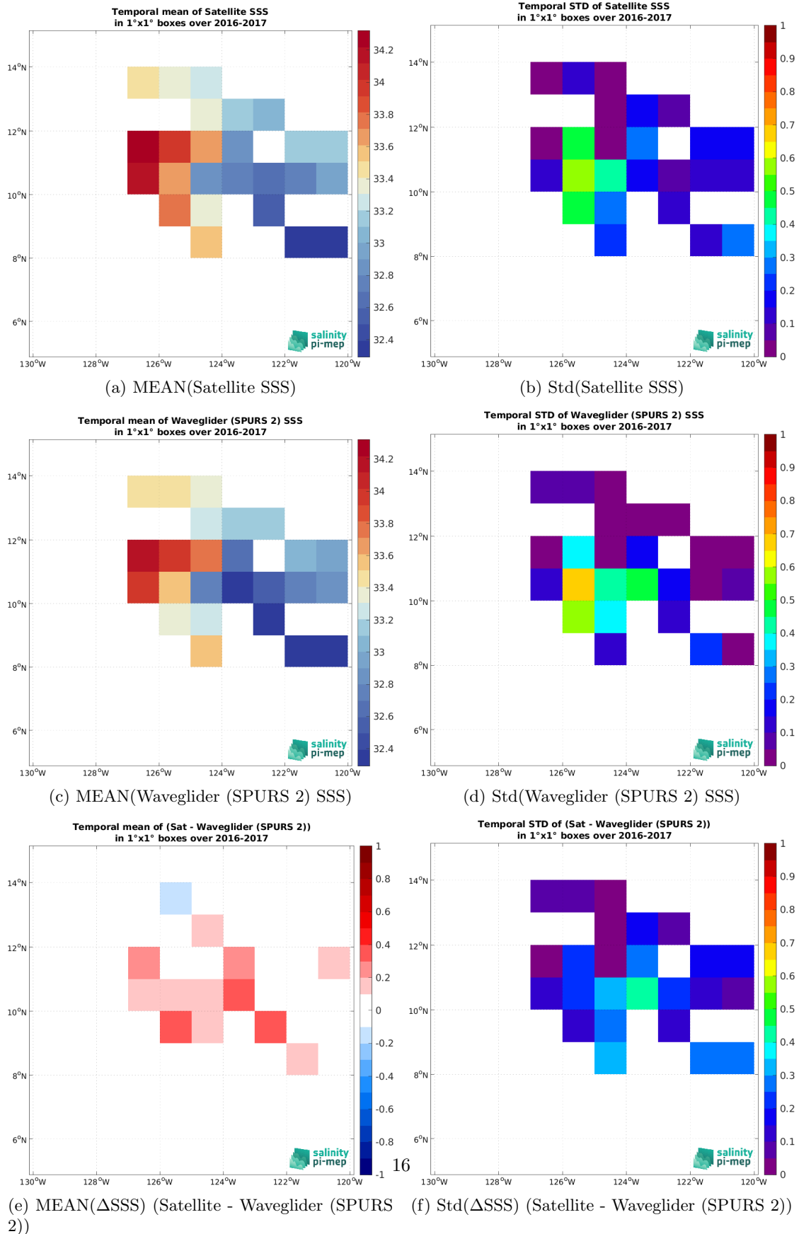
Figure 6: Temporal mean (left) and Std (right) of SSS from CCI SSS L4 Merged-OI v4.4 - 7-day running (ESA) (top), Waveglider (SPURS 2) (middle), and of \Delta SSS (Satellite - Waveglider (SPURS 2)). Only match-up pairs are used to generate these maps.
