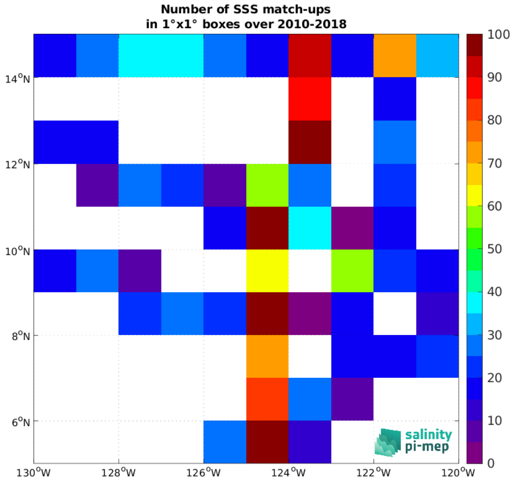
Figure 4: Number of SSS match-ups between TSG (SAMOS) SSS and the CCI SSS L4 Merged-OI v4.4 - 7-day running (ESA) SSS product for the SPURS 2 Pi-MEP region over 1^\circ \times 1^\circ boxes and for the full satellite product period.
