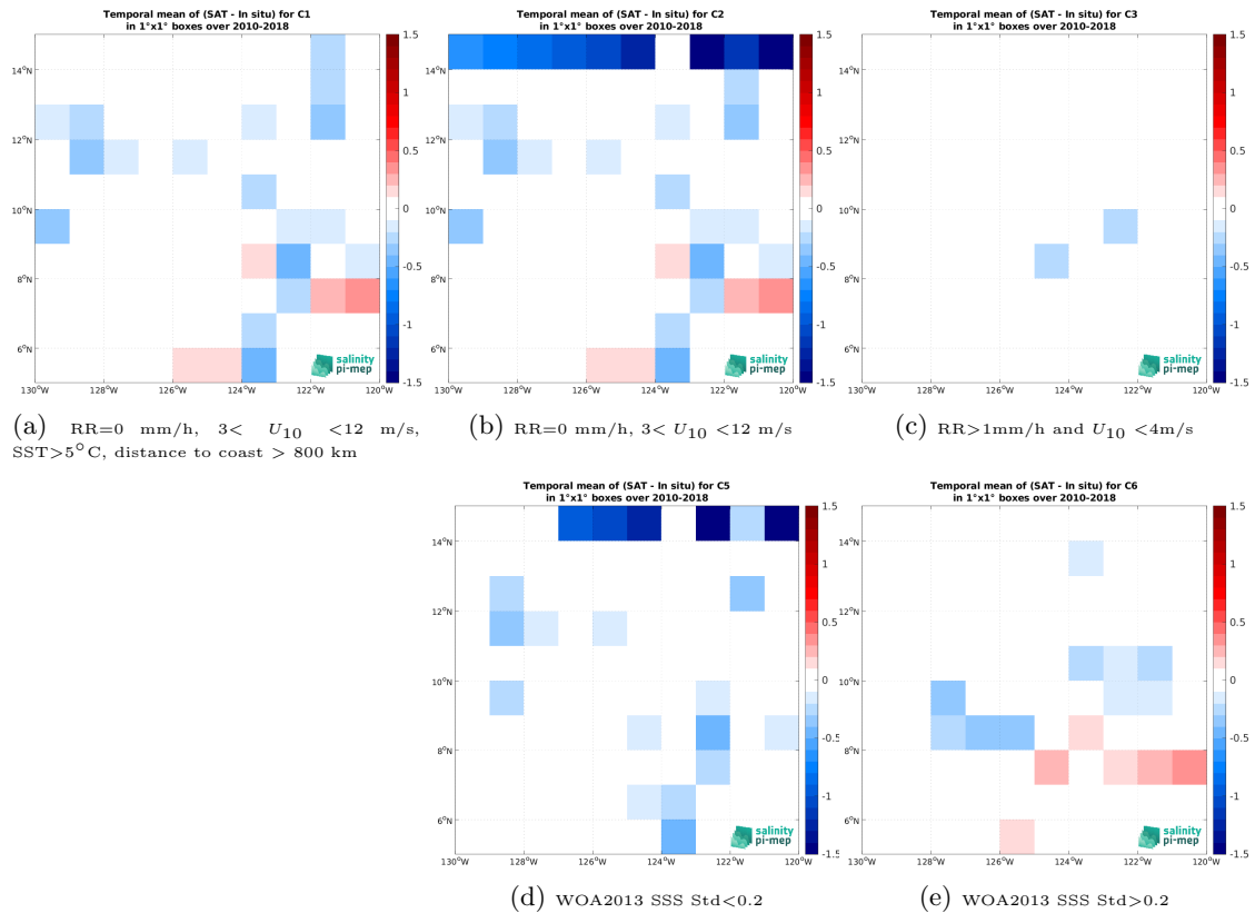
Figure 12: Temporal mean gridded over spatial boxes of size 1^\circ \times 1^\circ of \Delta\text{SSS} (CCI SSS L4 Merged-OI v4.4 - 7-day running (ESA) - TSG (SAMOS)) for 5 different subdatasets corresponding to:RR=0 mm/h, 3 < U_{10} < 12 m/s, SST >5^\circ\text{C} , distance to coast > 800 km (a), RR=0 mm/h, 3 < U_{10} < 12 m/s (b), RR >1 mm/h and U_{10} < 4 m/s (c), WOA2013 SSS Std <0.2 (d), WOA2013 SSS Std >0.2 (e).
