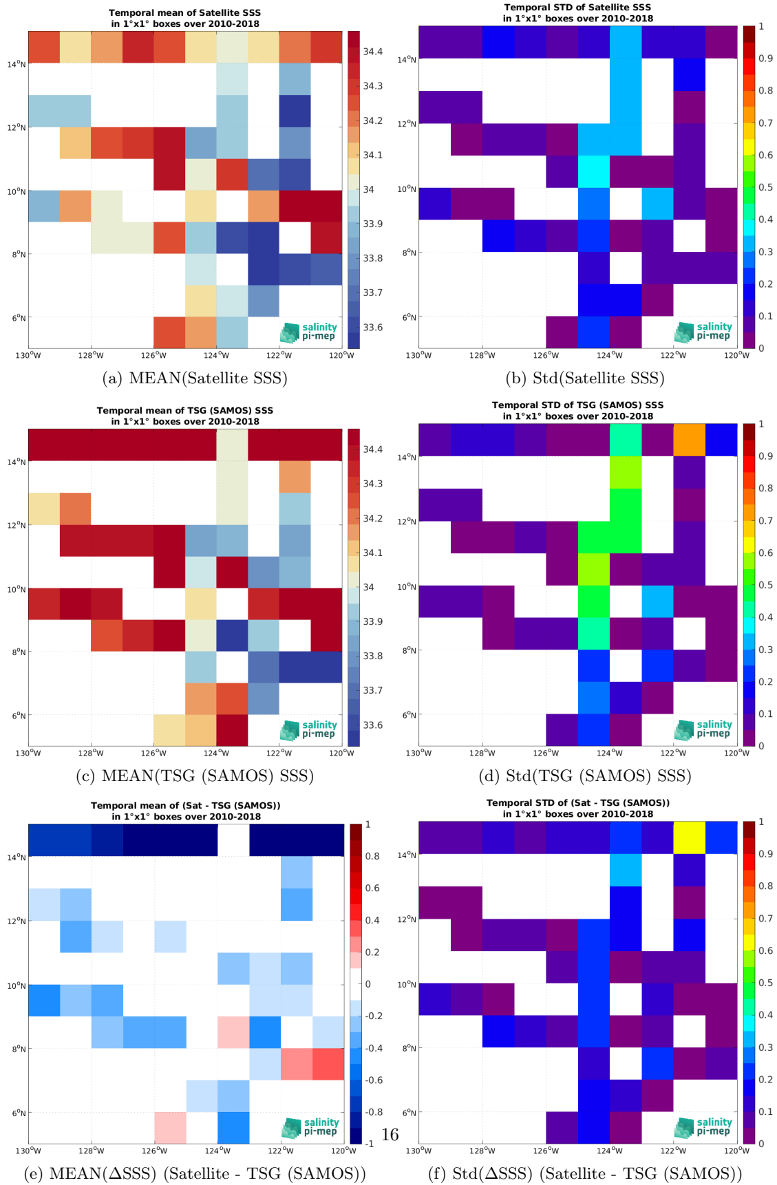
Figure 6: Temporal mean (left) and Std (right) of SSS from CCI SSS L4 Merged-OI v4.4 - 7-day running (ESA) (top), TSG (SAMOS) (middle), and of \Delta SSS (Satellite - TSG (SAMOS)). Only match-up pairs are used to generate these maps.
