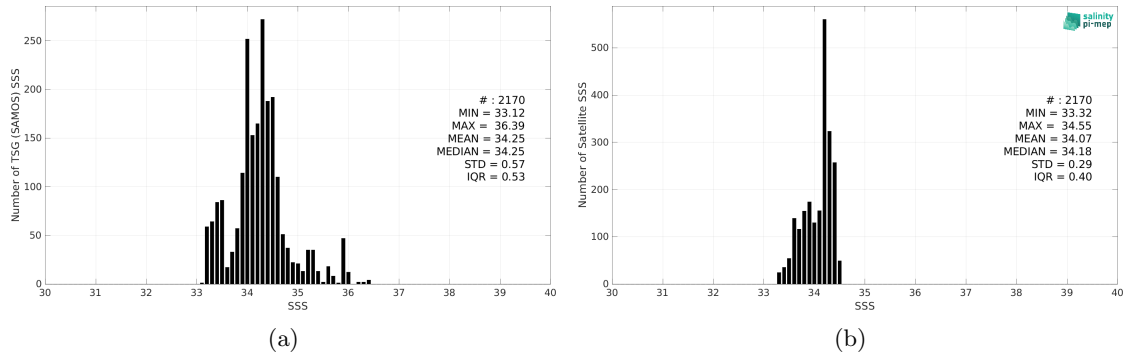
Figure 2: Histograms of SSS from TSG (SAMOS) (a) and CCI SSS L4 Merged-OI v4.4 - 7-day running (ESA) (b) considering all match-up pairs per bins of 0.1 over the SPURS 2 Pi-MEP region and for the full satellite product period.
