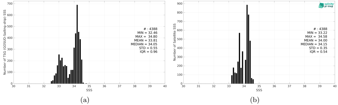
Figure 2: Histograms of SSS from TSG (GOSUD-Sailing-ship) (a) and CCI SSS L4 Merged-OI v4.4 - 7-day running (ESA) (b) considering all match-up pairs per bins of 0.1 over the SPURS 2 Pi-MEP region and for the full satellite product period.
