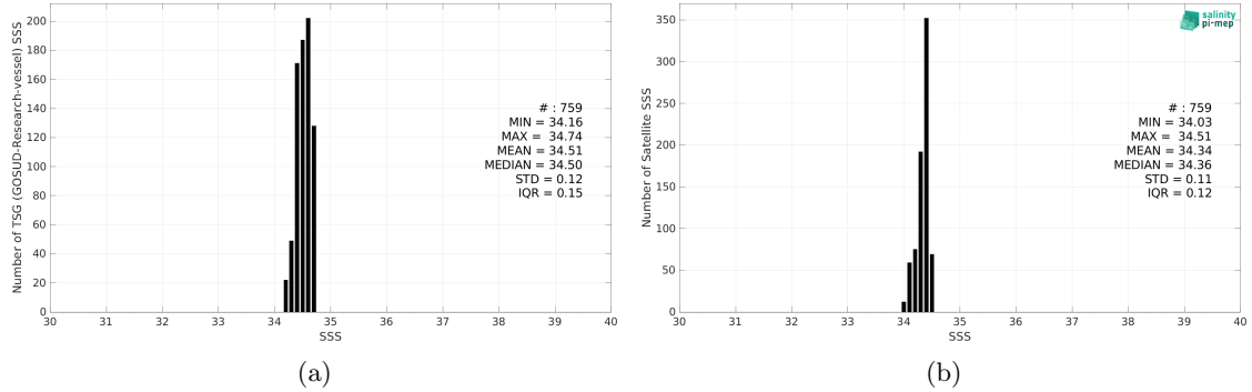
Figure 2: Histograms of SSS from TSG (GOSUD-Research-vessel) (a) and CCI SSS L4 Merged-OI v4.4 - 7-day running (ESA) (b) considering all match-up pairs per bins of 0.1 over the SPURS 2 Pi-MEP region and for the full satellite product period.
