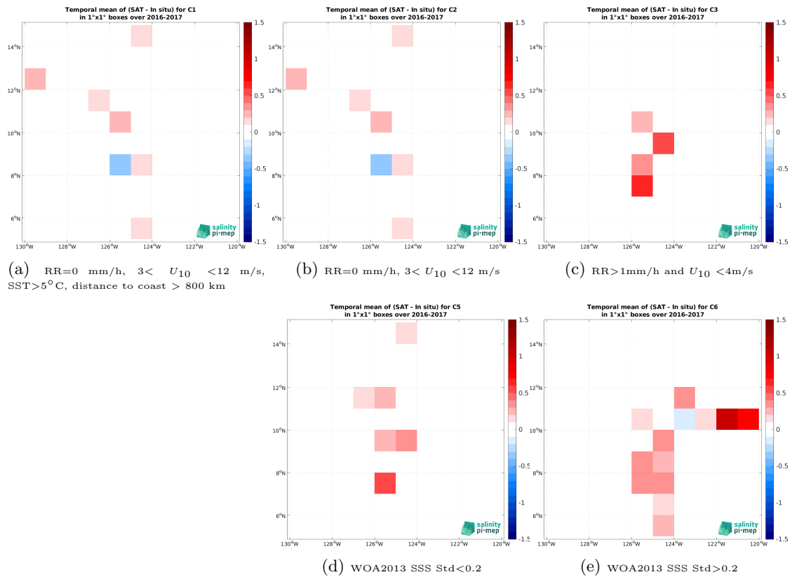
Figure 12: Temporal mean gridded over spatial boxes of size 1^\circ \times 1^\circ of \Delta SSS (CCI SSS L4 Merged-OI v4.4 - 7-day running (ESA) - Salinity Snake (SPURS 2)) for 5 different subdatasets corresponding to: RR=0 mm/h, 3 < U_{10} < 12 m/s, SST > 5°C, distance to coast > 800 km (a), RR=0 mm/h, 3 < U_{10} < 12 m/s (b), RR > 1mm/h and U_{10} < 4 m/s (c), WOA2013 SSS Std < 0.2 (d), WOA2013 SSS Std > 0.2 (e).
