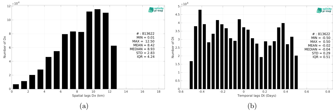
Figure 5: Histograms of the spatial (a) and temporal (b) lags between the location/time of the Salinity Snake (SPURS 2) measurement and the date of the corresponding CCI SSS L4 Merged-OI v4.4 - 7-day running (ESA) SSS pixel.
