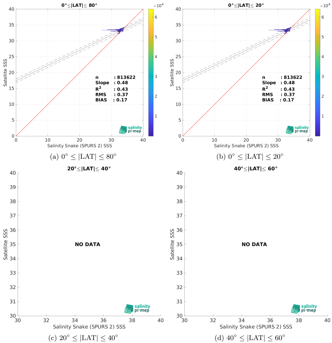
Figure 9: Contour maps of the concentration of CCI SSS L4 Merged-OI v4.4 - 7-day running (ESA) SSS (y-axis) versus Salinity Snake (SPURS 2) SSS (x-axis) at match-up pairs for different latitude bands. For each plot, the red line shows x=y . The black thin and dashed lines indicate a linear fit through the data cloud and the \pm 95\% confidence levels, respectively. The number match-up pairs n , the slope and R^2 coefficient of the linear fit, the root mean square (RMS) and the mean bias between satellite and in situ data are indicated for each latitude band in each plots.
