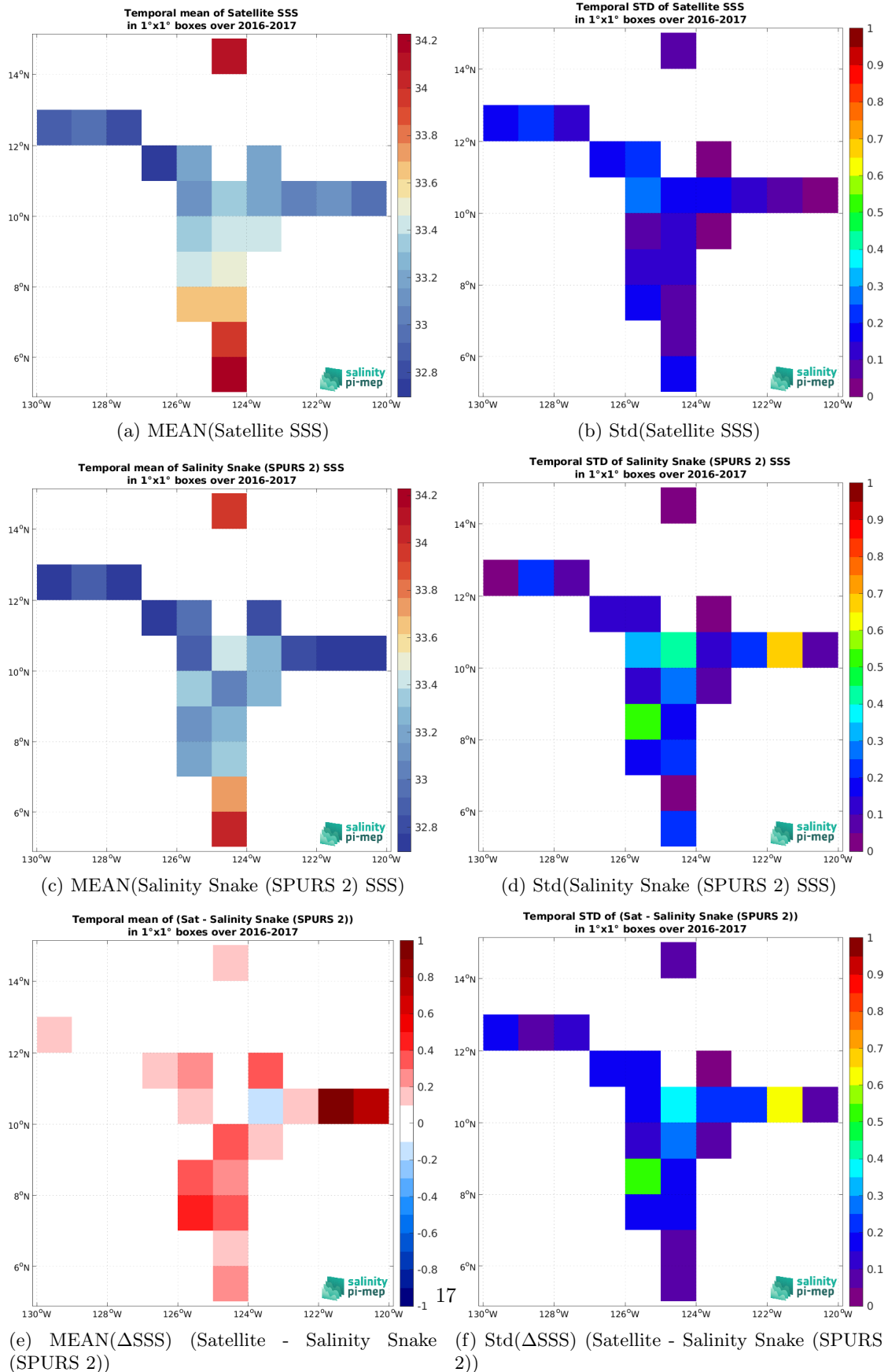
Figure 6: Temporal mean (left) and Std (right) of SSS from CCI SSS L4 Merged-OI v4.4 - 7-day running (ESA) (top), Salinity Snake (SPURS 2) (middle), and of \Delta SSS (Satellite - Salinity Snake (SPURS 2)). Only match-up pairs are used to generate these maps.
