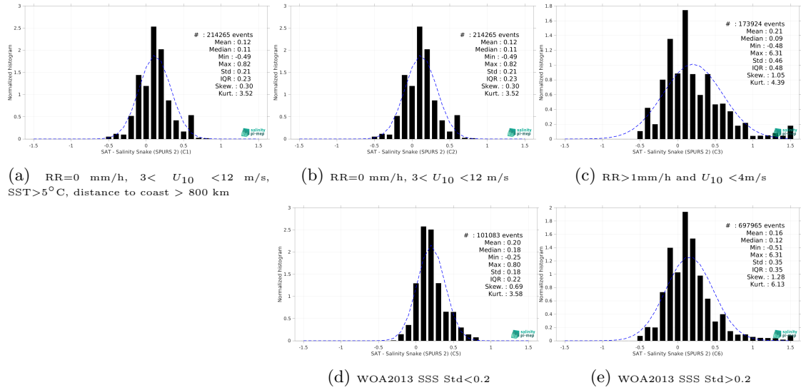
Figure 13: Normalized histogram of \Delta\text{SSS} (CCI SSS L4 Merged-OI v4.4 - 7-day running (ESA) - Salinity Snake (SPURS 2)) for 5 different subdatasets corresponding to: RR=0 mm/h, 3 < U_{10} < 12 m/s, SST>5°C, distance to coast > 800 km (a), RR=0 mm/h, 3 < U_{10} < 12 m/s (b), RR>1mm/h and U_{10} < 4 m/s (c), WOA2013 SSS Std<0.2 (d), WOA2013 SSS Std>0.2 (e).
