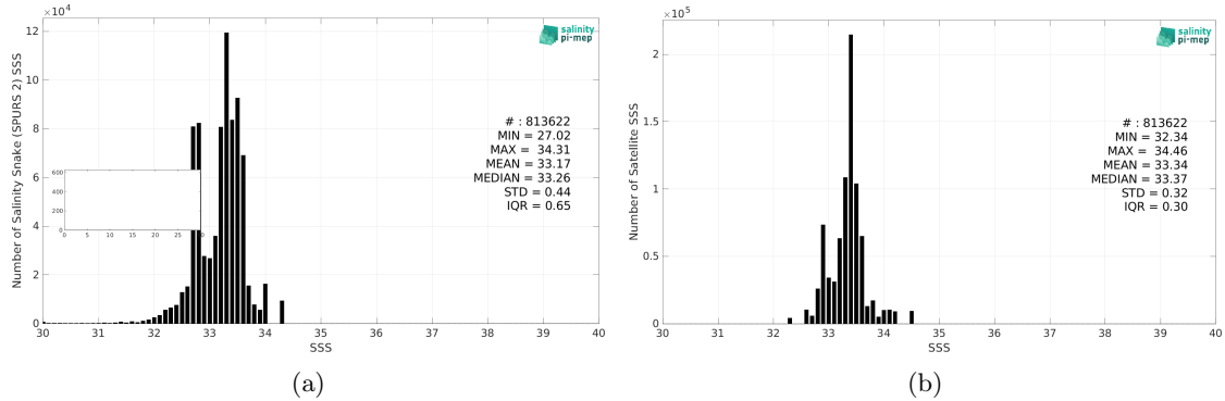
Figure 2: Histograms of SSS from Salinity Snake (SPURS 2) (a) and CCI SSS L4 Merged-OI v4.4 - 7-day running (ESA) (b) considering all match-up pairs per bins of 0.1 over the SPURS 2 Pi-MEP region and for the full satellite product period.
