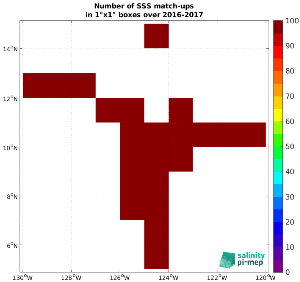
Figure 4: Number of SSS match-ups between Salinity Snake (SPURS 2) SSS and the CCI SSS L4 Merged-OI v4.4 - 7-day running (ESA) SSS product for the SPURS 2 Pi-MEP region over 1^\circ \times 1^\circ boxes and for the full satellite product period.
