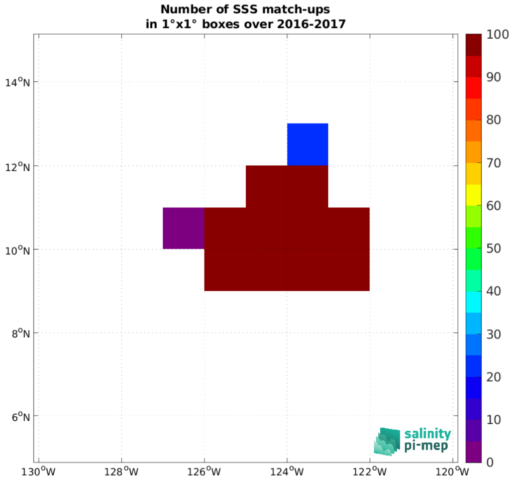
Figure 4: Number of SSS match-ups between Seaglider (SPURS 2) SSS and the CCI SSS L4 Merged-OI v4.4 - 7-day running (ESA) SSS product for the SPURS 2 Pi-MEP region over 1^\circ \times 1^\circ boxes and for the full satellite product period.
