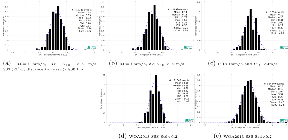
Figure 13: Normalized histogram of \Delta SSS (CCI SSS L4 Merged-OI v4.4 - 7-day running (ESA) - Seaglider (SPURS 2)) for 5 different subdatasets corresponding to: RR=0 mm/h, 3 < U_{10} < 12 m/s, SST > 5°C, distance to coast > 800 km (a), RR=0 mm/h, 3 < U_{10} < 12 m/s (b), RR > 1mm/h and U_{10} < 4 m/s (c), WOA2013 SSS Std < 0.2 (d), WOA2013 SSS Std > 0.2 (e).
