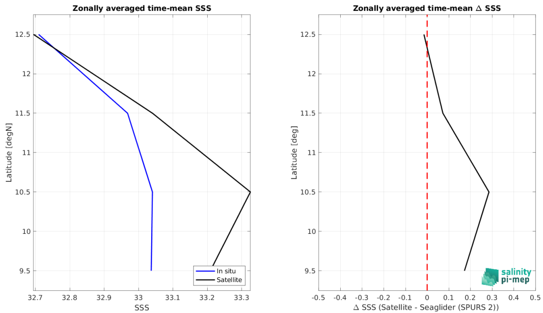
Figure 8: Left panel: Zonal mean SSS from CCI SSS L4 Merged-OI v4.4 - 7-day running (ESA) satellite product (black) and from Seaglider (SPURS 2) (blue). Right panel: Zonal mean of \Delta SSS (Satellite - Seaglider (SPURS 2)) for all the collected Pi-MEP match-up pairs estimated over the full satellite product period.
