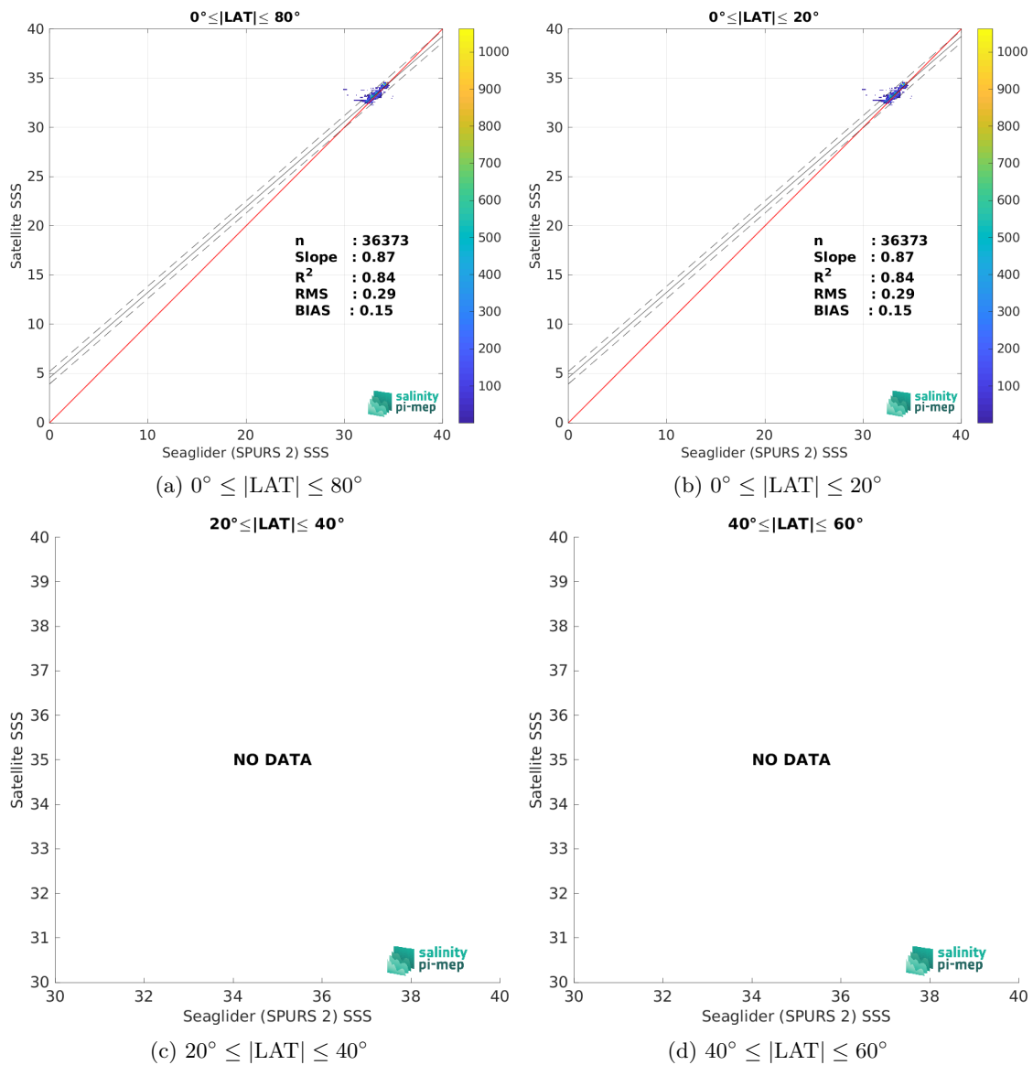
Figure 9: Contour maps of the concentration of CCI SSS L4 Merged-OI v4.4 - 7-day running (ESA) SSS (y-axis) versus Seaglider (SPURS 2) SSS (x-axis) at match-up pairs for different latitude bands. For each plot, the red line shows x=y . The black thin and dashed lines indicate a linear fit through the data cloud and the \pm 95\% confidence levels, respectively. The number match-up pairs n , the slope and R^2 coefficient of the linear fit, the root mean square (RMS) and the mean bias between satellite and in situ data are indicated for each latitude band in each plots.
