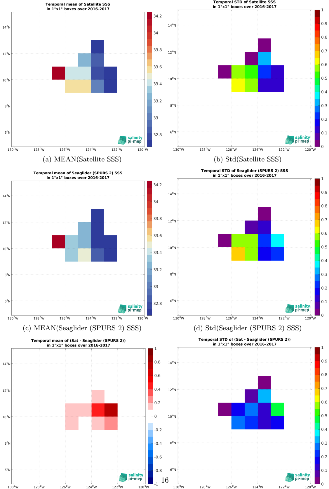
Figure 6: Temporal mean (left) and Std (right) of SSS from CCI SSS L4 Merged-OI v4.4 - 7-day running (ESA) (top), Seaglider (SPURS 2) (middle), and of \Delta SSS (Satellite - Seaglider (SPURS 2)). Only match-up pairs are used to generate these maps.
