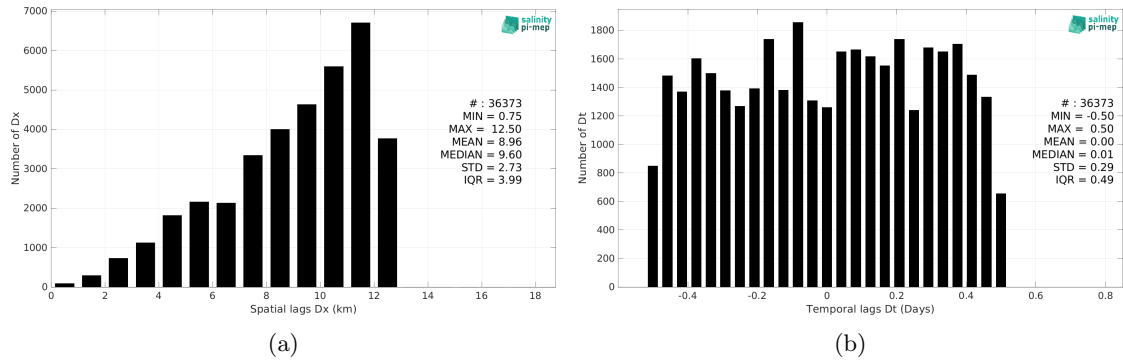
Figure 5: Histograms of the spatial (a) and temporal (b) lags between the location/time of the Seaglider (SPURS 2) measurement and the date of the corresponding CCI SSS L4 Merged-OI v4.4 - 7-day running (ESA) SSS pixel.
