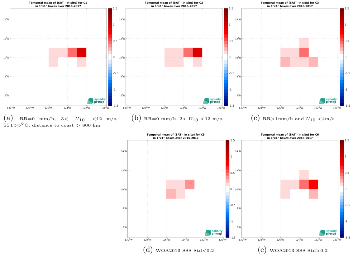
Figure 12: Temporal mean gridded over spatial boxes of size 1^{\circ}\times 1^{\circ} of \Delta\text{SSS} (CCI SSS L4 Merged-OI v4.4 - 7-day running (ESA) - Seaglider (SPURS 2)) for 5 different subdatasets corresponding to:RR=0 mm/h, 3 < U_{10} < 12 m/s, SST >5^{\circ}\text{C} , distance to coast > 800 km (a), RR=0 mm/h, 3 < U_{10} < 12 m/s (b), RR >1 mm/h and U_{10} < 4 m/s (c), WOA2013 SSS Std <0.2 (d), WOA2013 SSS Std >0.2 (e).
