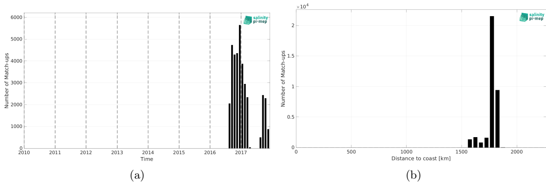
Figure 1: Number of match-ups between Seaglider (SPURS 2) and CCI SSS L4 Merged-OI v4.4 - 7-day running (ESA) SSS as a function of time (a) and as function of the distance to coast (b) over the SPURS 2 Pi-MEP region and for the full satellite product period.
