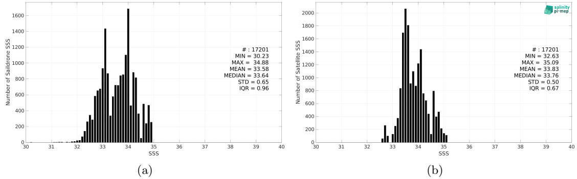
Figure 2: Histograms of SSS from Saildrone (a) and CCI SSS L4 Merged-OI v4.4 - 7-day running (ESA) (b) considering all match-up pairs per bins of 0.1 over the SPURS 2 Pi-MEP region and for the full satellite product period.
