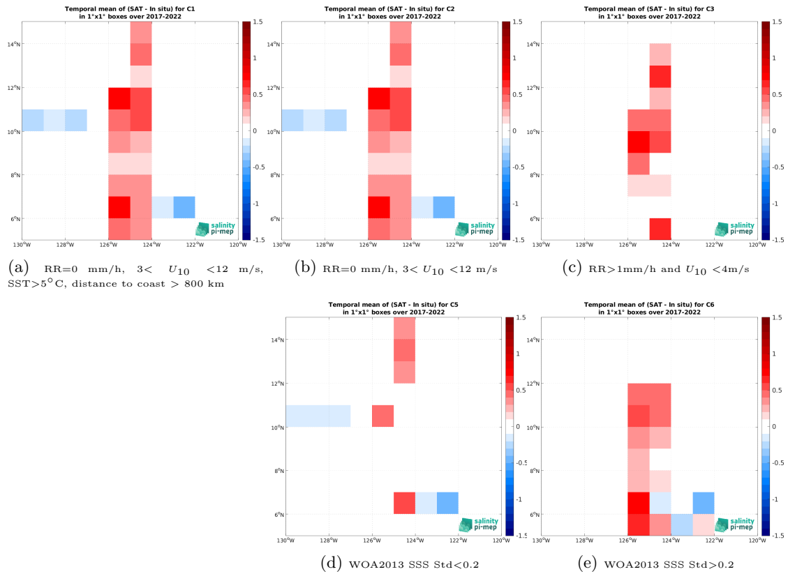
Figure 12: Temporal mean gridded over spatial boxes of size 1^\circ \times 1^\circ of \Delta SSS (CCI SSS L4 Merged-OI v4.4 - 7-day running (ESA) - Sairdrone) for 5 different subdatasets corresponding to:RR=0 mm/h, 3 < U_{10} < 12 m/s, SST >5^\circ\text{C} , distance to coast > 800 km (a), RR=0 mm/h, 3 < U_{10} < 12 m/s (b), RR >1 mm/h and U_{10} < 4 m/s (c), WOA2013 SSS Std <0.2 (d), WOA2013 SSS Std >0.2 (e).
