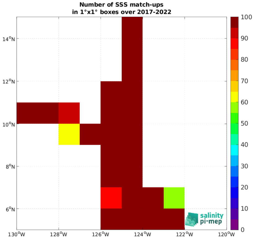
Figure 4: Number of SSS match-ups between Saildrone SSS and the CCI SSS L4 Merged-OI v4.4 - 7-day running (ESA) SSS product for the SPURS 2 Pi-MEP region over 1^\circ \times 1^\circ boxes and for the full satellite product period.
