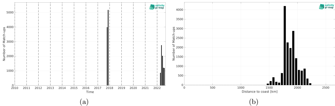
Figure 1: Number of match-ups between Saildrone and CCI SSS L4 Merged-OI v4.4 - 7-day running (ESA) SSS as a function of time (a) and as function of the distance to coast (b) over the SPURS 2 Pi-MEP region and for the full satellite product period.
