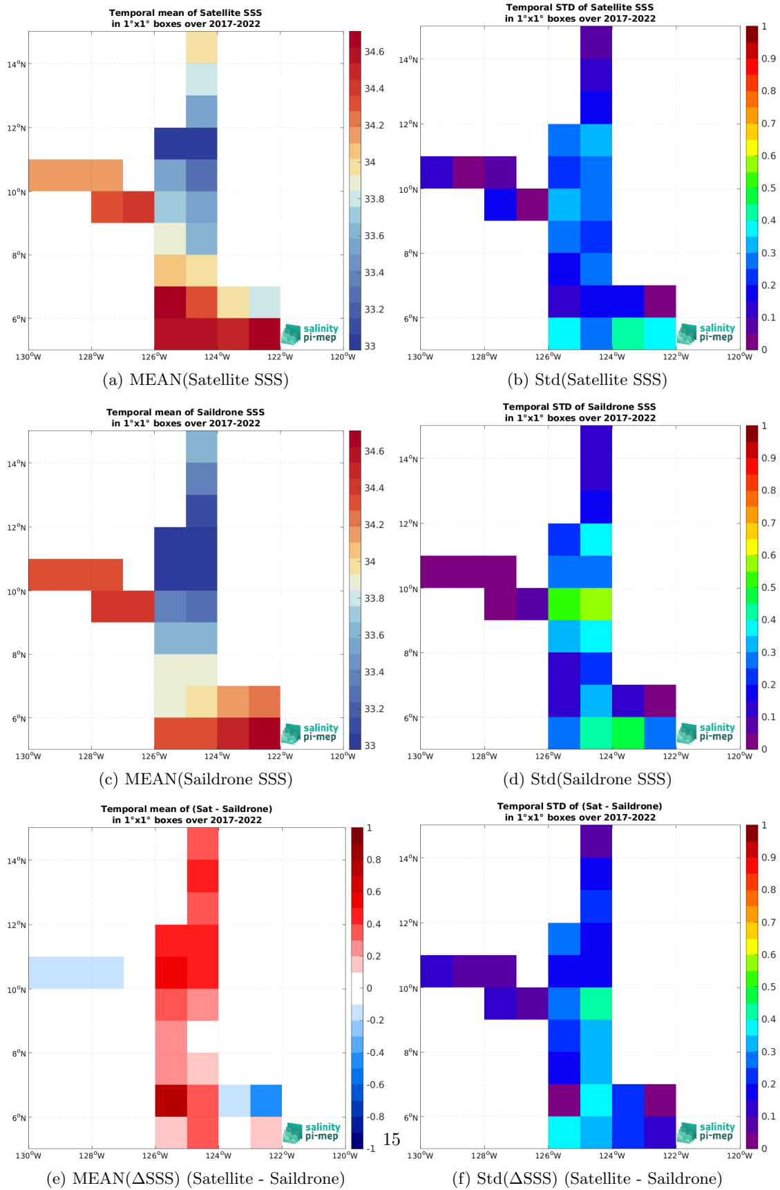
Figure 6: Temporal mean (left) and Std (right) of SSS from CCI SSS L4 Merged-OI v4.4 - 7-day running (ESA) (top), Saildrone (middle), and of \Delta SSS (Satellite - Saildrone). Only match-up pairs are used to generate these maps.
