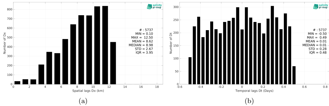
Figure 5: Histograms of the spatial (a) and temporal (b) lags between the location/time of the Saildrone (SPURS 2) measurement and the date of the corresponding CCI SSS L4 Merged-OI v4.4 - 7-day running (ESA) SSS pixel.
