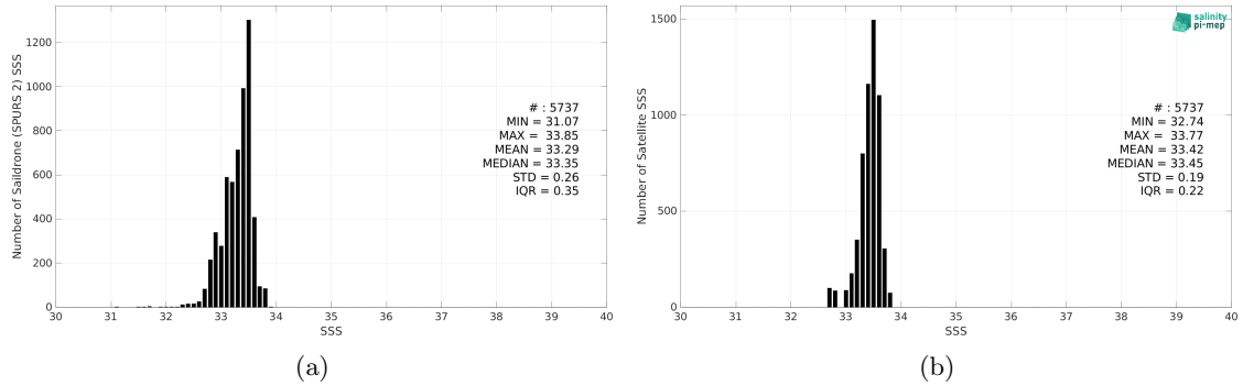
Figure 2: Histograms of SSS from Saildrone (SPURS 2) (a) and CCI SSS L4 Merged-OI v4.4 - 7-day running (ESA) (b) considering all match-up pairs per bins of 0.1 over the SPURS 2 Pi-MEP region and for the full satellite product period.
