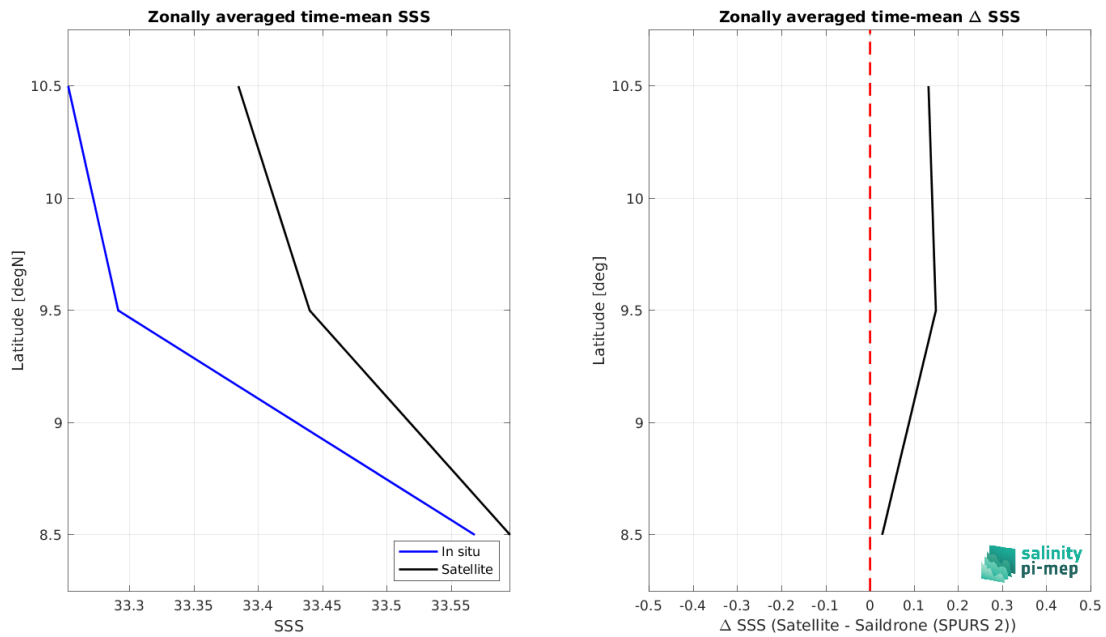
Figure 8: Left panel: Zonal mean SSS from CCI SSS L4 Merged-OI v4.4 - 7-day running (ESA) satellite product (black) and from Sairdron (SPURS 2) (blue). Right panel: Zonal mean of \Delta SSS (Satellite - Sairdron (SPURS 2)) for all the collected Pi-MEP match-up pairs estimated over the full satellite product period.
