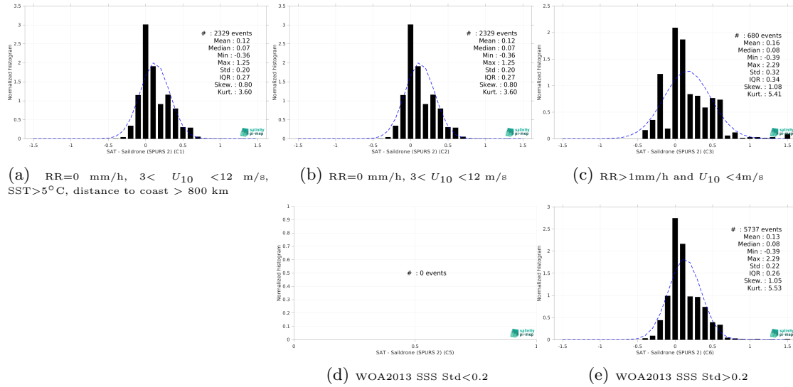
Figure 13: Normalized histogram of \Delta SSS (CCI SSS L4 Merged-OI v4.4 - 7-day running (ESA) - Saildrone (SPURS 2)) for 5 different subdatasets corresponding to: RR=0 mm/h, 3 < U_{10} < 12 m/s, SST > 5°C, distance to coast > 800 km (a), RR=0 mm/h, 3 < U_{10} < 12 m/s (b), RR > 1mm/h and U_{10} < 4 m/s (c), WOA2013 SSS Std < 0.2 (d), WOA2013 SSS Std > 0.2 (e).
