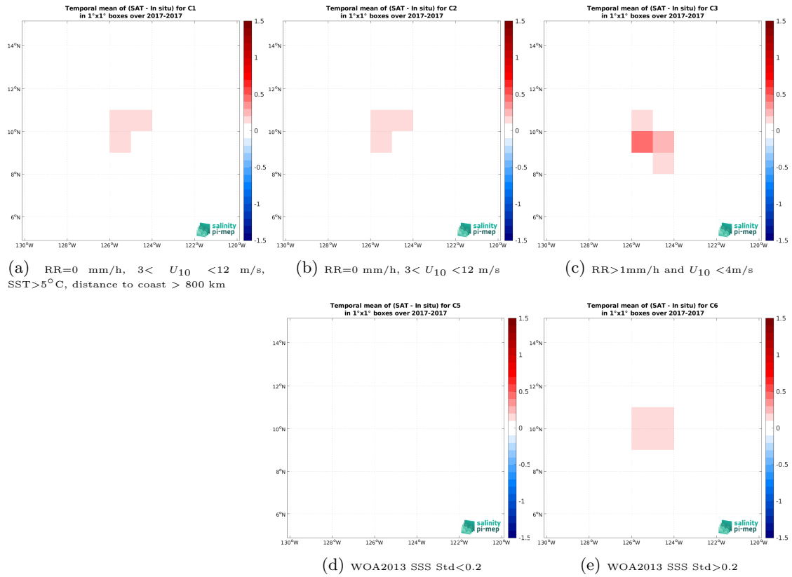
Figure 12: Temporal mean gridded over spatial boxes of size 1^{\circ}\times 1^{\circ} of \Delta\text{SSS} (CCI SSS L4 Merged-OI v4.4 - 7-day running (ESA) - Saildrone (SPURS 2)) for 5 different subdatasets corresponding to:RR=0 mm/h, 3 < U_{10} < 12 m/s, SST >5^{\circ}\text{C} , distance to coast > 800 km (a), RR=0 mm/h, 3 < U_{10} < 12 m/s (b), RR >1 mm/h and U_{10} < 4 m/s (c), WOA2013 SSS Std <0.2 (d), WOA2013 SSS Std >0.2 (e).
