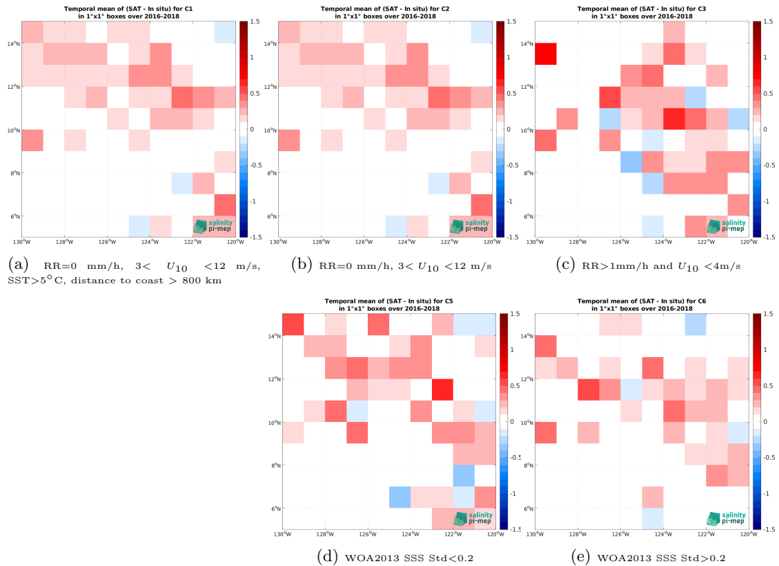
Figure 11: Temporal mean gridded over spatial boxes of size 1^\circ \times 1^\circ of \Delta SSS (CCI SSS L4 Merged-OI v4.4 - 7-day running (ESA) - Surface drifters) for 5 different subdatasets corresponding to:RR=0 mm/h, 3 < U_{10} < 12 m/s, SST >5^\circ C, distance to coast > 800 km (a), RR=0 mm/h, 3 < U_{10} < 12 m/s (b), RR >1 mm/h and U_{10} < 4 m/s (c), WOA2013 SSS Std <0.2 (d), WOA2013 SSS Std >0.2 (e).
