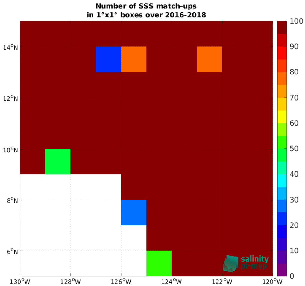
Figure 3: Number of SSS match-ups between Surface drifters SSS and the CCI SSS L4 Merged-OI v4.4 - 7-day running (ESA) SSS product for the SPURS 2 Pi-MEP region over 1^\circ \times 1^\circ boxes and for the full satellite product period.
