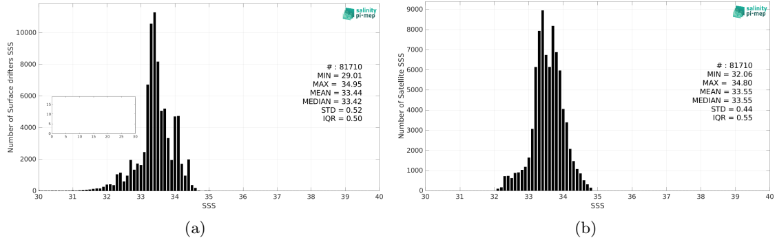
Figure 2: Histograms of SSS from Surface drifters (a) and CCI SSS L4 Merged-OI v4.4 - 7-day running (ESA) (b) considering all match-up pairs per bins of 0.1 over the SPURS 2 Pi-MEP region and for the full satellite product period.
