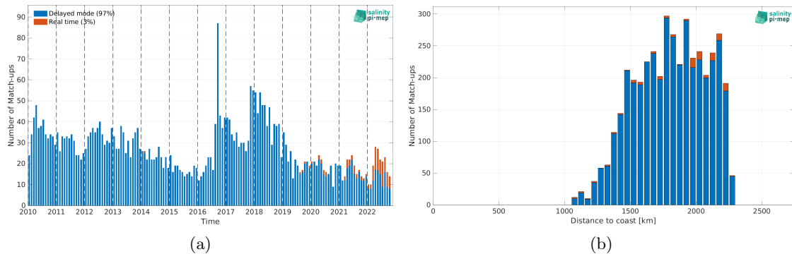
Figure 1: Number of match-ups between Argo and CCI SSS L4 Merged-OI v4.4 - 7-day running (ESA) SSS as a function of time (a) and as function of the distance to coast (b) over the SPURS 2 Pi-MEP region and for the full satellite product period.
