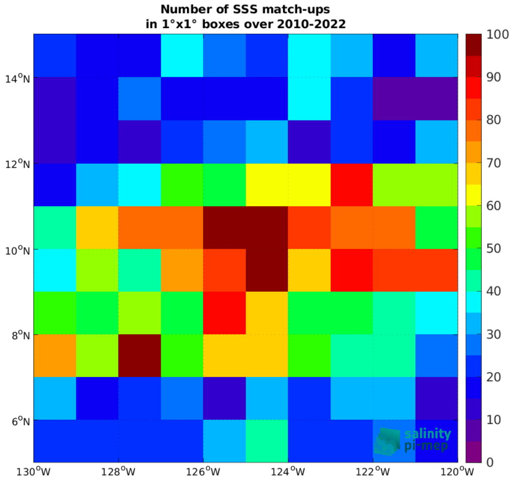
Figure 4: Number of SSS match-ups between Argo SSS and the CCI SSS L4 Merged-OI v4.4 - 7-day running (ESA) SSS product for the SPURS 2 Pi-MEP region over 1^\circ \times 1^\circ boxes and for the full satellite product period.
