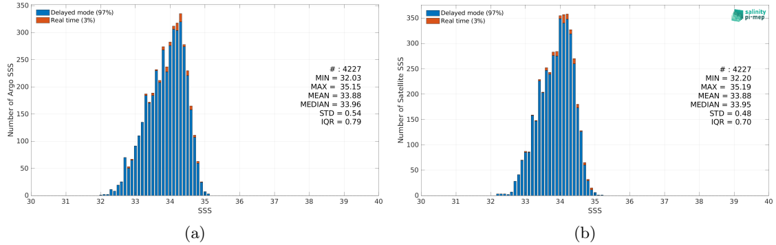
Figure 2: Histograms of SSS from Argo (a) and CCI SSS L4 Merged-OI v4.4 - 7-day running (ESA) (b) considering all match-up pairs per bins of 0.1 over the SPURS 2 Pi-MEP region and for the full satellite product period.
