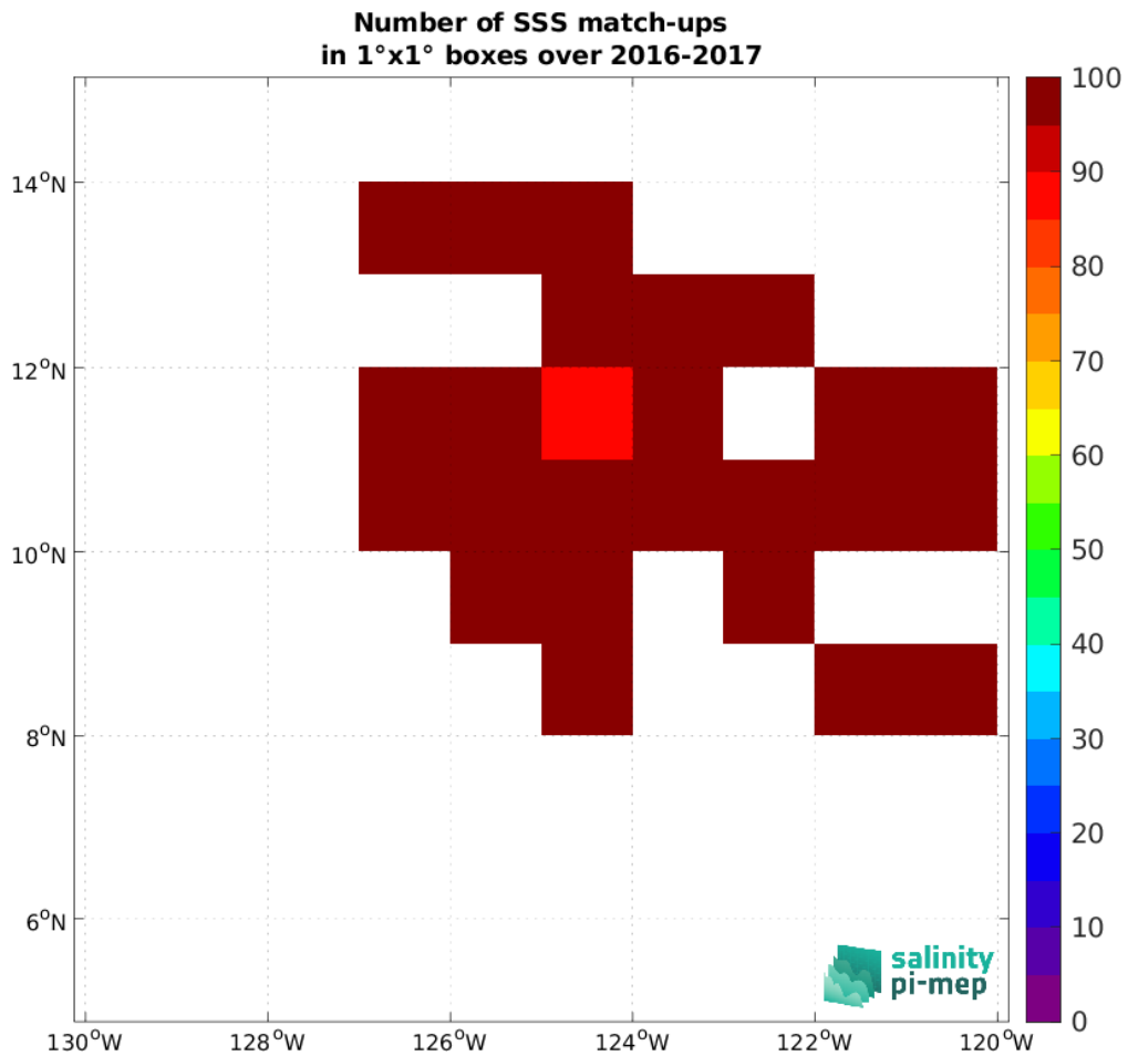
Figure 4: Number of SSS match-ups between Waveglider (SPURS 2) SSS and the CCI SSS L4 Merged-OI v4.4 - 30-day running (ESA) SSS product for the SPURS 2 Pi-MEP region over 1^\circ \times 1^\circ boxes and for the full satellite product period.
