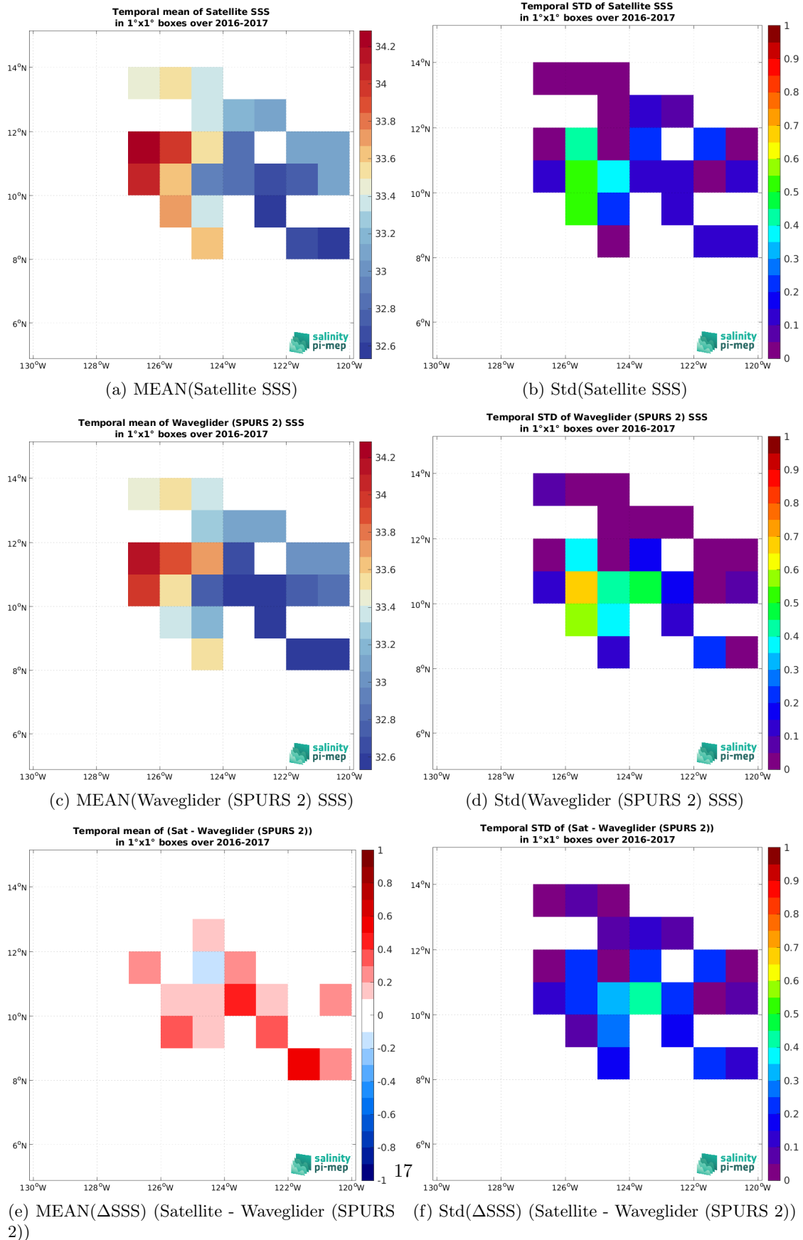
Figure 6: Temporal mean (left) and Std (right) of SSS from CCI SSS L4 Merged-OI v4.4 - 30-day running (ESA) (top), Waveglider (SPURS 2) (middle), and of \Delta SSS (Satellite - Waveglider (SPURS 2)). Only match-up pairs are used to generate these maps.
