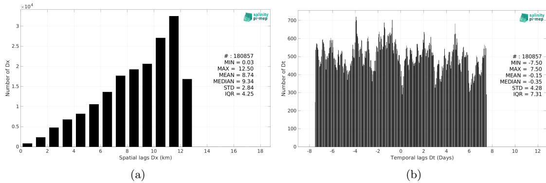
Figure 5: Histograms of the spatial (a) and temporal (b) lags between the location/time of the Waveglider (SPURS 2) measurement and the date of the corresponding CCI SSS L4 Merged-OI v4.4 - 30-day running (ESA) SSS pixel.
