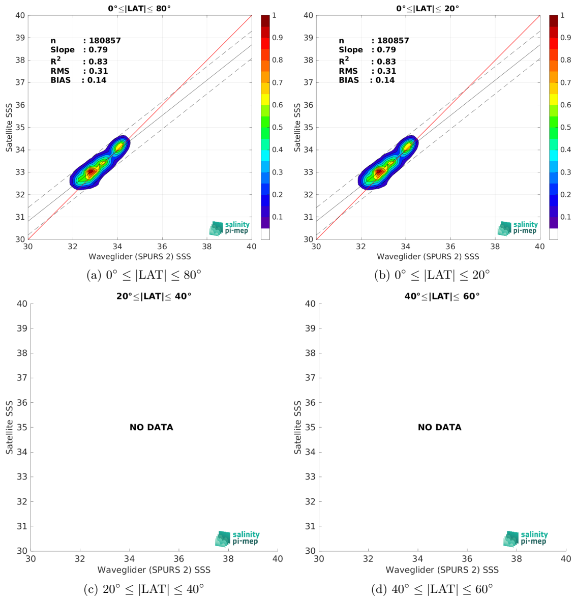
Figure 9: Contour maps of the concentration of CCI SSS L4 Merged-OI v4.4 - 30-day running (ESA) SSS (y-axis) versus Waveglider (SPURS 2) SSS (x-axis) at match-up pairs for different latitude bands. For each plot, the red line shows x=y . The black thin and dashed lines indicate a linear fit through the data cloud and the \pm 95\% confidence levels, respectively. The number match-up pairs n , the slope and R^2 coefficient of the linear fit, the root mean square (RMS) and the mean bias between satellite and in situ data are indicated for each latitude band in each plots.
