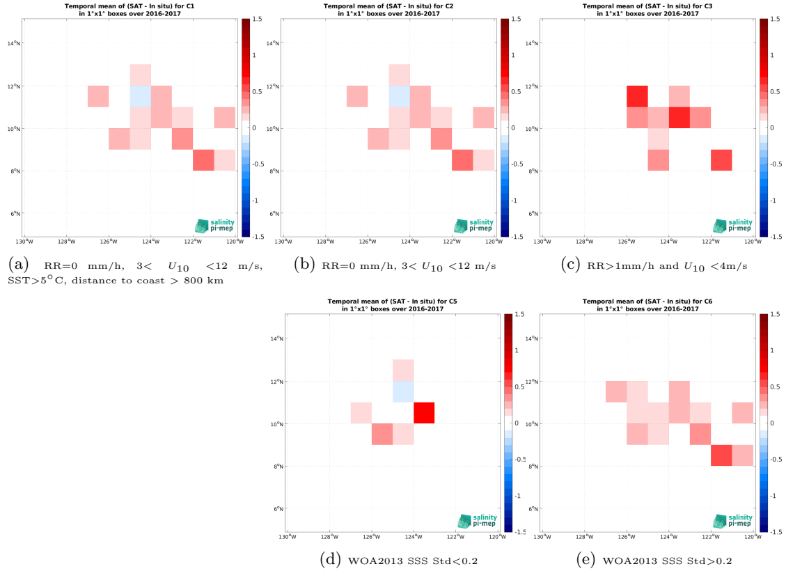
Figure 12: Temporal mean gridded over spatial boxes of size 1^{\circ}\times 1^{\circ} of \Delta\text{SSS} (CCI SSS L4 Merged-OI v4.4 - 30-day running (ESA) - Waveglider (SPURS 2)) for 5 different subdatasets corresponding to:RR=0 mm/h, 3 < U_{10} < 12 m/s, SST > 5^{\circ}\text{C} , distance to coast > 800 km (a), RR=0 mm/h, 3 < U_{10} < 12 m/s (b), RR > 1 mm/h and U_{10} < 4 m/s (c), WOA2013 SSS Std < 0.2 (d), WOA2013 SSS Std > 0.2 (e).
