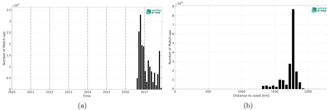
Figure 1: Number of match-ups between Waveglider (SPURS 2) and CCI SSS L4 Merged-OI v4.4 - 30-day running (ESA) SSS as a function of time (a) and as function of the distance to coast (b) over the SPURS 2 Pi-MEP region and for the full satellite product period.
