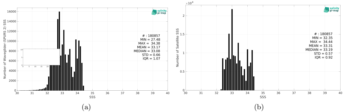
Figure 2: Histograms of SSS from Waveglider (SPURS 2) (a) and CCI SSS L4 Merged-OI v4.4 - 30-day running (ESA) (b) considering all match-up pairs per bins of 0.1 over the SPURS 2 Pi-MEP region and for the full satellite product period.
