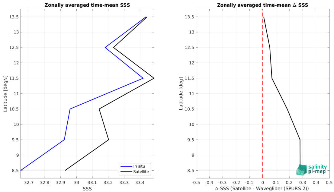
Figure 8: Left panel: Zonal mean SSS from CCI SSS L4 Merged-OI v4.4 - 30-day running (ESA) satellite product (black) and from Waveglider (SPURS 2) (blue). Right panel: Zonal mean of \Delta SSS (Satellite - Waveglider (SPURS 2)) for all the collected Pi-MEP match-up pairs estimated over the full satellite product period.
