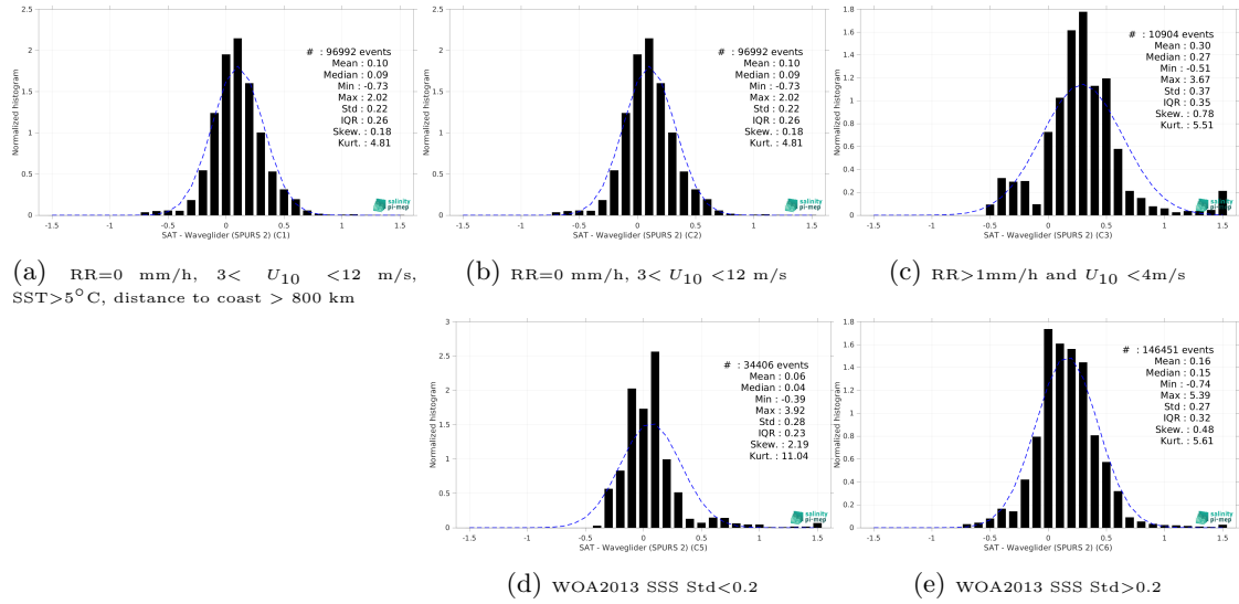
Figure 13: Normalized histogram of \Delta SSS (CCI SSS L4 Merged-OI v4.4 - 30-day running (ESA) - Waveglider (SPURS 2)) for 5 different subdatasets corresponding to: RR=0 mm/h, 3 < U_{10} < 12 m/s, SST>5°C, distance to coast > 800 km (a), RR=0 mm/h, 3 < U_{10} < 12 m/s (b), RR>1mm/h and U_{10} < 4 m/s (c), WOA2013 SSS Std<0.2 (d), WOA2013 SSS Std>0.2 (e).
