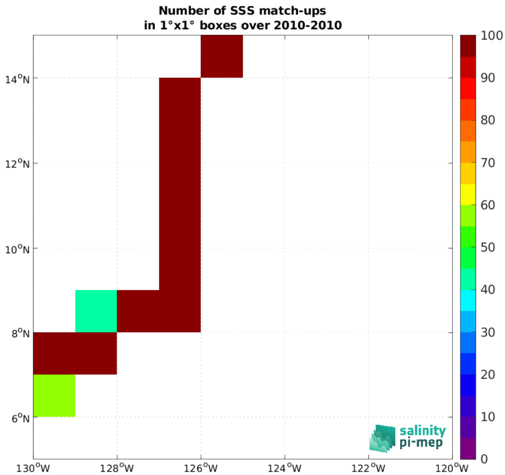
Figure 4: Number of SSS match-ups between TSG (GOSUD-Sailing-ship) SSS and the CCI SSS L4 Merged-OI v4.4 - 30-day running (ESA) SSS product for the SPURS 2 Pi-MEP region over 1^\circ \times 1^\circ boxes and for the full satellite product period.
