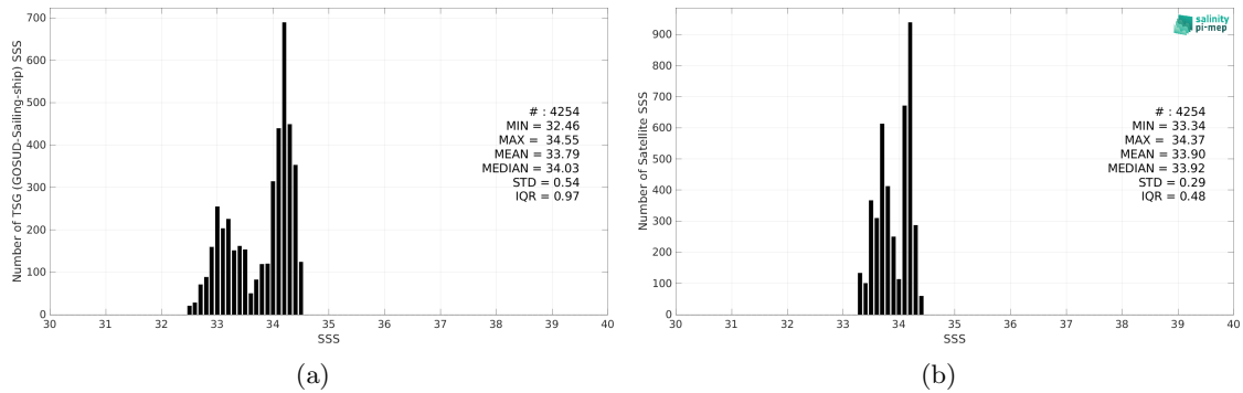
Figure 2: Histograms of SSS from TSG (GOSUD-Sailing-ship) (a) and CCI SSS L4 Merged-OI v4.4 - 30-day running (ESA) (b) considering all match-up pairs per bins of 0.1 over the SPURS 2 Pi-MEP region and for the full satellite product period.
