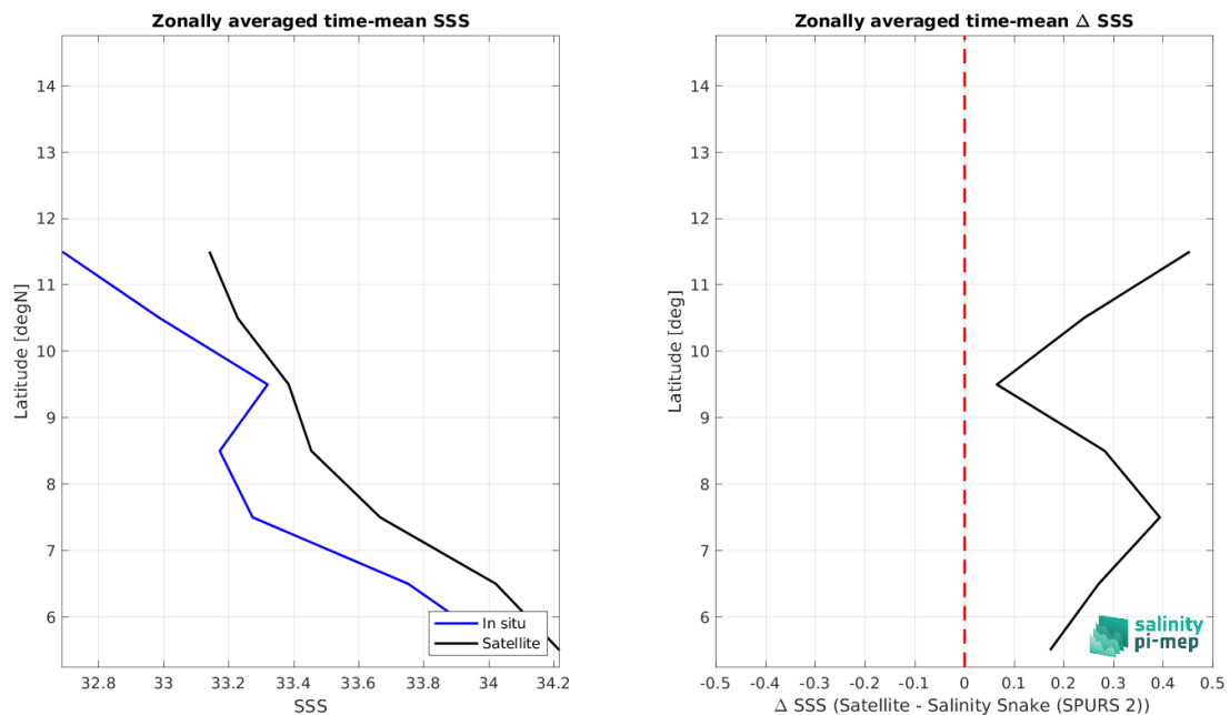
Figure 8: Left panel: Zonal mean SSS from CCI SSS L4 Merged-OI v4.4 - 30-day running (ESA) satellite product (black) and from Salinity Snake (SPURS 2) (blue). Right panel: Zonal mean of \Delta SSS (Satellite - Salinity Snake (SPURS 2)) for all the collected Pi-MEP match-up pairs estimated over the full satellite product period.
