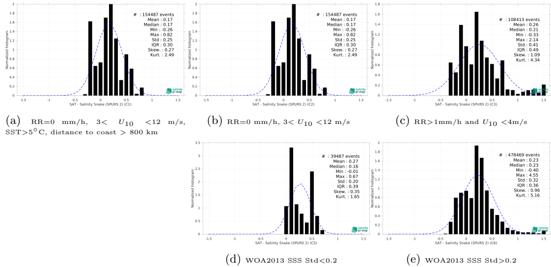
Figure 13: Normalized histogram of \Delta SSS (CCI SSS L4 Merged-OI v4.4 - 30-day running (ESA) - Salinity Snake (SPURS 2)) for 5 different subdatasets corresponding to: RR=0 mm/h, 3 < U_{10} < 12 m/s, SST > 5°C, distance to coast > 800 km (a), RR=0 mm/h, 3 < U_{10} < 12 m/s (b), RR > 1mm/h and U_{10} < 4 m/s (c), WOA2013 SSS Std < 0.2 (d), WOA2013 SSS Std > 0.2 (e).
