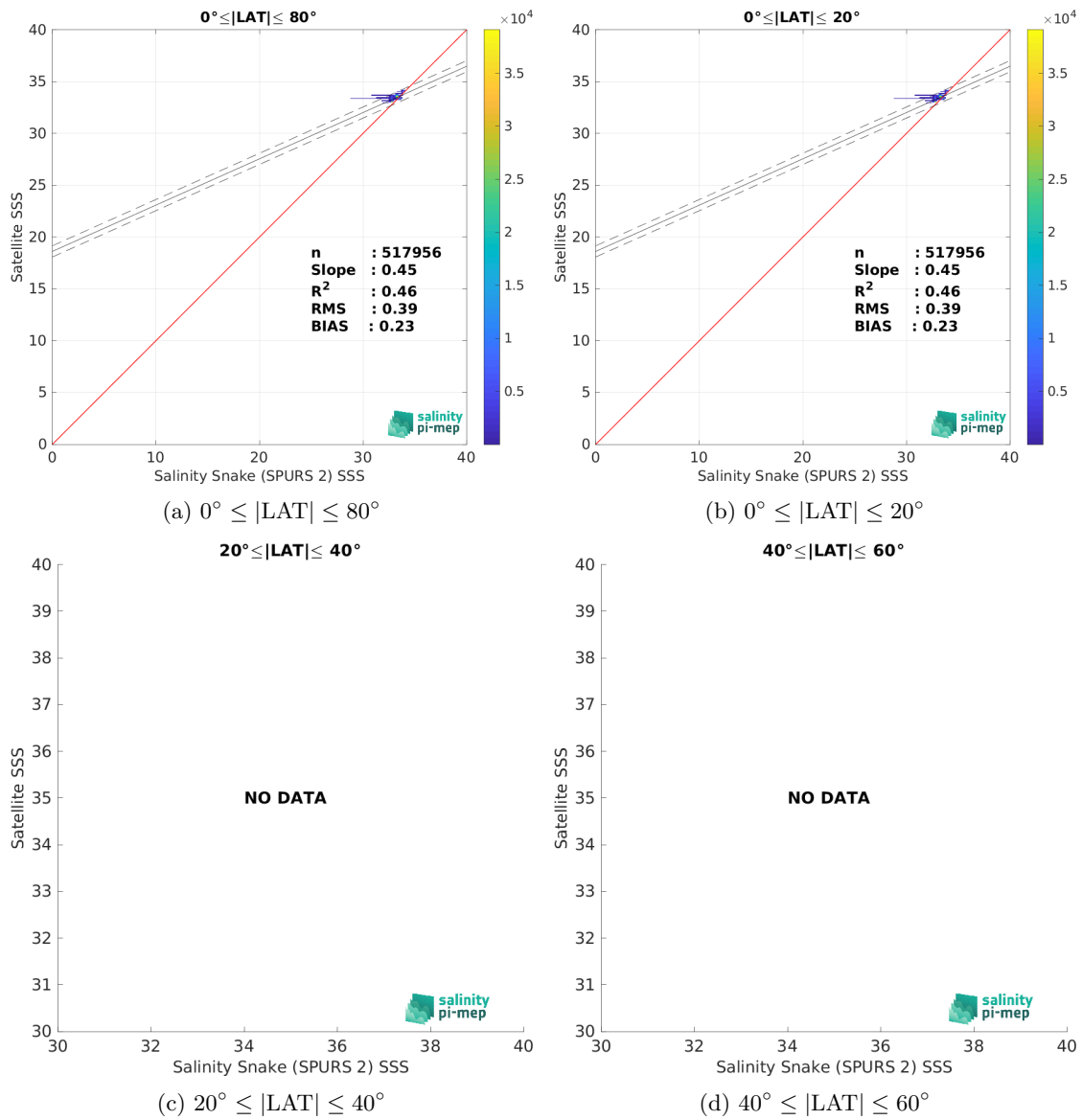
Figure 9: Contour maps of the concentration of CCI SSS L4 Merged-OI v4.4 - 30-day running (ESA) SSS (y-axis) versus Salinity Snake (SPURS 2) SSS (x-axis) at match-up pairs for different latitude bands. For each plot, the red line shows x=y . The black thin and dashed lines indicate a linear fit through the data cloud and the \pm 95\% confidence levels, respectively. The number match-up pairs n , the slope and R^2 coefficient of the linear fit, the root mean square (RMS) and the mean bias between satellite and in situ data are indicated for each latitude band in each plots.
