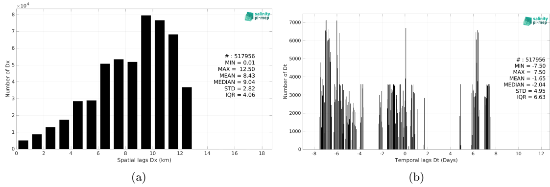
Figure 5: Histograms of the spatial (a) and temporal (b) lags between the location/time of the Salinity Snake (SPURS 2) measurement and the date of the corresponding CCI SSS L4 Merged-OI v4.4 - 30-day running (ESA) SSS pixel.
