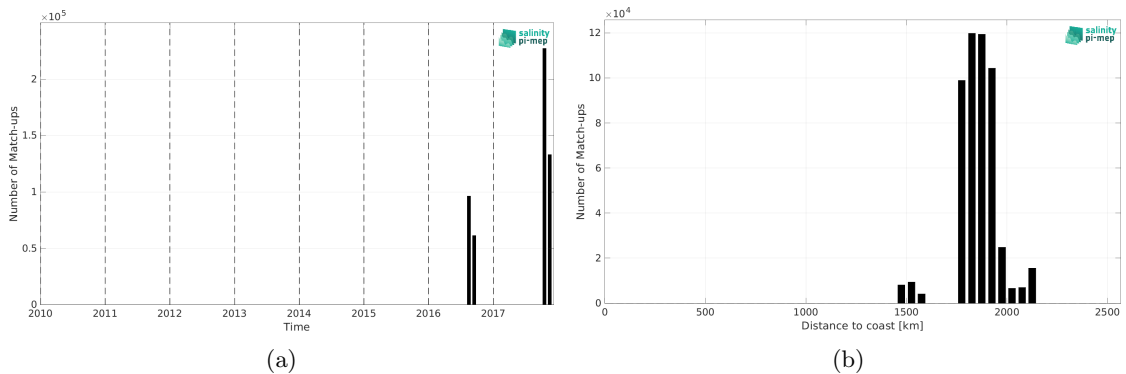
Figure 1: Number of match-ups between Salinity Snake (SPURS 2) and CCI SSS L4 Merged-OI v4.4 - 30-day running (ESA) SSS as a function of time (a) and as function of the distance to coast (b) over the SPURS 2 Pi-MEP region and for the full satellite product period.
