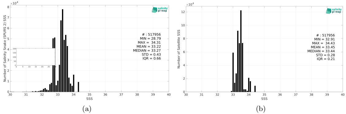
Figure 2: Histograms of SSS from Salinity Snake (SPURS 2) (a) and CCI SSS L4 Merged-OI v4.4 - 30-day running (ESA) (b) considering all match-up pairs per bins of 0.1 over the SPURS 2 Pi-MEP region and for the full satellite product period.
