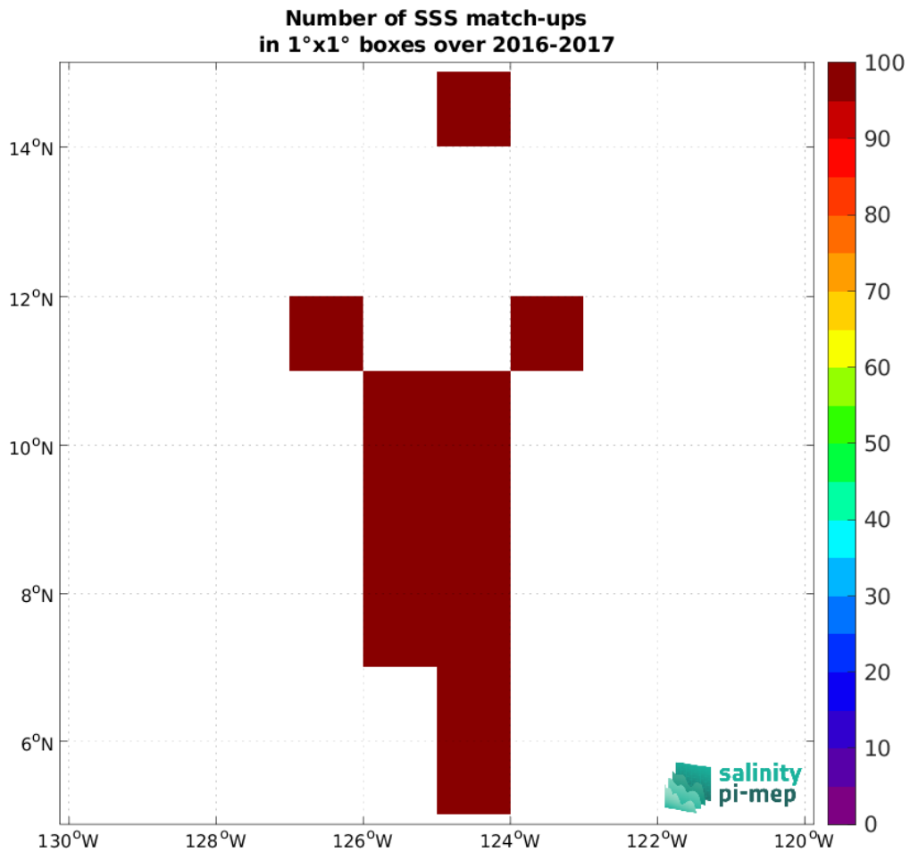
Figure 4: Number of SSS match-ups between Salinity Snake (SPURS 2) SSS and the CCI SSS L4 Merged-OI v4.4 - 30-day running (ESA) SSS product for the SPURS 2 Pi-MEP region over 1^\circ \times 1^\circ boxes and for the full satellite product period.
