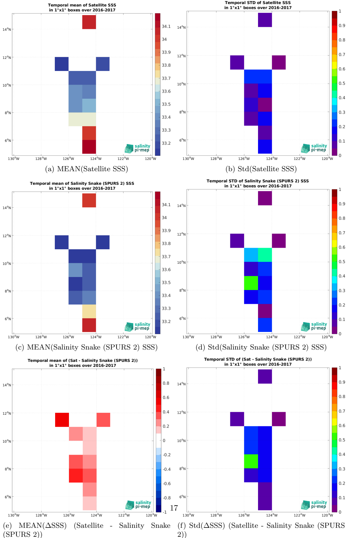
Figure 6: Temporal mean (left) and Std (right) of SSS from CCI SSS L4 Merged-OI v4.4 - 30-day running (ESA) (top), Salinity Snake (SPURS 2) (middle), and of \Delta SSS (Satellite - Salinity Snake (SPURS 2)). Only match-up pairs are used to generate these maps.
