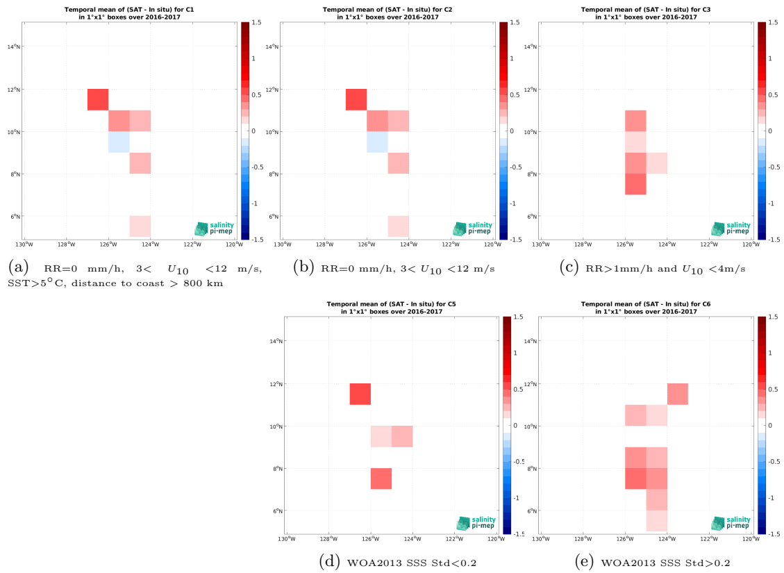
Figure 12: Temporal mean gridded over spatial boxes of size 1^\circ \times 1^\circ of \Delta\text{SSS} (CCI SSS L4 Merged-OI v4.4 - 30-day running (ESA) - Salinity Snake (SPURS 2)) for 5 different subdatasets corresponding to: RR=0 mm/h, 3 < U_{10} < 12 m/s, SST > 5^\circ\text{C} , distance to coast > 800 km (a), RR=0 mm/h, 3 < U_{10} < 12 m/s (b), RR > 1 mm/h and U_{10} < 4 m/s (c), WOA2013 SSS Std < 0.2 (d), WOA2013 SSS Std > 0.2 (e).
