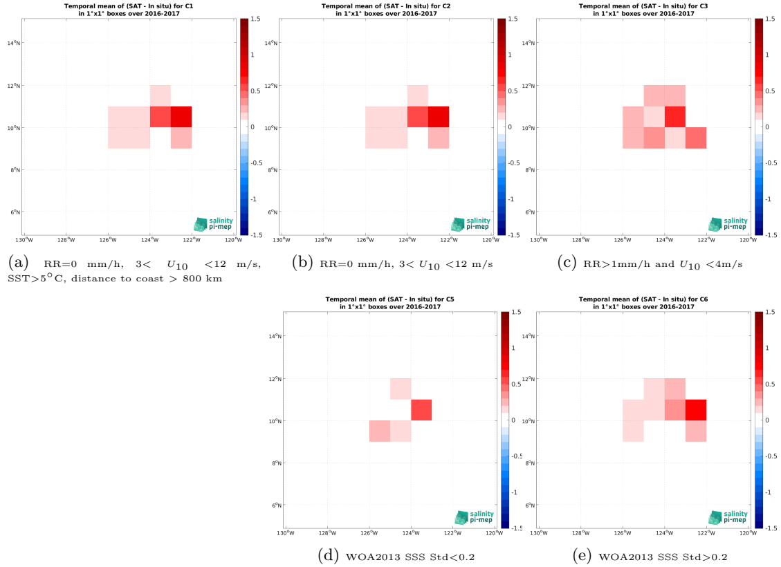
Figure 12: Temporal mean gridded over spatial boxes of size 1^{\circ}\times 1^{\circ} of \Delta\text{SSS} (CCI SSS L4 Merged-OI v4.4 - 30-day running (ESA) - Seaglider (SPURS 2)) for 5 different subdatasets corresponding to:RR=0 mm/h, 3 < U_{10} < 12 m/s, SST >5^{\circ}\text{C} , distance to coast > 800 km (a), RR=0 mm/h, 3 < U_{10} < 12 m/s (b), RR >1 mm/h and U_{10} < 4 m/s (c), WOA2013 SSS Std <0.2 (d), WOA2013 SSS Std >0.2 (e).
