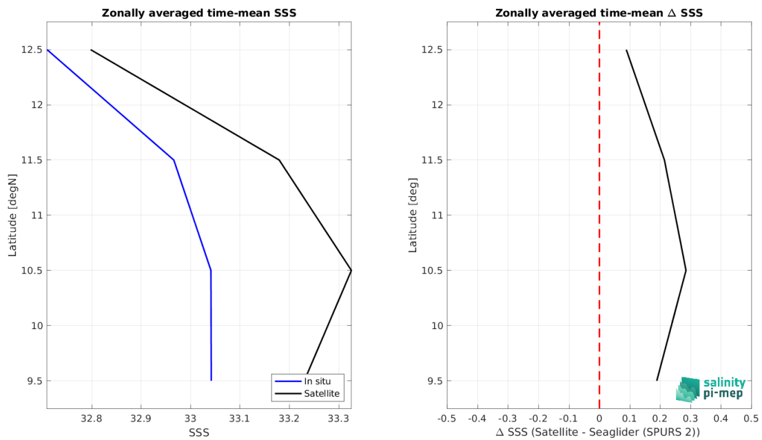
Figure 8: Left panel: Zonal mean SSS from CCI SSS L4 Merged-OI v4.4 - 30-day running (ESA) satellite product (black) and from Seaglider (SPURS 2) (blue). Right panel: Zonal mean of \Delta SSS (Satellite - Seaglider (SPURS 2)) for all the collected Pi-MEP match-up pairs estimated over the full satellite product period.
