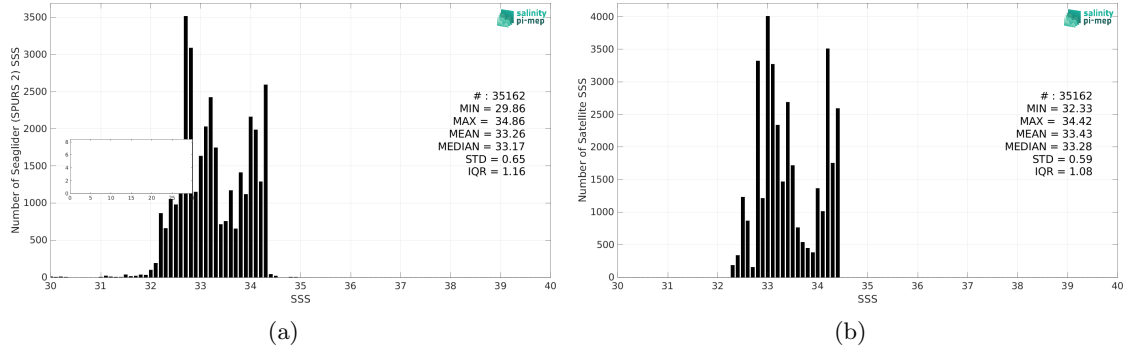
Figure 2: Histograms of SSS from Seaglider (SPURS 2) (a) and CCI SSS L4 Merged-OI v4.4 - 30-day running (ESA) (b) considering all match-up pairs per bins of 0.1 over the SPURS 2 Pi-MEP region and for the full satellite product period.
