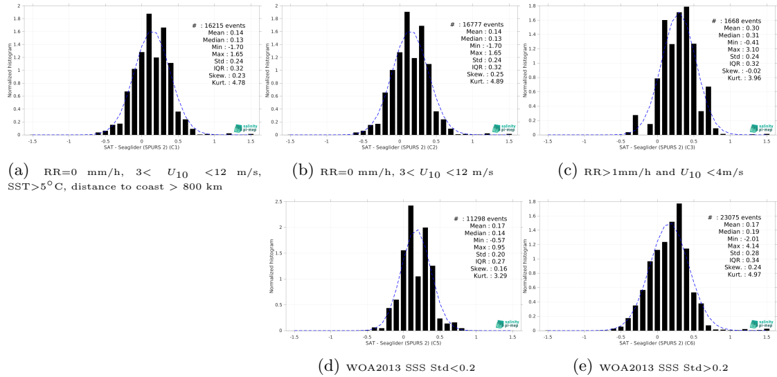
Figure 13: Normalized histogram of \Delta\text{SSS} (CCI SSS L4 Merged-OI v4.4 - 30-day running (ESA) - Seaglider (SPURS 2)) for 5 different subdatasets corresponding to: RR=0 mm/h, 3 < U_{10} < 12 m/s, SST >5^{\circ}\text{C} , distance to coast > 800 km (a), RR=0 mm/h, 3 < U_{10} < 12 m/s (b), RR >1 mm/h and U_{10} < 4 m/s (c), WOA2013 SSS Std <0.2 (d), WOA2013 SSS Std >0.2 (e).
