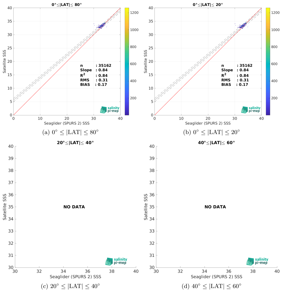
Figure 9: Contour maps of the concentration of CCI SSS L4 Merged-OI v4.4 - 30-day running (ESA) SSS (y-axis) versus Seaglider (SPURS 2) SSS (x-axis) at match-up pairs for different latitude bands. For each plot, the red line shows x=y . The black thin and dashed lines indicate a linear fit through the data cloud and the \pm 95\% confidence levels, respectively. The number match-up pairs n , the slope and R^2 coefficient of the linear fit, the root mean square (RMS) and the mean bias between satellite and in situ data are indicated for each latitude band in each plots.
