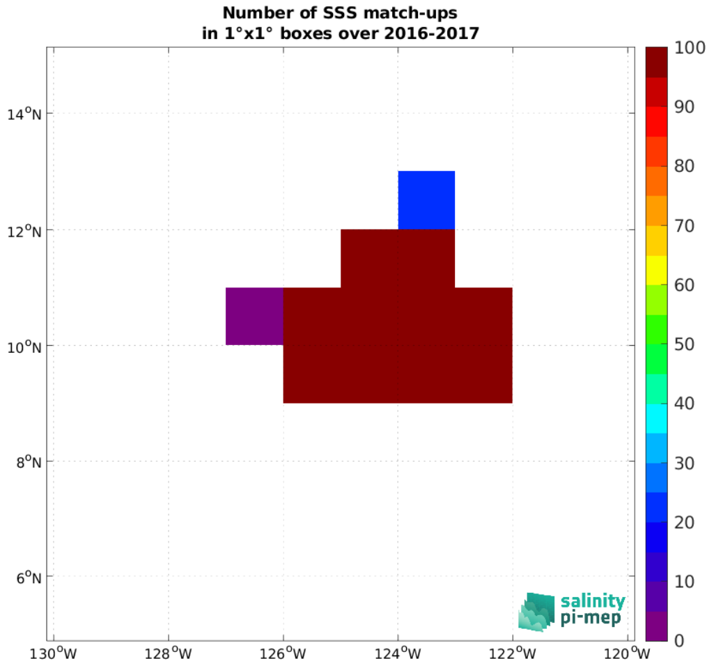
Figure 4: Number of SSS match-ups between Seaglider (SPURS 2) SSS and the CCI SSS L4 Merged-OI v4.4 - 30-day running (ESA) SSS product for the SPURS 2 Pi-MEP region over 1^\circ \times 1^\circ boxes and for the full satellite product period.
