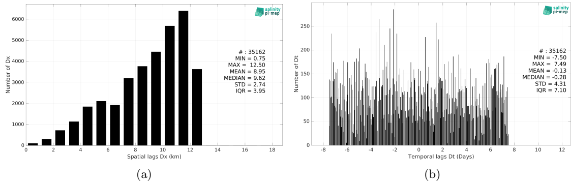
Figure 5: Histograms of the spatial (a) and temporal (b) lags between the location/time of the Seaglider (SPURS 2) measurement and the date of the corresponding CCI SSS L4 Merged-OI v4.4 - 30-day running (ESA) SSS pixel.
