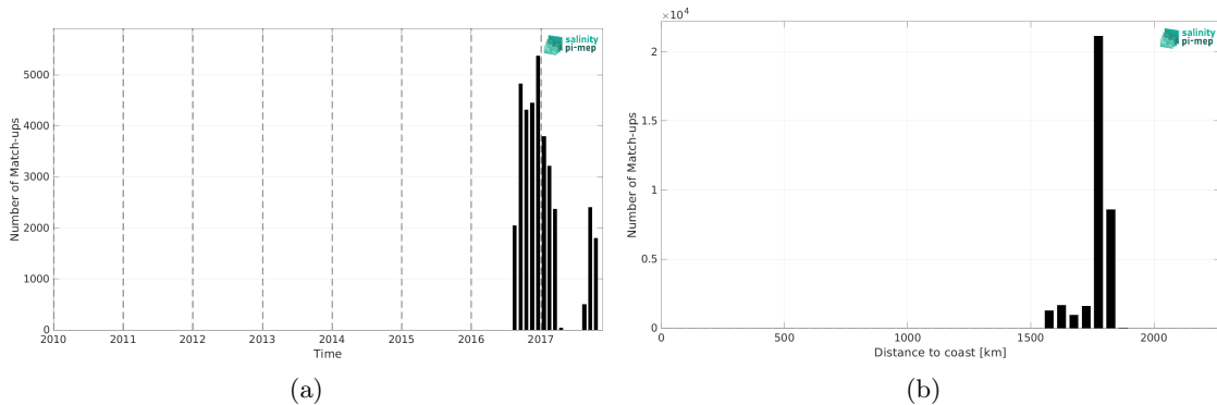
Figure 1: Number of match-ups between Seaglider (SPURS 2) and CCI SSS L4 Merged-OI v4.4 - 30-day running (ESA) SSS as a function of time (a) and as function of the distance to coast (b) over the SPURS 2 Pi-MEP region and for the full satellite product period.
