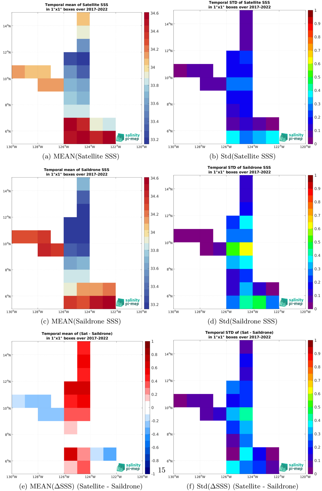
Figure 6: Temporal mean (left) and Std (right) of SSS from CCI SSS L4 Merged-OI v4.4 - 30-day running (ESA) (top), Saildrone (middle), and of \Delta SSS (Satellite - Saildrone). Only match-up pairs are used to generate these maps.
