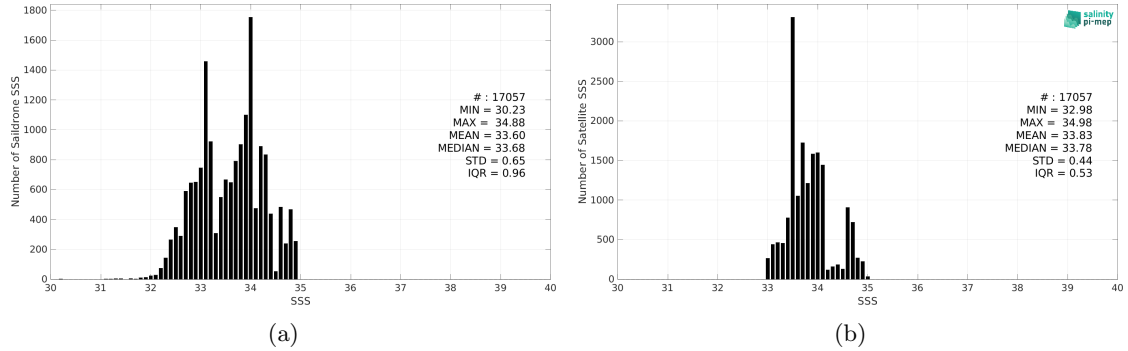
Figure 2: Histograms of SSS from Saildrone (a) and CCI SSS L4 Merged-OI v4.4 - 30-day running (ESA) (b) considering all match-up pairs per bins of 0.1 over the SPURS 2 Pi-MEP region and for the full satellite product period.
