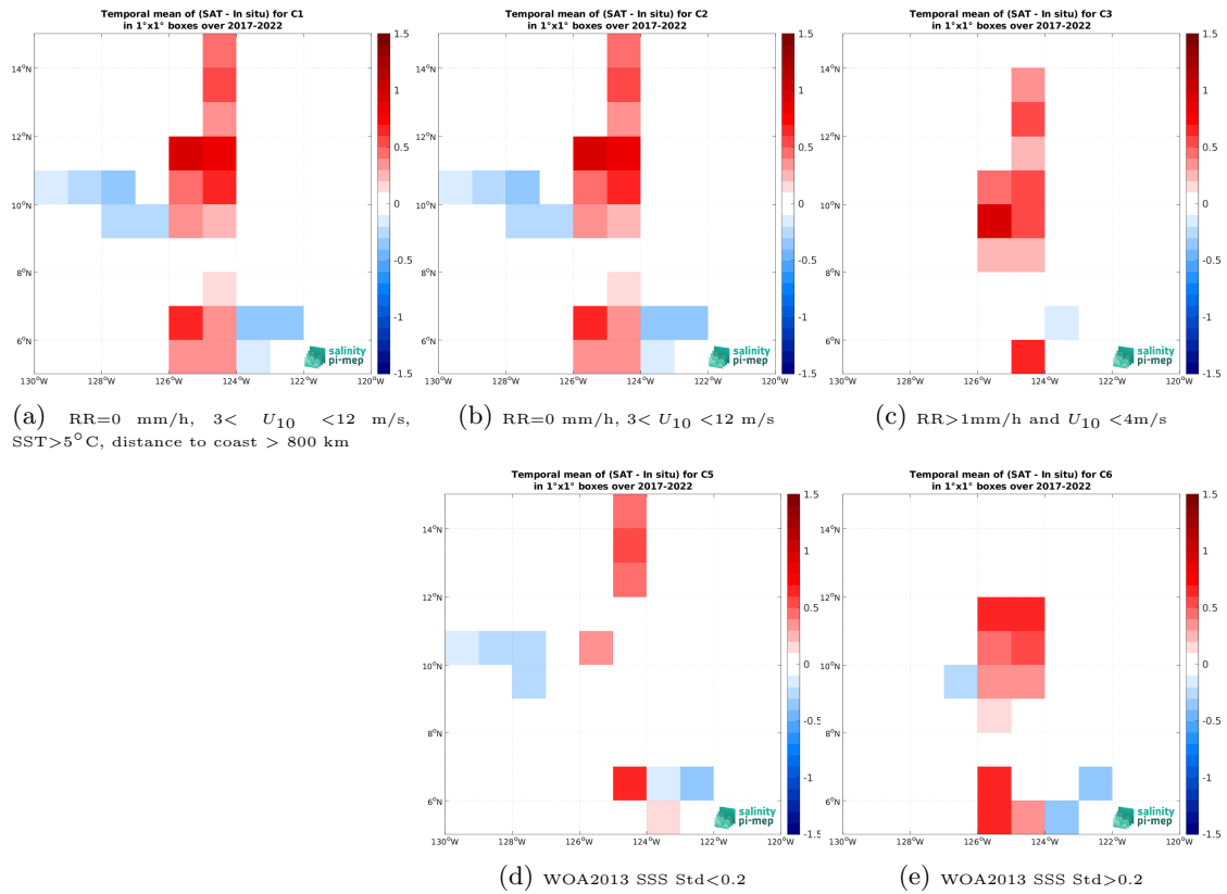
Figure 12: Temporal mean gridded over spatial boxes of size 1^\circ \times 1^\circ of \Delta\text{SSS} (CCI SSS L4 Merged-OI v4.4 - 30-day running (ESA) - Saildrone) for 5 different subdatasets corresponding to:RR=0 mm/h, 3 < U_{10} < 12 m/s, SST >5^\circ\text{C} , distance to coast > 800 km (a), RR=0 mm/h, 3 < U_{10} < 12 m/s (b), RR >1 mm/h and U_{10} < 4 m/s (c), WOA2013 SSS Std <0.2 (d), WOA2013 SSS Std >0.2 (e).
