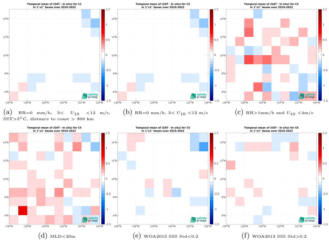
Figure 12: Temporal mean gridded over spatial boxes of size 1^\circ \times 1^\circ of \Delta SSS (CCI SSS L4 Merged-OI v4.4 - 30-day running (ESA) - Argo) for 6 different subdatasets corresponding to:RR=0 mm/h, 3 < U_{10} < 12 m/s, SST >5^\circ C, distance to coast > 800 km (a), RR=0 mm/h, 3 < U_{10} < 12 m/s (b), RR >1 mm/h and U_{10} < 4 m/s (c),MLD <20 m (d),WOA2013 SSS Std <0.2 (e),WOA2013 SSS Std >0.2 (f).
