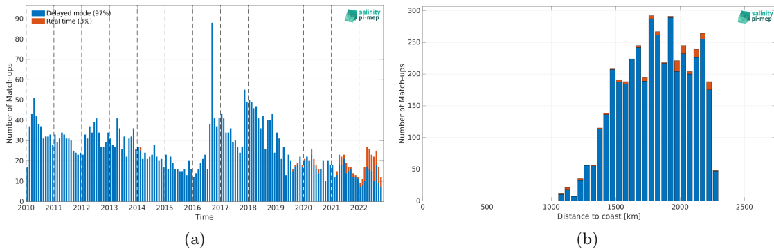
Figure 1: Number of match-ups between Argo and CCI SSS L4 Merged-OI v4.4 - 30-day running (ESA) SSS as a function of time (a) and as function of the distance to coast (b) over the SPURS 2 Pi-MEP region and for the full satellite product period.
