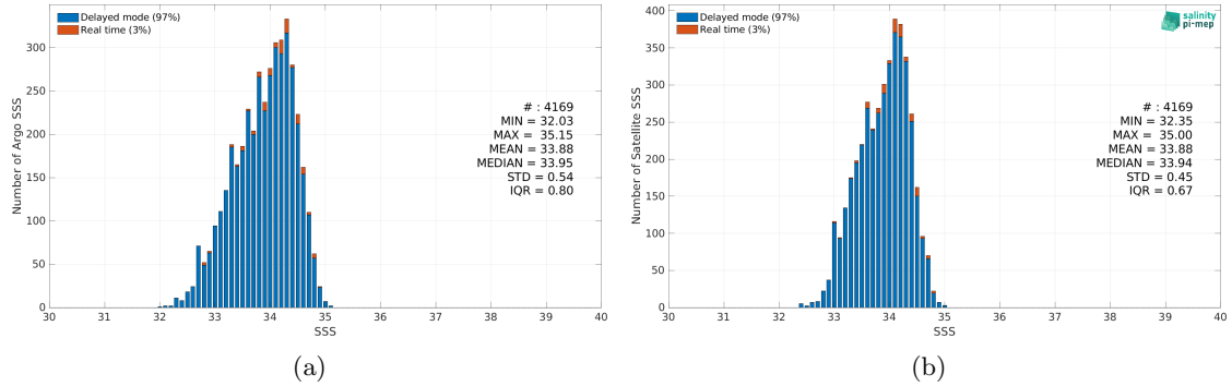
Figure 2: Histograms of SSS from Argo (a) and CCI SSS L4 Merged-OI v4.4 - 30-day running (ESA) (b) considering all match-up pairs per bins of 0.1 over the SPURS 2 Pi-MEP region and for the full satellite product period.
