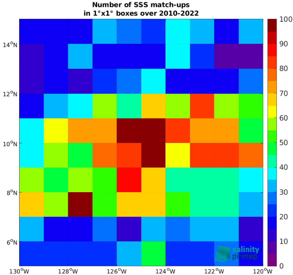
Figure 4: Number of SSS match-ups between Argo SSS and the CCI SSS L4 Merged-OI v4.4 - 30-day running (ESA) SSS product for the SPURS 2 Pi-MEP region over 1^\circ \times 1^\circ boxes and for the full satellite product period.
