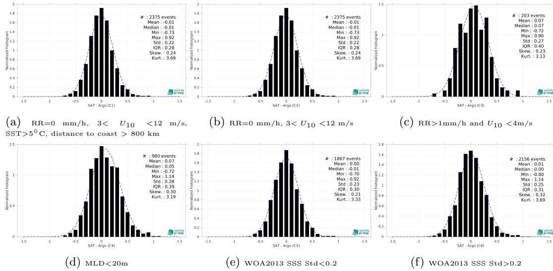
Figure 13: Normalized histogram of \Delta\text{SSS} (CCI SSS L4 Merged-OI v4.4 - 30-day running (ESA) - Argo) for 6 different subdatasets corresponding to: RR=0 mm/h, 3 < U_{10} < 12 m/s, SST>5°C, distance to coast > 800 km (a), RR=0 mm/h, 3 < U_{10} < 12 m/s (b), RR>1mm/h and U_{10} < 4 m/s (c), MLD<20m (d), WOA2013 SSS Std<0.2 (e), WOA2013 SSS Std>0.2 (f).
