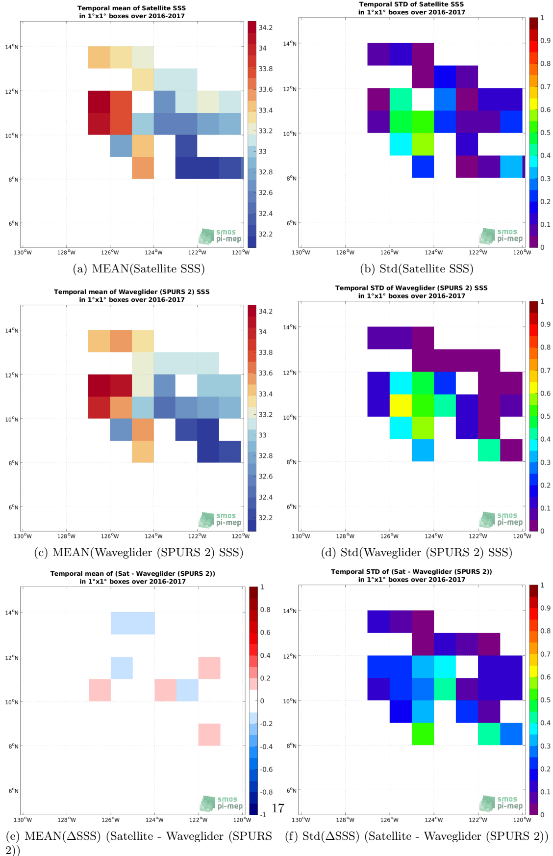
Figure 6: Temporal mean (left) and Std (right) of SSS from CCI SSS L4 Merged-OI v3.2 - 7-day running (ESA) (top), Waveglider (SPURS 2) (middle), and of \Delta SSS (Satellite - Waveglider (SPURS 2)). Only match-up pairs are used to generate these maps.
