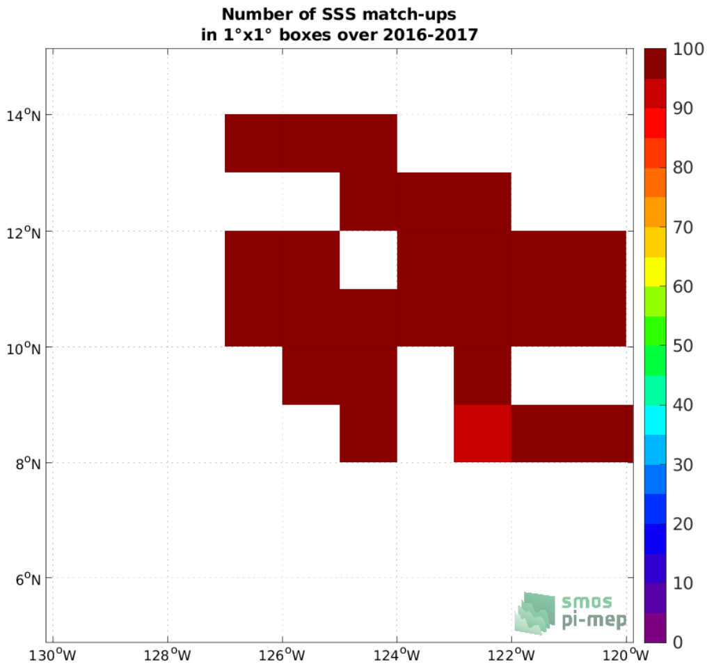
Figure 4: Number of SSS match-ups between Waveglider (SPURS 2) SSS and the CCI SSS L4 Merged-OI v3.2 - 7-day running (ESA) SSS product for the SPURS 2 Pi-MEP region over 1°x1° boxes and for the full satellite product period.
