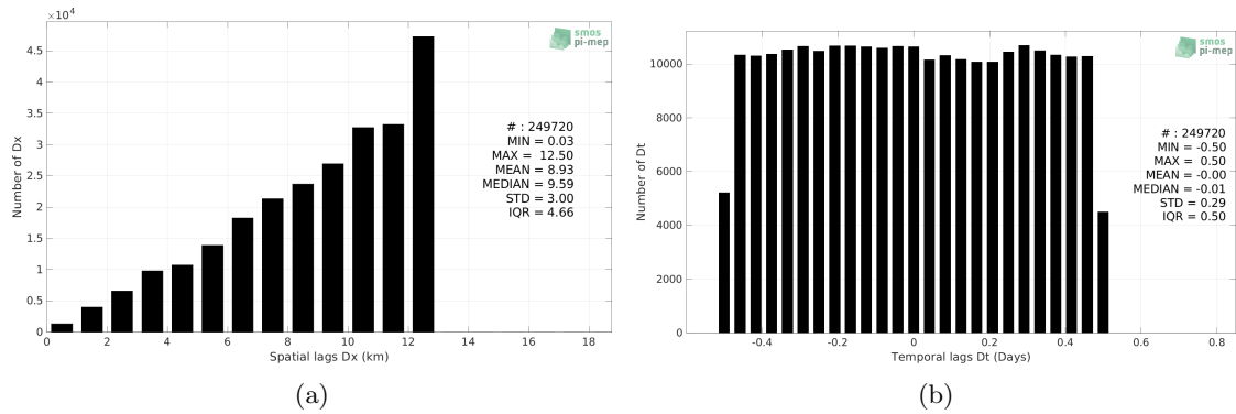
Figure 5: Histograms of the spatial (a) and temporal (b) lags between the location/time of the Waveglider (SPURS 2) measurement and the date of the corresponding CCI SSS L4 Merged-OI v3.2 - 7-day running (ESA) SSS pixel.
