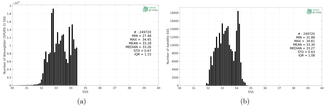
Figure 2: Histograms of SSS from Waveglider (SPURS 2) (a) and CCI SSS L4 Merged-OI v3.2 - 7-day running (ESA) (b) considering all match-up pairs per bins of 0.1 over the SPURS 2 Pi-MEP region and for the full satellite product period.
