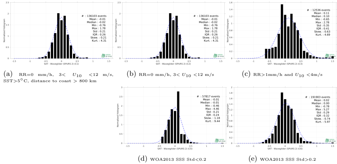
Figure 13: Normalized histogram of \Delta SSS (CCI SSS L4 Merged-OI v3.2 - 7-day running (ESA) - Waveglider (SPURS 2)) for 5 different subdatasets corresponding to: RR=0 mm/h, 3 < U_{10} < 12 m/s, SST>5°C, distance to coast > 800 km (a), RR=0 mm/h, 3 < U_{10} < 12 m/s (b), RR>1mm/h and U_{10} < 4 m/s (c), WOA2013 SSS Std<0.2 (d), WOA2013 SSS Std>0.2 (e).
