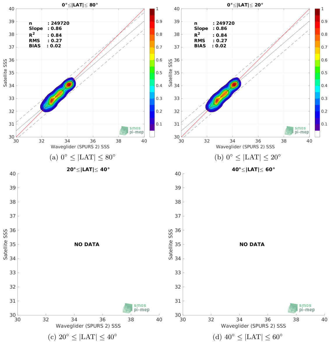
Figure 9: Contour maps of the concentration of CCI SSS L4 Merged-OI v3.2 - 7-day running (ESA) SSS (y-axis) versus Waveglider (SPURS 2) SSS (x-axis) at match-up pairs for different latitude bands. For each plot, the red line shows x=y . The black thin and dashed lines indicate a linear fit through the data cloud and the \pm 95\% confidence levels, respectively. The number match-up pairs n , the slope and R^2 coefficient of the linear fit, the root mean square (RMS) and the mean bias between satellite and in situ data are indicated for each latitude band in each plots.
