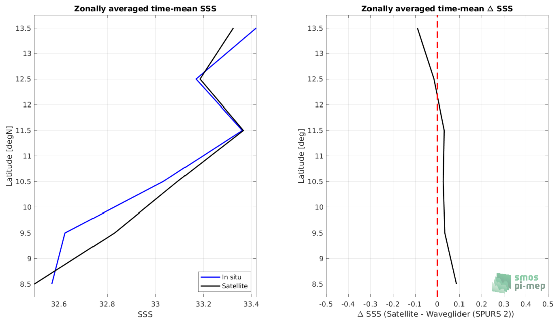
Figure 8: Left panel: Zonal mean SSS from CCI SSS L4 Merged-OI v3.2 - 7-day running (ESA) satellite product (black) and from Waveglider (SPURS 2) (blue). Right panel: Zonal mean of \Delta SSS (Satellite - Waveglider (SPURS 2)) for all the collected Pi-MEP match-up pairs estimated over the full satellite product period.
