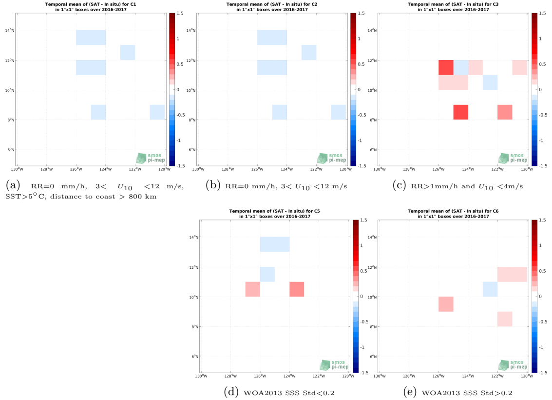
Figure 12: Temporal mean gridded over spatial boxes of size 1^{\circ}\times 1^{\circ} of \Delta\text{SSS} (CCI SSS L4 Merged-OI v3.2 - 7-day running (ESA) - Waveglider (SPURS 2)) for 5 different subdatasets corresponding to:RR=0 mm/h, 3 < U_{10} < 12 m/s, SST >5^{\circ}\text{C} , distance to coast > 800 km (a), RR=0 mm/h, 3 < U_{10} < 12 m/s (b), RR >1 mm/h and U_{10} < 4 m/s (c), WOA2013 SSS Std <0.2 (d), WOA2013 SSS Std >0.2 (e).
