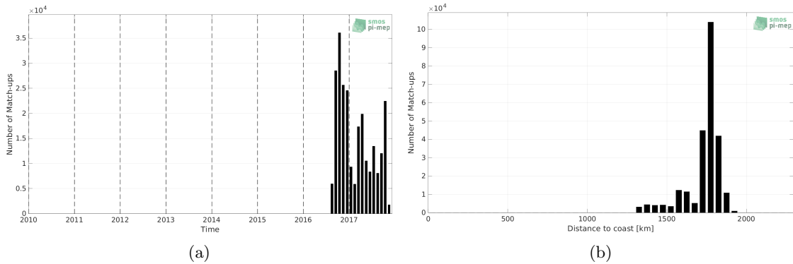
Figure 1: Number of match-ups between Waveglider (SPURS 2) and CCI SSS L4 Merged-OI v3.2 - 7-day running (ESA) SSS as a function of time (a) and as function of the distance to coast (b) over the SPURS 2 Pi-MEP region and for the full satellite product period.
