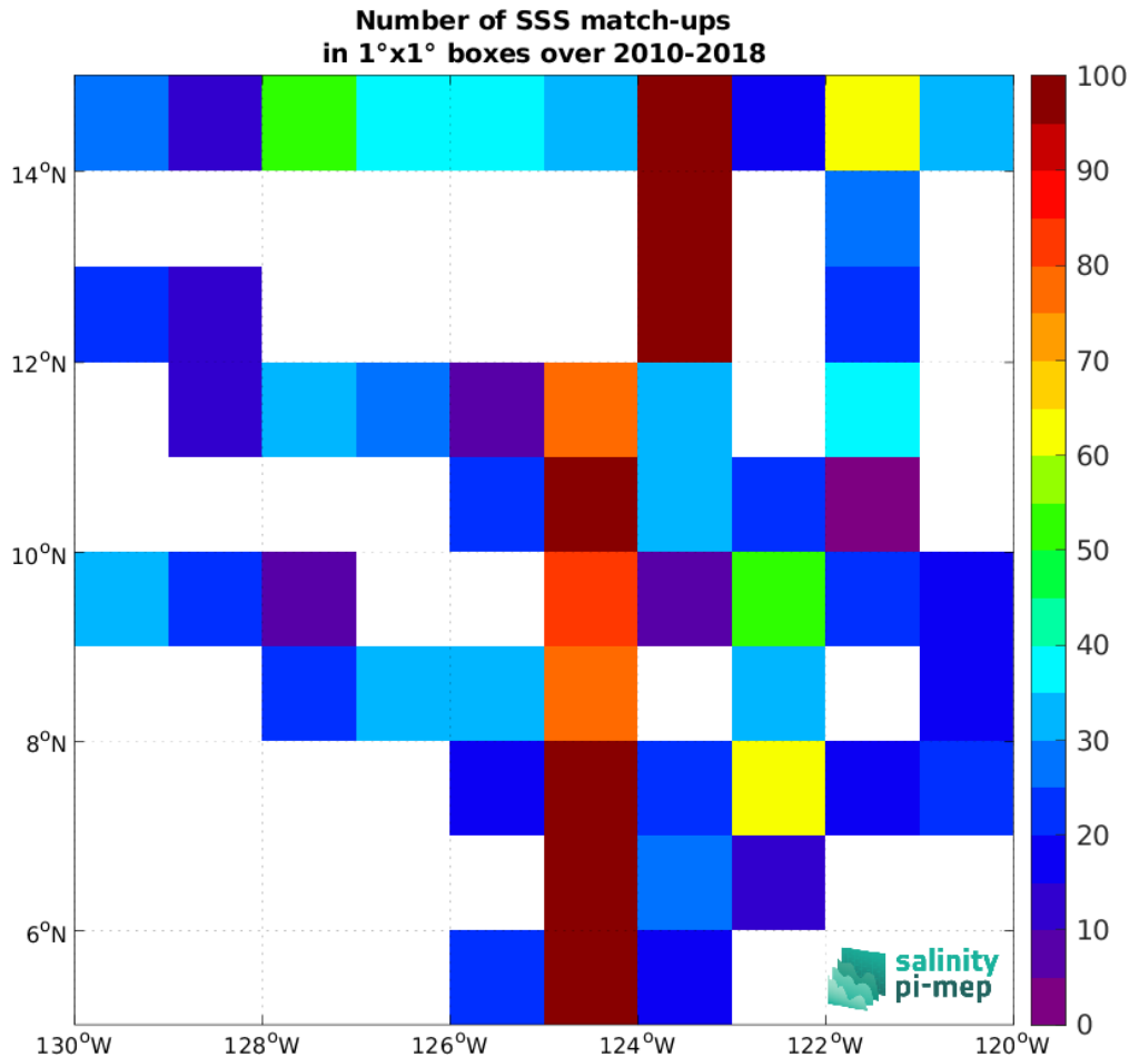
Figure 4: Number of SSS match-ups between TSG (SAMOS) SSS and the CCI SSS L4 Merged-OI v3.2 - 7-day running (ESA) SSS product for the SPURS 2 Pi-MEP region over 1^\circ \times 1^\circ boxes and for the full satellite product period.
