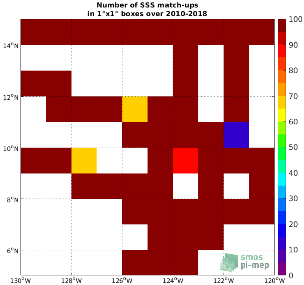
Figure 4: Number of SSS match-ups between TSG (SAMOS) SSS and the CCI SSS L4 Merged-OI v3.2 - 7-day running (ESA) SSS product for the SPURS 2 Pi-MEP region over 1°x1° boxes and for the full satellite product period.
