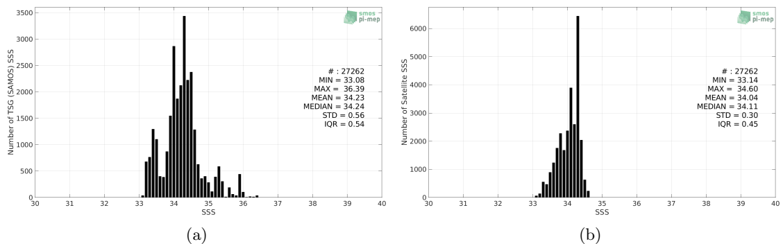
Figure 2: Histograms of SSS from TSG (SAMOS) (a) and CCI SSS L4 Merged-OI v3.2 - 7-day running (ESA) (b) considering all match-up pairs per bins of 0.1 over the SPURS 2 Pi-MEP region and for the full satellite product period.
