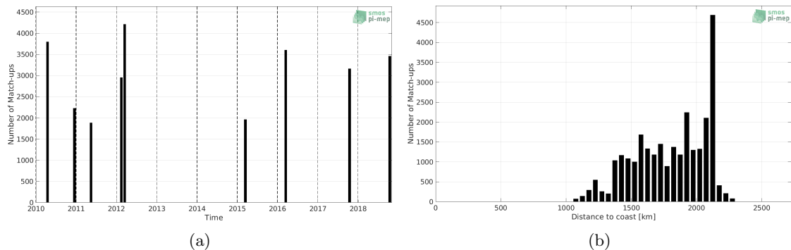
Figure 1: Number of match-ups between TSG (SAMOS) and CCI SSS L4 Merged-OI v3.2 - 7-day running (ESA) SSS as a function of time (a) and as function of the distance to coast (b) over the SPURS 2 Pi-MEP region and for the full satellite product period.
