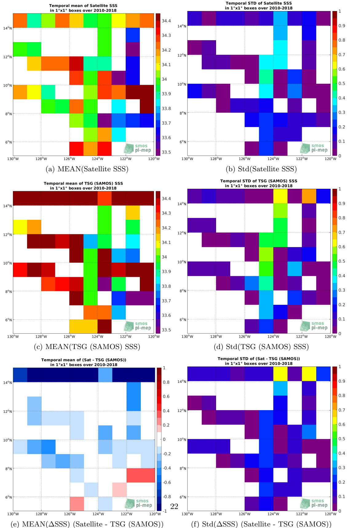
Figure 6: Temporal mean (left) and Std (right) of SSS from CCI SSS L4 Merged-OI v3.2 - 7-day running (ESA) (top), TSG (SAMOS) (middle), and of \Delta SSS (Satellite - TSG (SAMOS)). Only match-up pairs are used to generate these maps.
