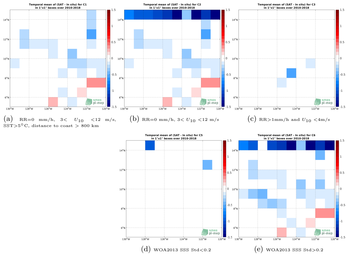
Figure 12: Temporal mean gridded over spatial boxes of size 1^\circ \times 1^\circ of \Delta SSS (CCI SSS L4 Merged-OI v3.2 - 7-day running (ESA) - TSG (SAMOS)) for 5 different subdatasets corresponding to:RR=0 mm/h, 3 < U_{10} < 12 m/s, SST >5^\circ\text{C} , distance to coast > 800 km (a), RR=0 mm/h, 3 < U_{10} < 12 m/s (b), RR >1 mm/h and U_{10} < 4 m/s (c), WOA2013 SSS Std <0.2 (d), WOA2013 SSS Std >0.2 (e).
