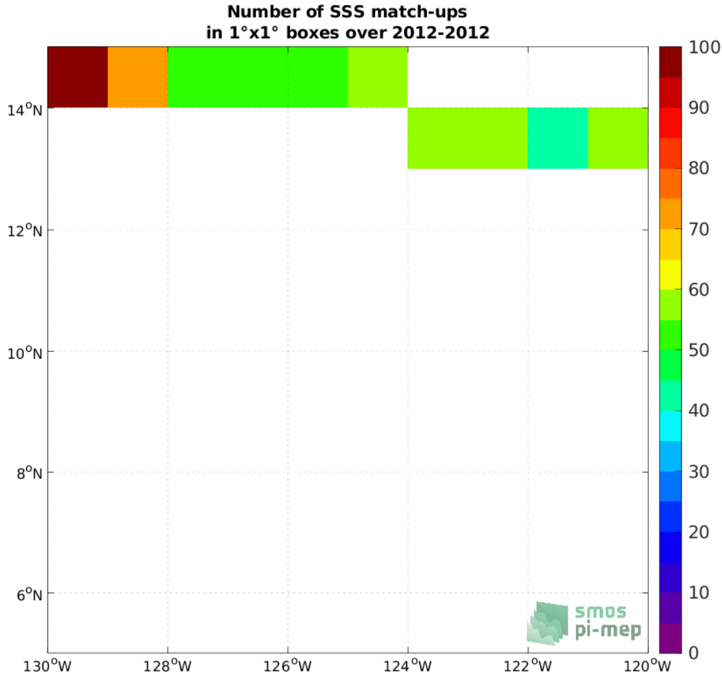
Figure 4: Number of SSS match-ups between TSG (GOSUD-Research-vessel) SSS and the CCI SSS L4 Merged-OI v3.2 - 7-day running (ESA) SSS product for the SPURS 2 Pi-MEP region over 1^\circ \times 1^\circ boxes and for the full satellite product period.
