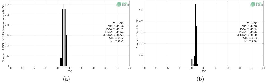
Figure 2: Histograms of SSS from TSG (GOSUD-Research-vessel) (a) and CCI SSS L4 Merged-OI v3.2 - 7-day running (ESA) (b) considering all match-up pairs per bins of 0.1 over the SPURS 2 Pi-MEP region and for the full satellite product period.
