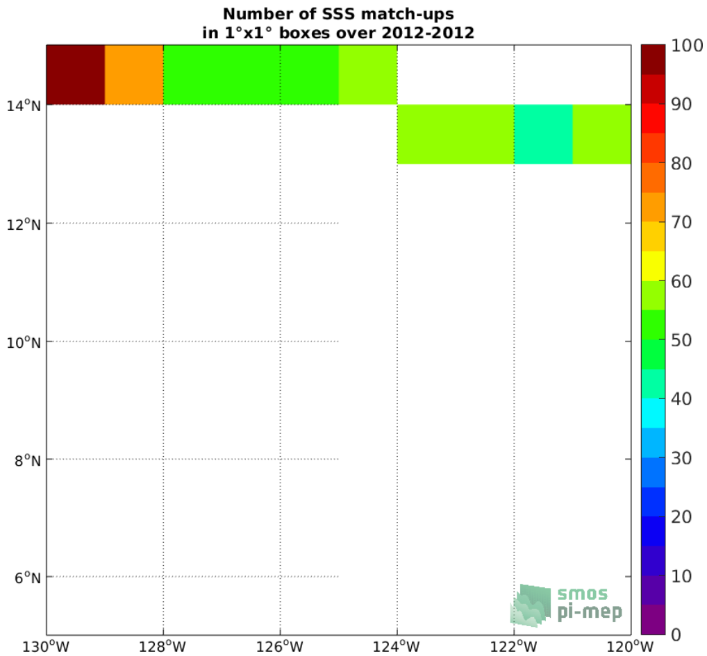
Figure 4: Number of SSS match-ups between TSG (GOSUD-Research-vessel) SSS and the CCI SSS L4 Merged-OI v3.2 - 7-day running (ESA) SSS product for the SPURS 2 Pi-MEP region over 1°×1° boxes and for the full satellite product period.
