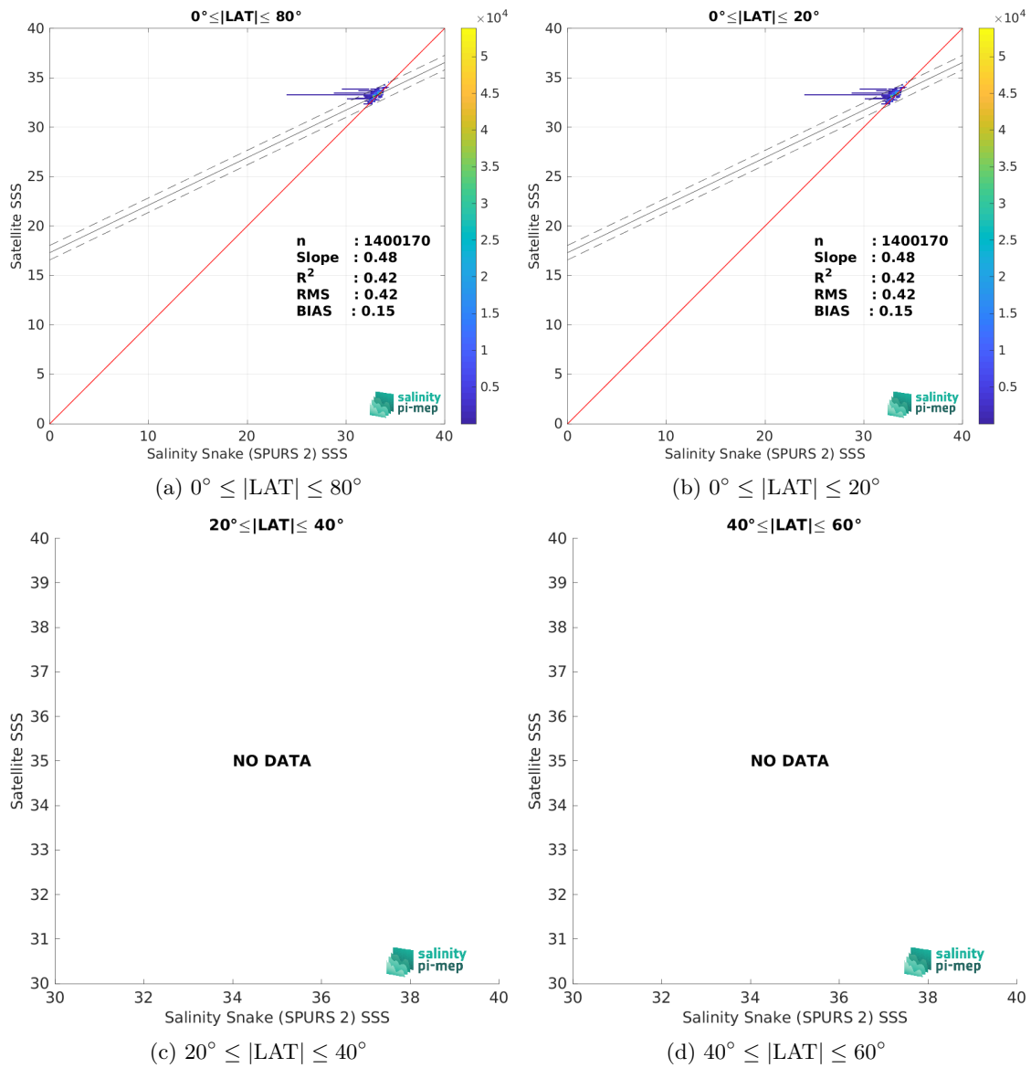
Figure 9: Contour maps of the concentration of CCI SSS L4 Merged-OI v3.2 - 7-day running (ESA) SSS (y-axis) versus Salinity Snake (SPURS 2) SSS (x-axis) at match-up pairs for different latitude bands. For each plot, the red line shows x=y . The black thin and dashed lines indicate a linear fit through the data cloud and the \pm 95\% confidence levels, respectively. The number of match-up pairs n , the slope and R^2 coefficient of the linear fit, the root mean square (RMS) and the mean bias between satellite and in situ data are indicated for each latitude band in each plot.
