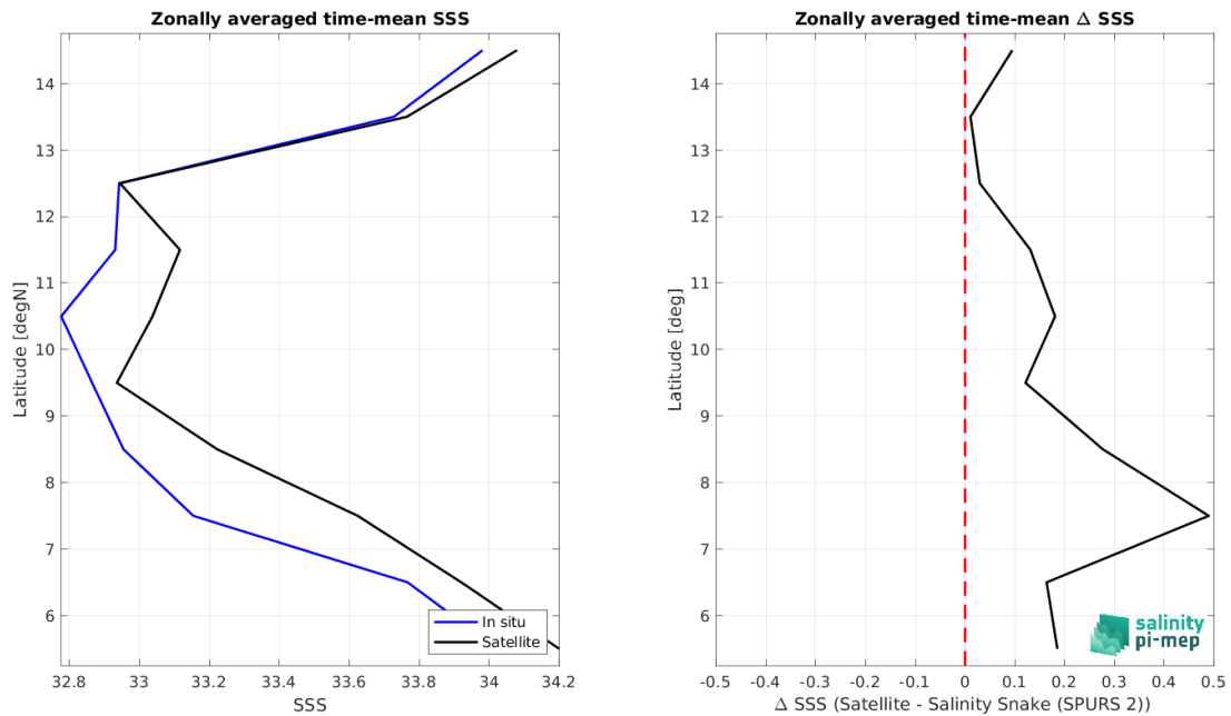
Figure 8: Left panel: Zonal mean SSS from CCI SSS L4 Merged-OI v3.2 - 7-day running (ESA) satellite product (black) and from Salinity Snake (SPURS 2) (blue). Right panel: Zonal mean of \Delta SSS (Satellite - Salinity Snake (SPURS 2)) for all the collected Pi-MEP match-up pairs estimated over the full satellite product period.
