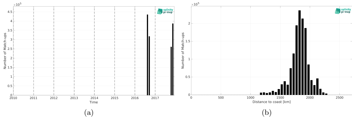
Figure 1: Number of match-ups between Salinity Snake (SPURS 2) and CCI SSS L4 Merged-OI v3.2 - 7-day running (ESA) SSS as a function of time (a) and as function of the distance to coast (b) over the SPURS 2 Pi-MEP region and for the full satellite product period.
