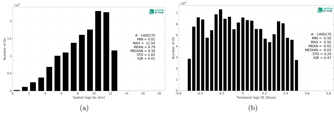
Figure 5: Histograms of the spatial (a) and temporal (b) lags between the location/time of the Salinity Snake (SPURS 2) measurement and the date of the corresponding CCI SSS L4 Merged-OI v3.2 - 7-day running (ESA) SSS pixel.
