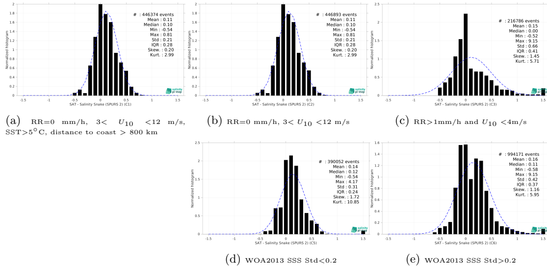
Figure 13: Normalized histogram of \Delta SSS (CCI SSS L4 Merged-OI v3.2 - 7-day running (ESA) - Salinity Snake (SPURS 2)) for 5 different subdatasets corresponding to: RR=0 mm/h, 3 < U_{10} < 12 m/s, SST>5°C, distance to coast > 800 km (a), RR=0 mm/h, 3 < U_{10} < 12 m/s (b), RR>1mm/h and U_{10} < 4 m/s (c), WOA2013 SSS Std<0.2 (d), WOA2013 SSS Std>0.2 (e).
