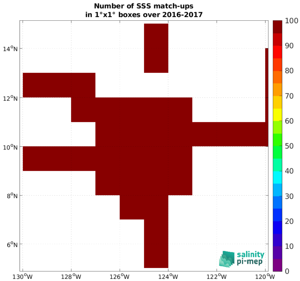
Figure 4: Number of SSS match-ups between Salinity Snake (SPURS 2) SSS and the CCI SSS L4 Merged-OI v3.2 - 7-day running (ESA) SSS product for the SPURS 2 Pi-MEP region over 1^\circ \times 1^\circ boxes and for the full satellite product period.
