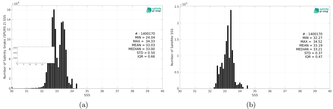
Figure 2: Histograms of SSS from Salinity Snake (SPURS 2) (a) and CCI SSS L4 Merged-OI v3.2 - 7-day running (ESA) (b) considering all match-up pairs per bins of 0.1 over the SPURS 2 Pi-MEP region and for the full satellite product period.
