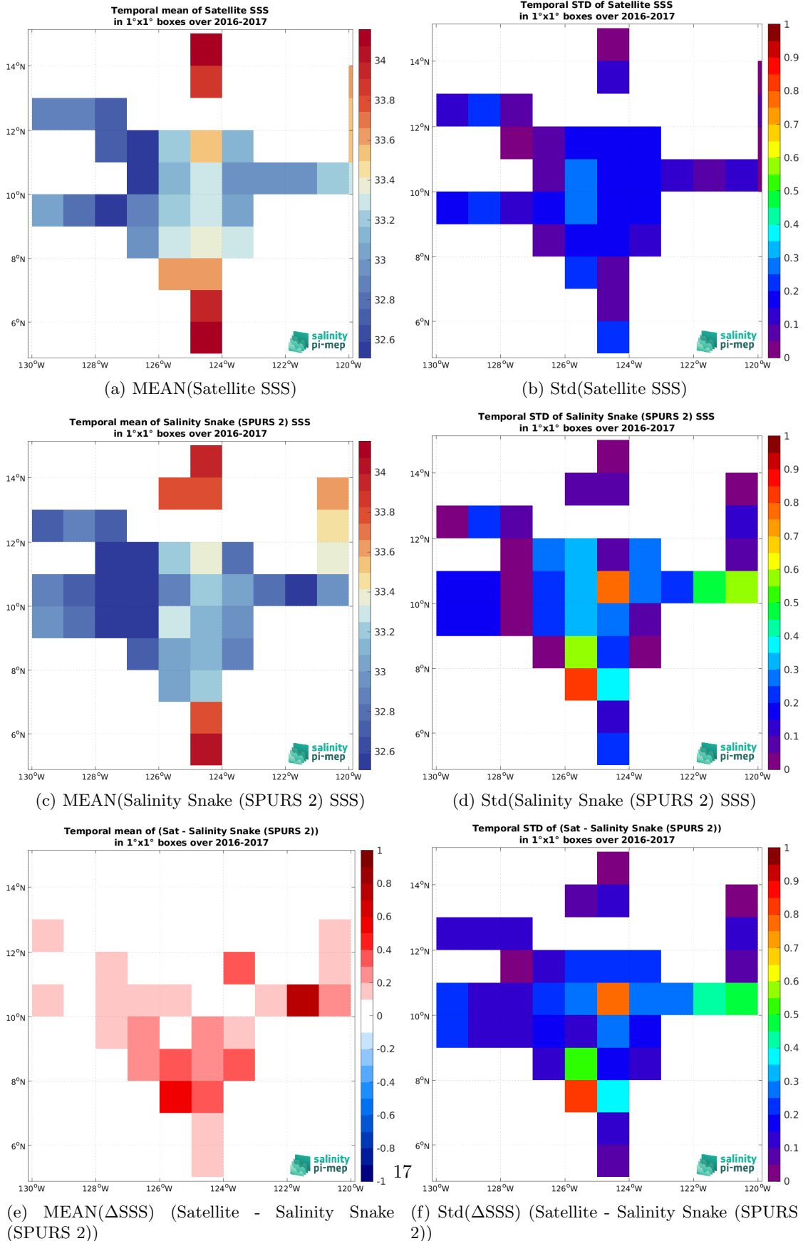
Figure 6: Temporal mean (left) and Std (right) of SSS from CCI SSS L4 Merged-OI v3.2 - 7-day running (ESA) (top), Salinity Snake (SPURS 2) (middle), and of \Delta SSS (Satellite - Salinity Snake (SPURS 2)). Only match-up pairs are used to generate these maps.
