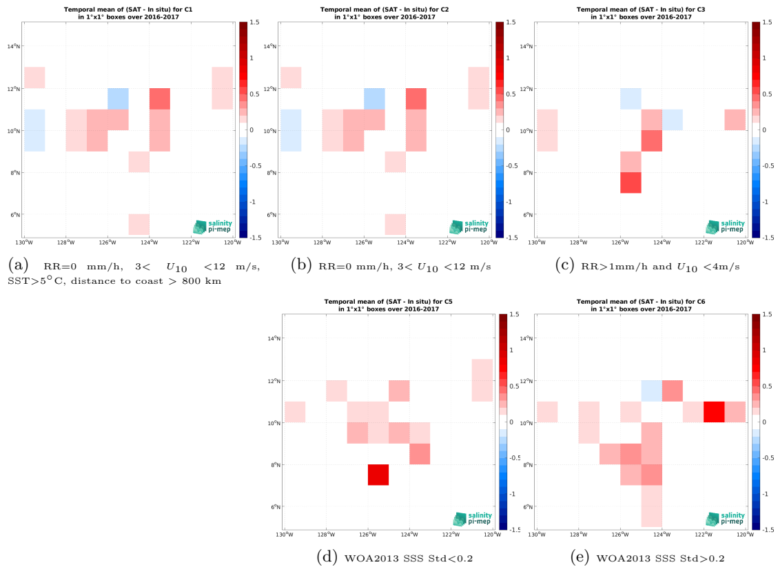
Figure 12: Temporal mean gridded over spatial boxes of size 1^\circ \times 1^\circ of \Delta SSS (CCI SSS L4 Merged-OI v3.2 - 7-day running (ESA) - Salinity Snake (SPURS 2)) for 5 different subdatasets corresponding to: RR=0 mm/h, 3 < U_{10} < 12 m/s, SST > 5°C, distance to coast > 800 km (a), RR=0 mm/h, 3 < U_{10} < 12 m/s (b), RR > 1mm/h and U_{10} < 4 m/s (c), WOA2013 SSS Std < 0.2 (d), WOA2013 SSS Std > 0.2 (e).
