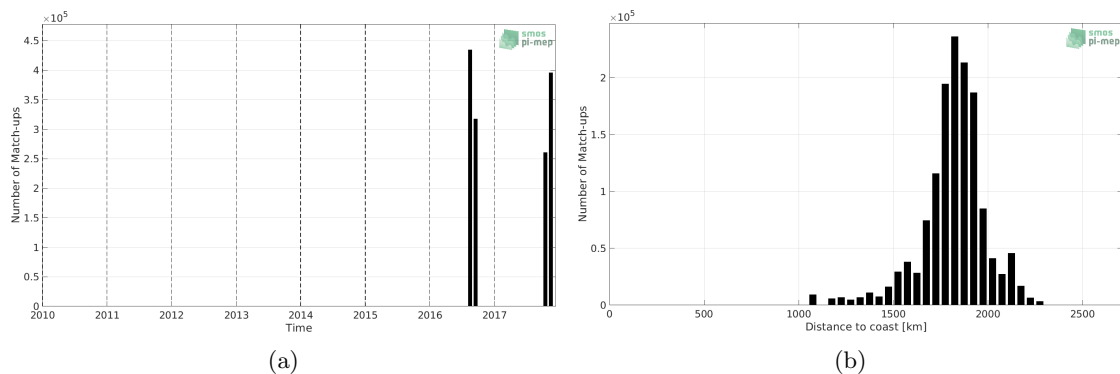
Figure 1: Number of match-ups between Salinity Snake and CCI SSS L4 Merged-OI v3.2 - 7-day running (ESA) SSS as a function of time (a) and as function of the distance to coast (b) over the SPURS 2 Pi-MEP region and for the full satellite product period.
