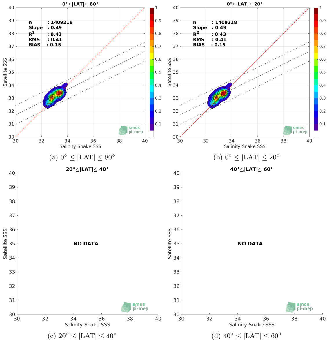
Figure 8: Contour maps of the concentration of CCI SSS L4 Merged-OI v3.2 - 7-day running (ESA) SSS (y-axis) versus Salinity Snake SSS (x-axis) at match-up pairs for different latitude bands. For each plot, the red line shows x=y . The black thin and dashed lines indicate a linear fit through the data cloud and the \pm 95\% confidence levels, respectively. The number match-up pairs n , the slope and R^2 coefficient of the linear fit, the root mean square (RMS) and the mean bias between satellite and in situ data are indicated for each latitude band in each plots.
