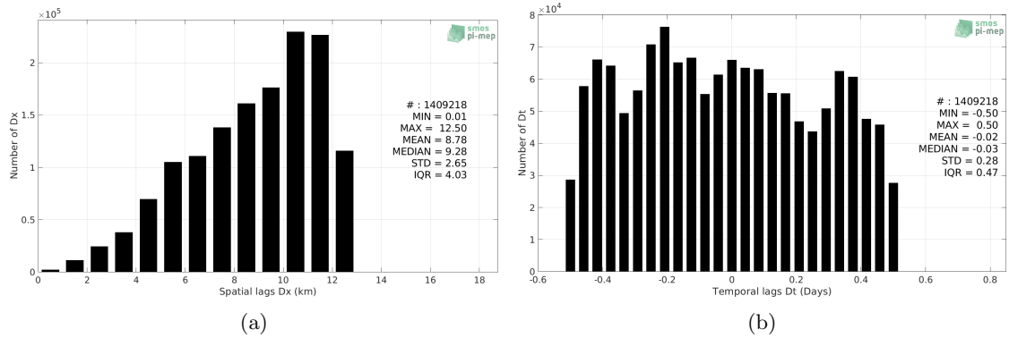
Figure 4: Histograms of the spatial (a) and temporal (b) lags between the location/time of the Salinity Snake measurement and the date of the corresponding CCI SSS L4 Merged-OI v3.2 - 7-day running (ESA) SSS pixel.
