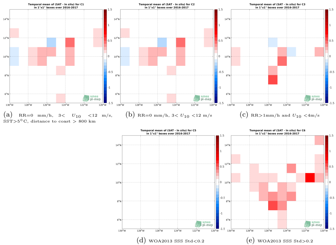
Figure 11: Temporal mean gridded over spatial boxes of size 1^\circ \times 1^\circ of \Delta SSS (CCI SSS L4 Merged-OI v3.2 - 7-day running (ESA) - Salinity Snake) for 5 different subdatasets corresponding to:RR=0 mm/h, 3 < U_{10} < 12 m/s, SST >5^\circ C, distance to coast > 800 km (a), RR=0 mm/h, 3 < U_{10} < 12 m/s (b), RR >1 mm/h and U_{10} < 4 m/s (c), WOA2013 SSS Std <0.2 (d), WOA2013 SSS Std >0.2 (e).
