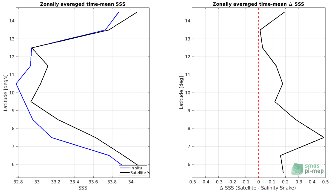
Figure 7: Left panel: Zonal mean SSS from CCI SSS L4 Merged-OI v3.2 - 7-day running (ESA) satellite product (black) and from Salinity Snake (blue). Right panel: Zonal mean of \Delta SSS (Satellite - Salinity Snake) for all the collected Pi-MEP match-up pairs estimated over the full satellite product period.
