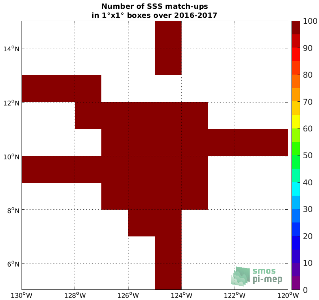
Figure 3: Number of SSS match-ups between Salinity Snake SSS and the CCI SSS L4 Merged-OI v3.2 - 7-day running (ESA) SSS product for the SPURS 2 Pi-MEP region over 1°×1° boxes and for the full satellite product period.
