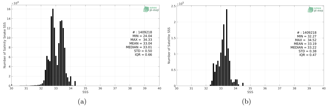
Figure 2: Histograms of SSS from Salinity Snake (a) and CCI SSS L4 Merged-OI v3.2 - 7-day running (ESA) (b) considering all match-up pairs per bins of 0.1 over the SPURS 2 Pi-MEP region and for the full satellite product period.
