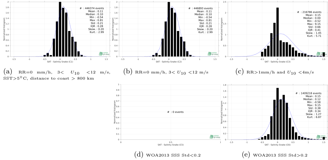
Figure 12: Normalized histogram of \Delta SSS (CCI SSS L4 Merged-OI v3.2 - 7-day running (ESA) - Salinity Snake) for 5 different subdatasets corresponding to: RR=0 mm/h, 3 < U_{10} < 12 m/s, SST > 5°C, distance to coast > 800 km (a), RR=0 mm/h, 3 < U_{10} < 12 m/s (b), RR > 1mm/h and U_{10} < 4 m/s (c), WOA2013 SSS Std < 0.2 (d), WOA2013 SSS Std > 0.2 (e).
