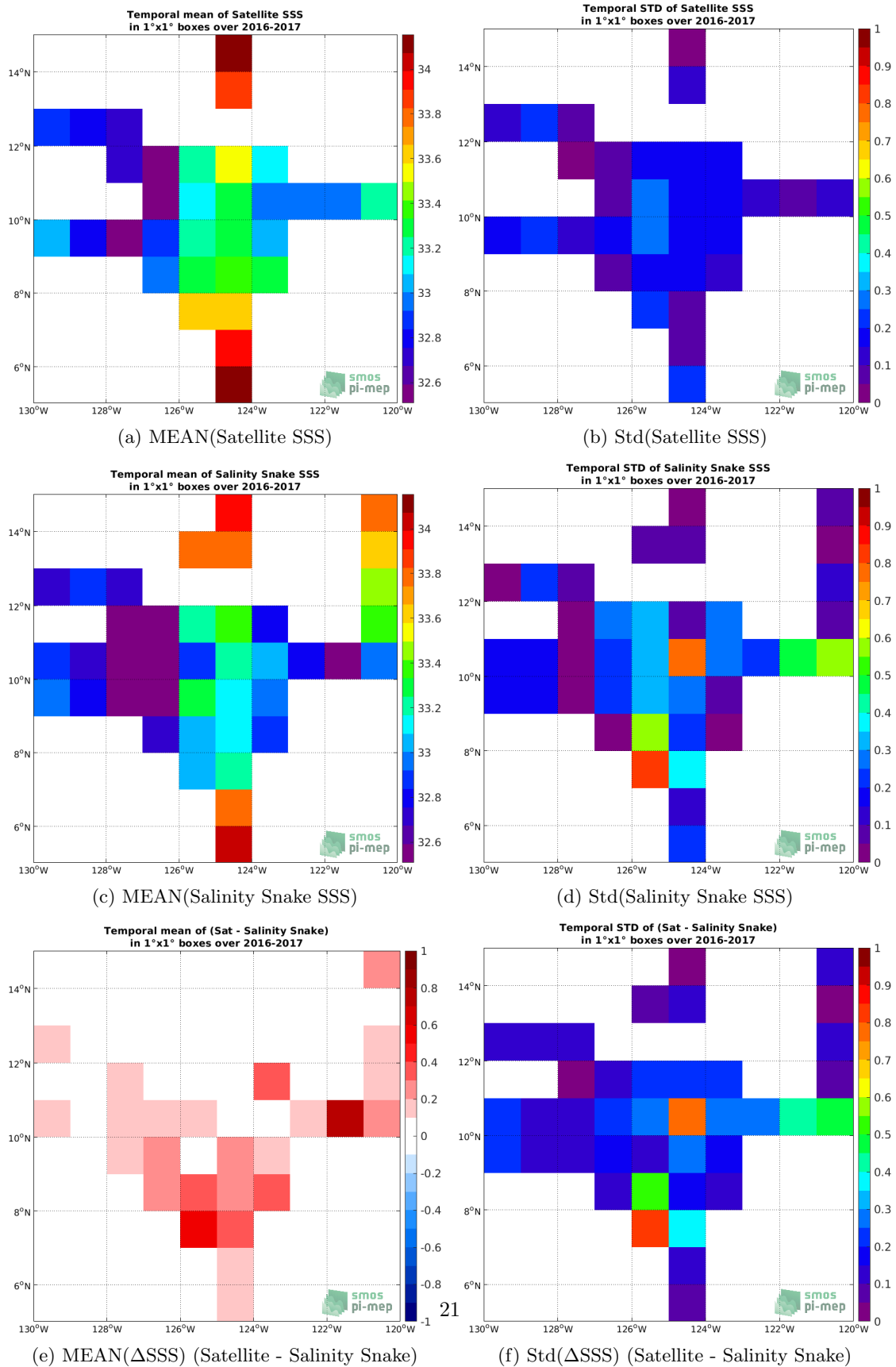
Figure 5: Temporal mean (left) and Std (right) of SSS from CCI SSS L4 Merged-OI v3.2 - 7-day running (ESA) (top), Salinity Snake (middle), and of \Delta SSS (Satellite - Salinity Snake). Only match-up pairs are used to generate these maps.
