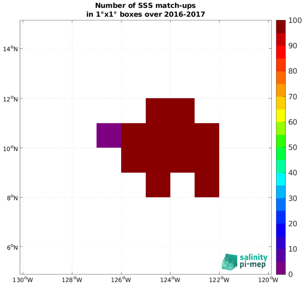
Figure 4: Number of SSS match-ups between Seaglider (SPURS 2) SSS and the CCI SSS L4 Merged-OI v3.2 - 7-day running (ESA) SSS product for the SPURS 2 Pi-MEP region over 1^\circ \times 1^\circ boxes and for the full satellite product period.
