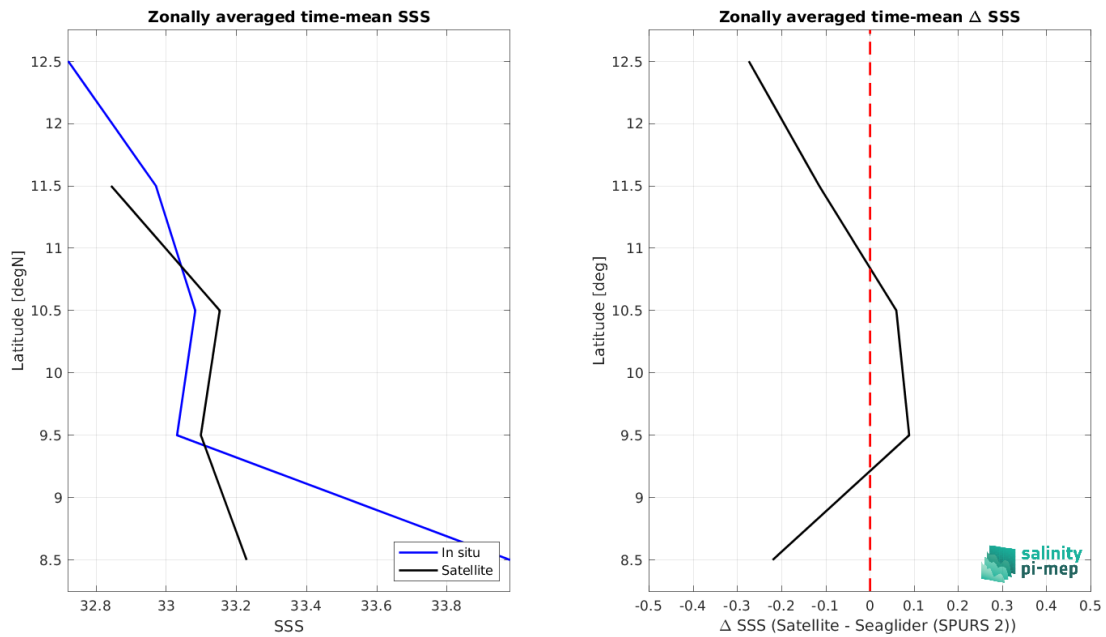
Figure 8: Left panel: Zonal mean SSS from CCI SSS L4 Merged-OI v3.2 - 7-day running (ESA) satellite product (black) and from Seaglider (SPURS 2) (blue). Right panel: Zonal mean of \Delta SSS (Satellite - Seaglider (SPURS 2)) for all the collected Pi-MEP match-up pairs estimated over the full satellite product period.
