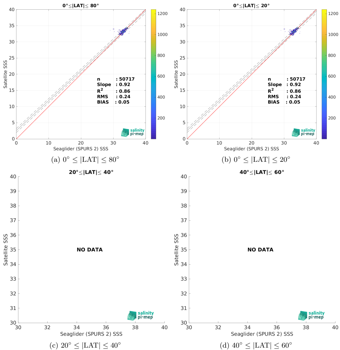
Figure 9: Contour maps of the concentration of CCI SSS L4 Merged-OI v3.2 - 7-day running (ESA) SSS (y-axis) versus Seaglider (SPURS 2) SSS (x-axis) at match-up pairs for different latitude bands. For each plot, the red line shows x=y . The black thin and dashed lines indicate a linear fit through the data cloud and the \pm 95\% confidence levels, respectively. The number match-up pairs n , the slope and R^2 coefficient of the linear fit, the root mean square (RMS) and the mean bias between satellite and in situ data are indicated for each latitude band in each plots.
