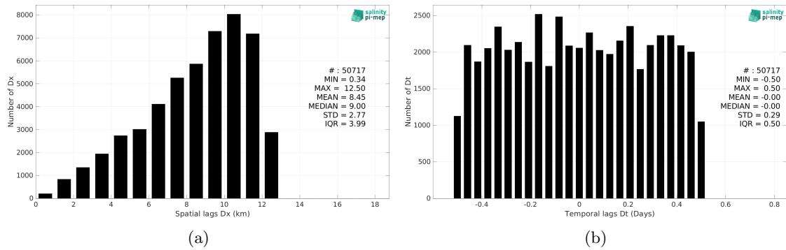
Figure 5: Histograms of the spatial (a) and temporal (b) lags between the location/time of the Seaglider (SPURS 2) measurement and the date of the corresponding CCI SSS L4 Merged-OI v3.2 - 7-day running (ESA) SSS pixel.
