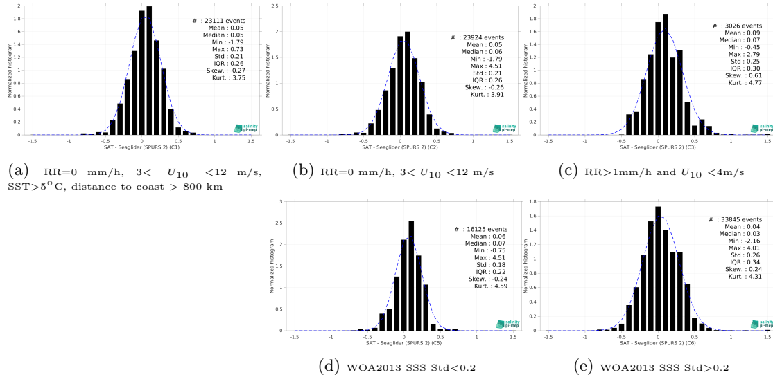
Figure 13: Normalized histogram of \Delta\text{SSS} (CCI SSS L4 Merged-OI v3.2 - 7-day running (ESA) - Seaglider (SPURS 2)) for 5 different subdatasets corresponding to: RR=0 mm/h, 3 < U_{10} < 12 m/s, SST>5°C, distance to coast > 800 km (a), RR=0 mm/h, 3 < U_{10} < 12 m/s (b), RR>1mm/h and U_{10} < 4 m/s (c), WOA2013 SSS Std<0.2 (d), WOA2013 SSS Std>0.2 (e).
