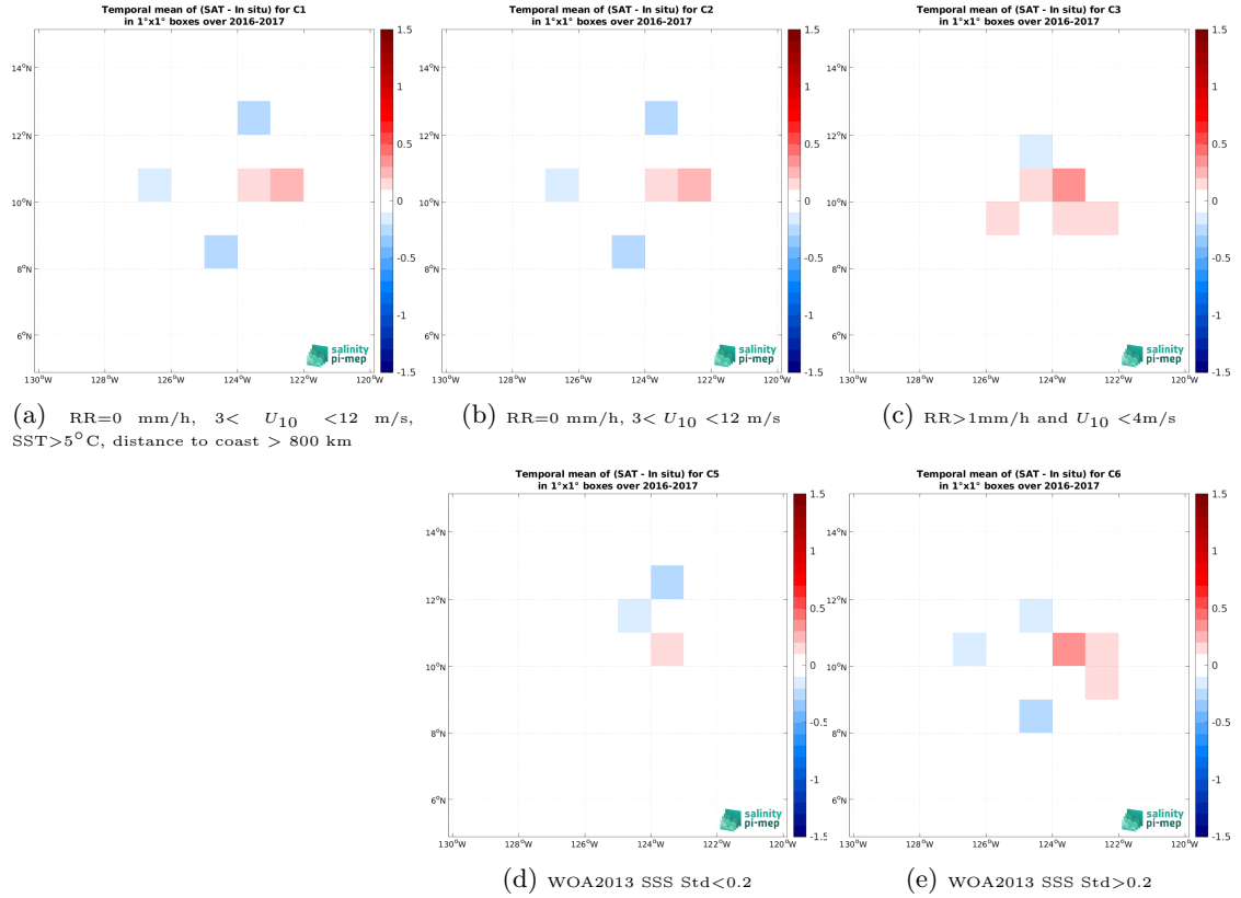
Figure 12: Temporal mean gridded over spatial boxes of size 1^{\circ}\times 1^{\circ} of \Delta\text{SSS} (CCI SSS L4 Merged-OI v3.2 - 7-day running (ESA) - Seaglider (SPURS 2)) for 5 different subdatasets corresponding to:RR=0 mm/h, 3 < U_{10} < 12 m/s, SST > 5^{\circ}\text{C} , distance to coast > 800 km (a), RR=0 mm/h, 3 < U_{10} < 12 m/s (b), RR > 1 mm/h and U_{10} < 4 m/s (c), WOA2013 SSS Std < 0.2 (d), WOA2013 SSS Std > 0.2 (e).
