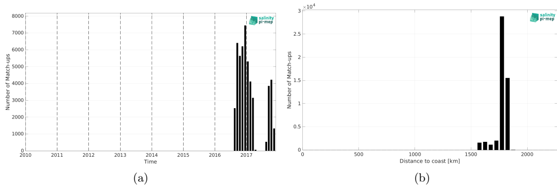
Figure 1: Number of match-ups between Seaglider (SPURS 2) and CCI SSS L4 Merged-OI v3.2 - 7-day running (ESA) SSS as a function of time (a) and as function of the distance to coast (b) over the SPURS 2 Pi-MEP region and for the full satellite product period.
