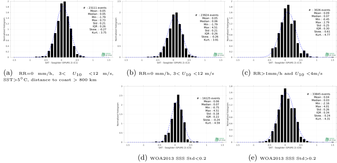
Figure 13: Normalized histogram of \Delta SSS (CCI SSS L4 Merged-OI v3.2 - 7-day running (ESA) - Seaglider (SPURS 2)) for 5 different subdatasets corresponding to: RR=0 mm/h, 3 < U_{10} < 12 m/s, SST>5°C, distance to coast > 800 km (a), RR=0 mm/h, 3 < U_{10} < 12 m/s (b), RR>1mm/h and U_{10} < 4 m/s (c), WOA2013 SSS Std<0.2 (d), WOA2013 SSS Std>0.2 (e).
