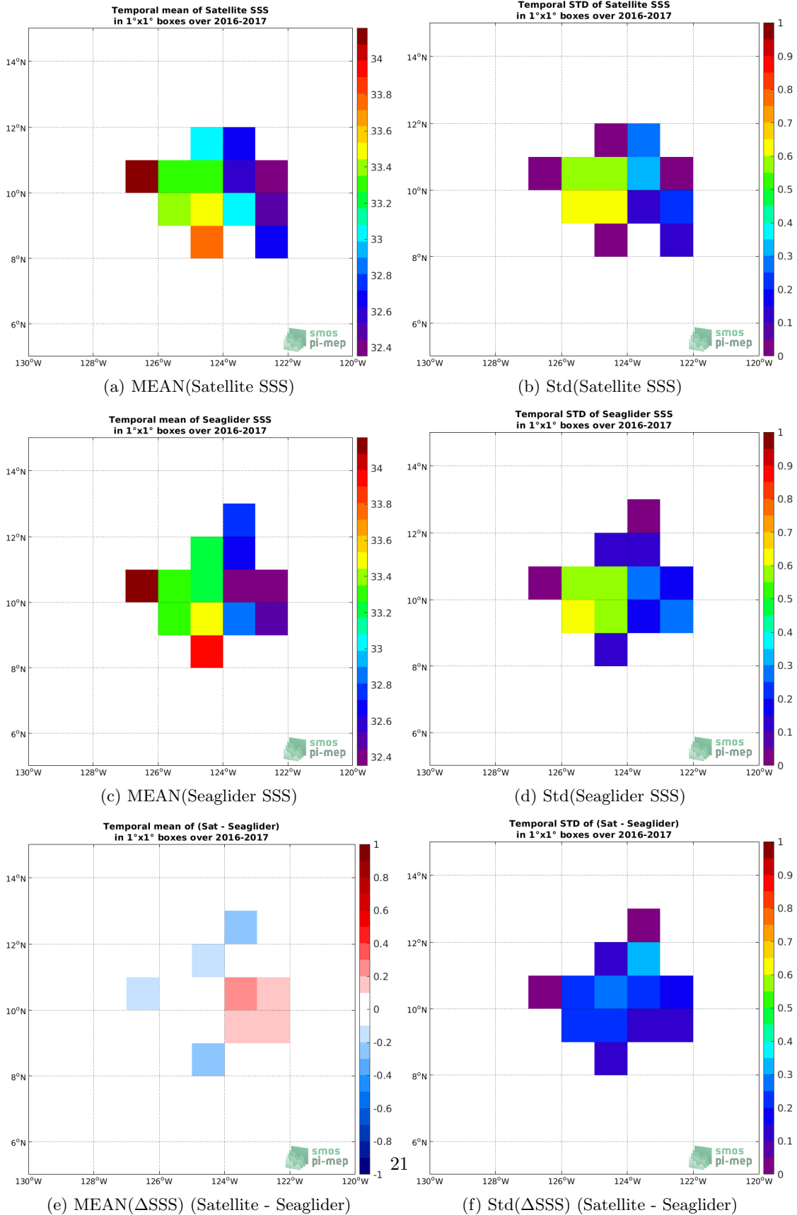
Figure 5: Temporal mean (left) and Std (right) of SSS from CCI SSS L4 Merged-OI v3.2 - 7-day running (ESA) (top), Seaglider (middle), and of \Delta SSS (Satellite - Seaglider). Only match-up pairs are used to generate these maps.
