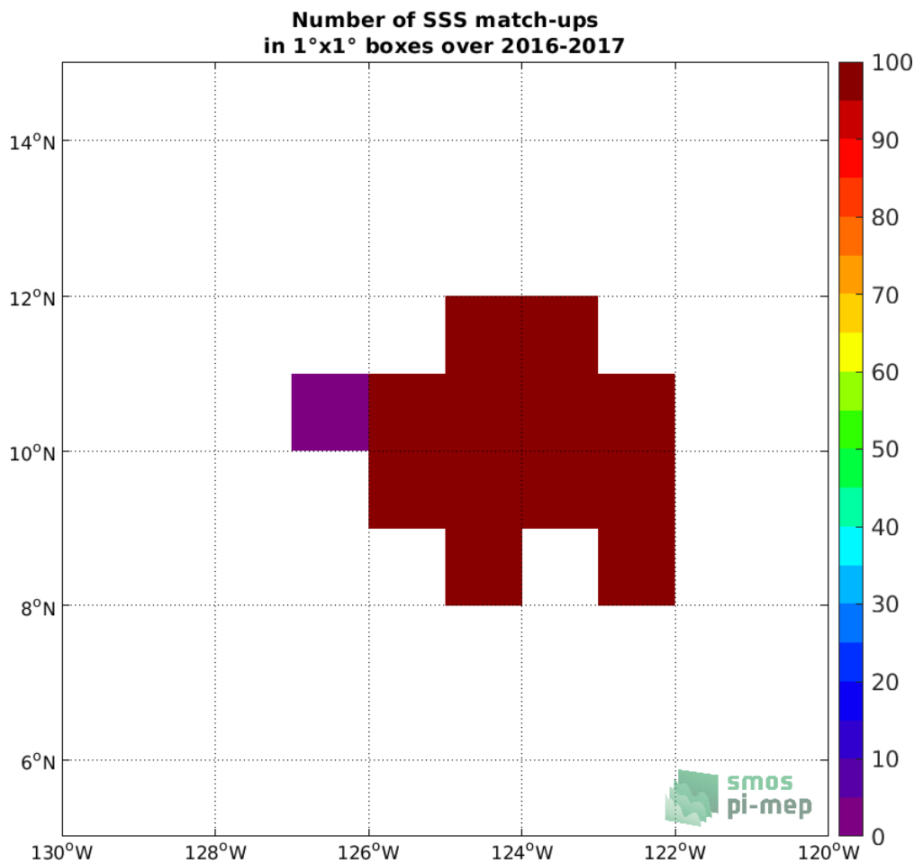
Figure 3: Number of SSS match-ups between Seaglider SSS and the CCI SSS L4 Merged-OI v3.2 - 7-day running (ESA) SSS product for the SPURS 2 Pi-MEP region over 1°×1° boxes and for the full satellite product period.
