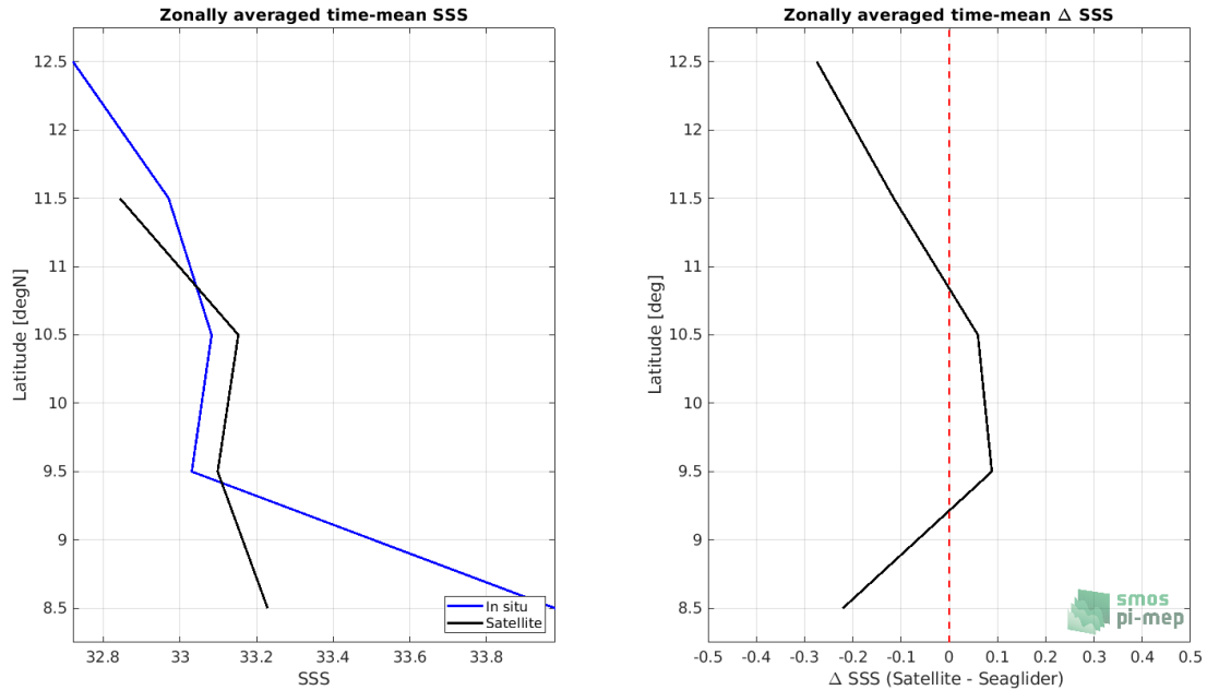
Figure 7: Left panel: Zonal mean SSS from CCI SSS L4 Merged-OI v3.2 - 7-day running (ESA) satellite product (black) and from Seaglider (blue). Right panel: Zonal mean of \Delta SSS (Satellite - Seaglider) for all the collected Pi-MEP match-up pairs estimated over the full satellite product period.
