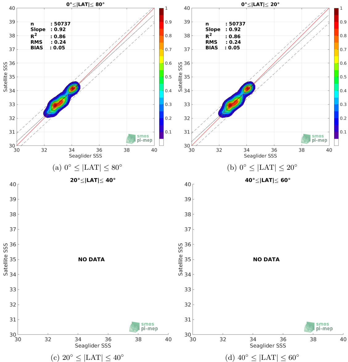
Figure 8: Contour maps of the concentration of CCI SSS L4 Merged-OI v3.2 - 7-day running (ESA) SSS (y-axis) versus Seaglider SSS (x-axis) at match-up pairs for different latitude bands. For each plot, the red line shows x=y . The black thin and dashed lines indicate a linear fit through the data cloud and the \pm 95\% confidence levels, respectively. The number match-up pairs n , the slope and R^2 coefficient of the linear fit, the root mean square (RMS) and the mean bias between satellite and in situ data are indicated for each latitude band in each plots.
