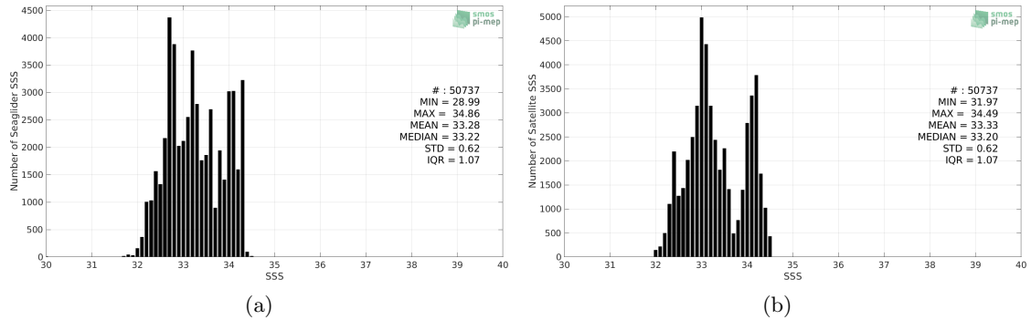
Figure 2: Histograms of SSS from Seaglider (a) and CCI SSS L4 Merged-OI v3.2 - 7-day running (ESA) (b) considering all match-up pairs per bins of 0.1 over the SPURS 2 Pi-MEP region and for the full satellite product period.
