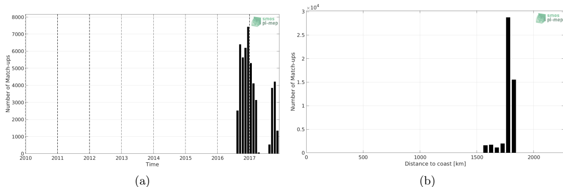
Figure 1: Number of match-ups between Seagliders and CCI SSS L4 Merged-OI v3.2 - 7-day running (ESA) SSS as a function of time (a) and as function of the distance to coast (b) over the SPURS 2 Pi-MEP region and for the full satellite product period.
