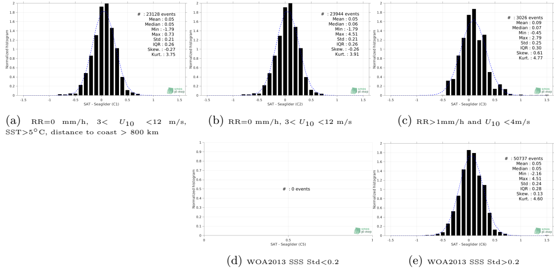
Figure 12: Normalized histogram of \Delta SSS (CCI SSS L4 Merged-OI v3.2 - 7-day running (ESA) - Seaglider) for 5 different subdatasets corresponding to: RR=0 mm/h, 3 < U_{10} < 12 m/s, SST>5°C, distance to coast > 800 km (a), RR=0 mm/h, 3 < U_{10} < 12 m/s (b), RR>1mm/h and U_{10} < 4 m/s (c), WOA2013 SSS Std<0.2 (d), WOA2013 SSS Std>0.2 (e).
