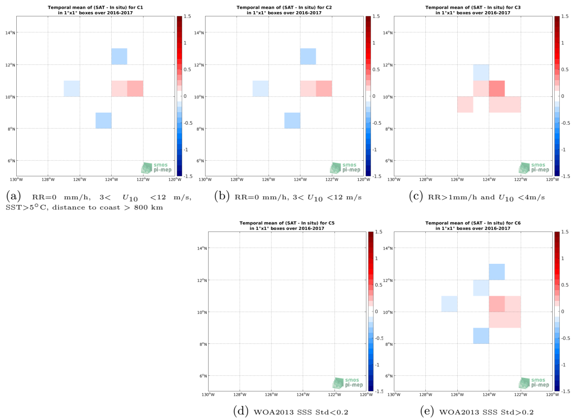
Figure 11: Temporal mean gridded over spatial boxes of size 1^\circ \times 1^\circ of \Delta SSS (CCI SSS L4 Merged-OI v3.2 - 7-day running (ESA) - Seaglider) for 5 different subdatasets corresponding to:RR=0 mm/h, 3 < U_{10} < 12 m/s, SST >5^\circ\text{C} , distance to coast > 800 km (a), RR=0 mm/h, 3 < U_{10} < 12 m/s (b), RR >1 mm/h and U_{10} < 4 m/s (c), WOA2013 SSS Std <0.2 (d), WOA2013 SSS Std >0.2 (e).
