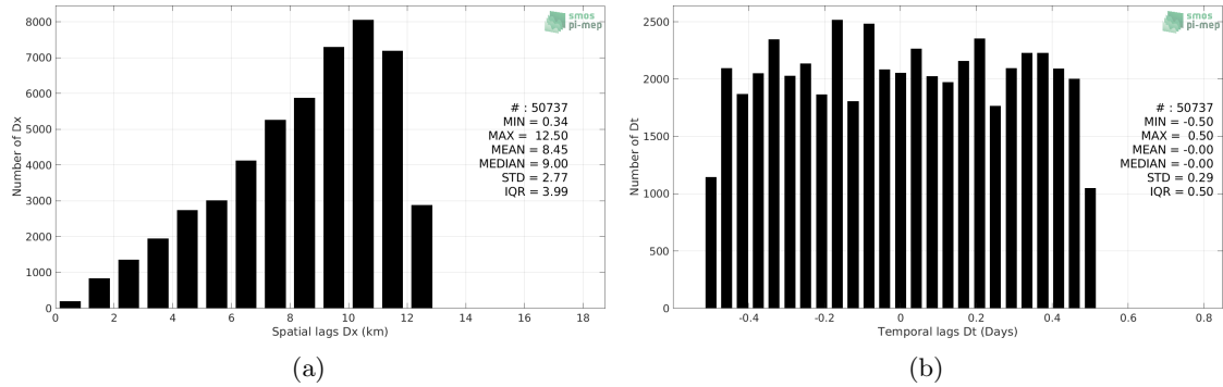
Figure 4: Histograms of the spatial (a) and temporal (b) lags between the location/time of the Seaglider measurement and the date of the corresponding CCI SSS L4 Merged-OI v3.2 - 7-day running (ESA) SSS pixel.
