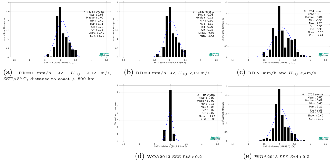
Figure 13: Normalized histogram of \Delta SSS (CCI SSS L4 Merged-OI v3.2 - 7-day running (ESA) - Saldrone (SPURS 2)) for 5 different subdatasets corresponding to: RR=0 mm/h, 3 < U_{10} < 12 m/s, SST > 5°C, distance to coast > 800 km (a), RR=0 mm/h, 3 < U_{10} < 12 m/s (b), RR > 1mm/h and U_{10} < 4 m/s (c), WOA2013 SSS Std < 0.2 (d), WOA2013 SSS Std > 0.2 (e).
