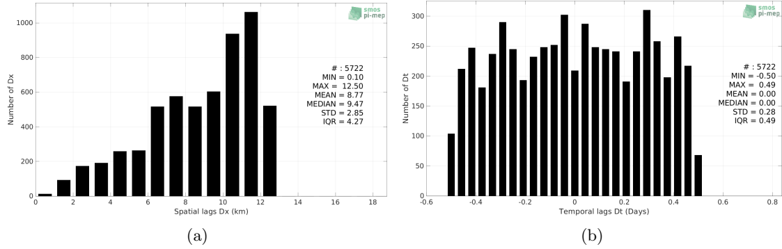
Figure 5: Histograms of the spatial (a) and temporal (b) lags between the location/time of the Saildrone (SPURS 2) measurement and the date of the corresponding CCI SSS L4 Merged-OI v3.2 - 7-day running (ESA) SSS pixel.
