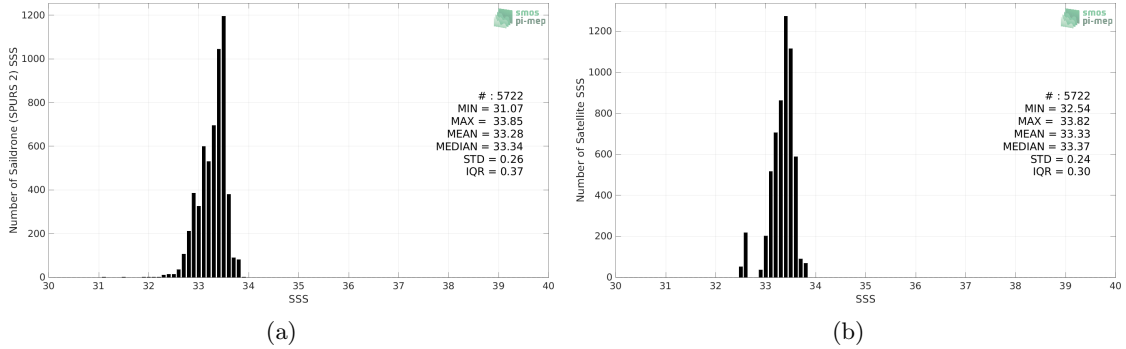
Figure 2: Histograms of SSS from Saildrone (SPURS 2) (a) and CCI SSS L4 Merged-OI v3.2 - 7-day running (ESA) (b) considering all match-up pairs per bins of 0.1 over the SPURS 2 Pi-MEP region and for the full satellite product period.
