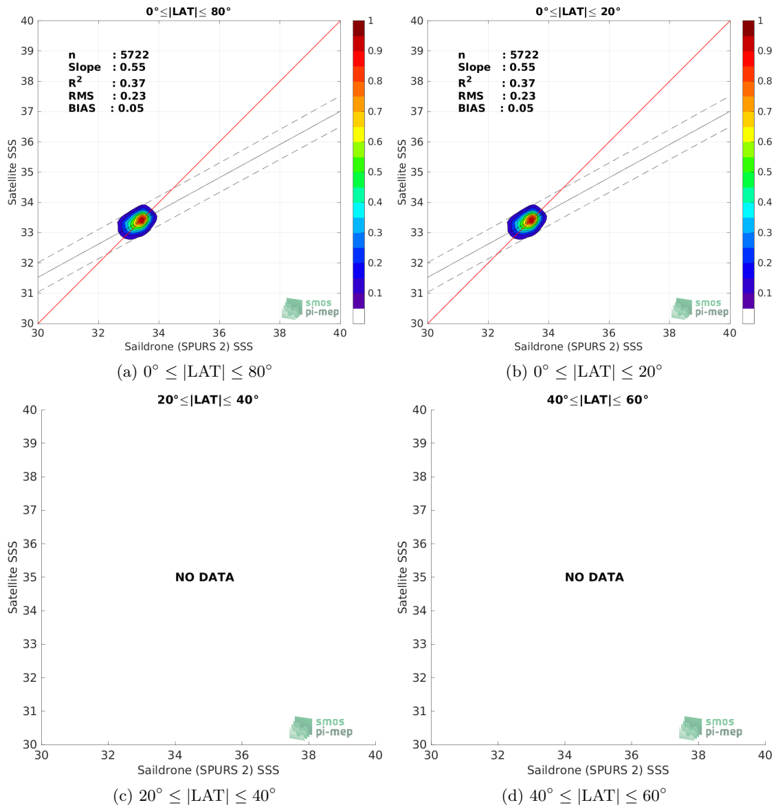
Figure 9: Contour maps of the concentration of CCI SSS L4 Merged-OI v3.2 - 7-day running (ESA) SSS (y-axis) versus Saildrone (SPURS 2) SSS (x-axis) at match-up pairs for different latitude bands. For each plot, the red line shows x=y . The black thin and dashed lines indicate a linear fit through the data cloud and the \pm 95\% confidence levels, respectively. The number match-up pairs n , the slope and R^2 coefficient of the linear fit, the root mean square (RMS) and the mean bias between satellite and in situ data are indicated for each latitude band in each plots.
