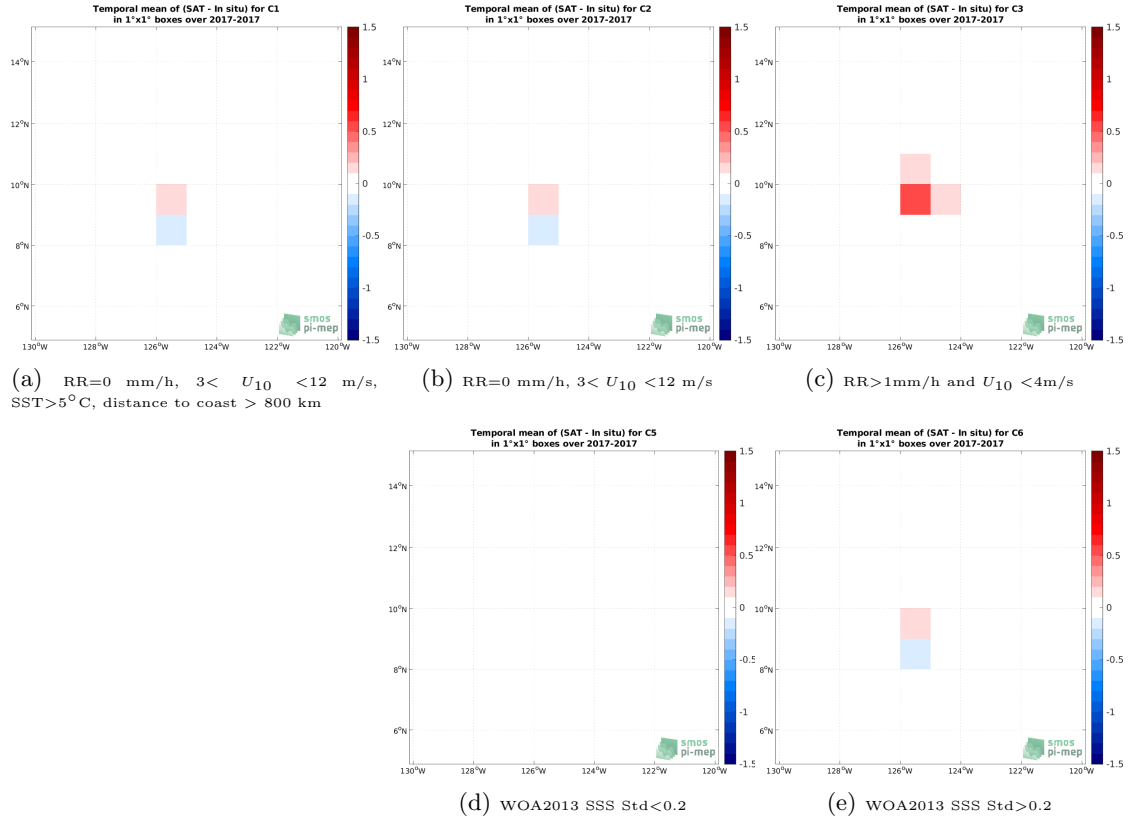
Figure 12: Temporal mean gridded over spatial boxes of size 1^{\circ}\times 1^{\circ} of \Delta\text{SSS} (CCI SSS L4 Merged-OI v3.2 - 7-day running (ESA) - Saildrone (SPURS 2)) for 5 different subdatasets corresponding to:RR=0 mm/h, 3 < U_{10} < 12 m/s, SST >5^{\circ}\text{C} , distance to coast > 800 km (a), RR=0 mm/h, 3 < U_{10} < 12 m/s (b), RR >1 mm/h and U_{10} < 4 m/s (c), WOA2013 SSS Std <0.2 (d), WOA2013 SSS Std >0.2 (e).
