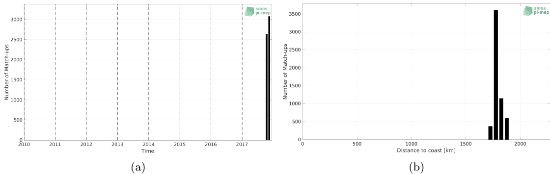
Figure 1: Number of match-ups between Saildrone (SPURS 2) and CCI SSS L4 Merged-OI v3.2 - 7-day running (ESA) SSS as a function of time (a) and as function of the distance to coast (b) over the SPURS 2 Pi-MEP region and for the full satellite product period.
