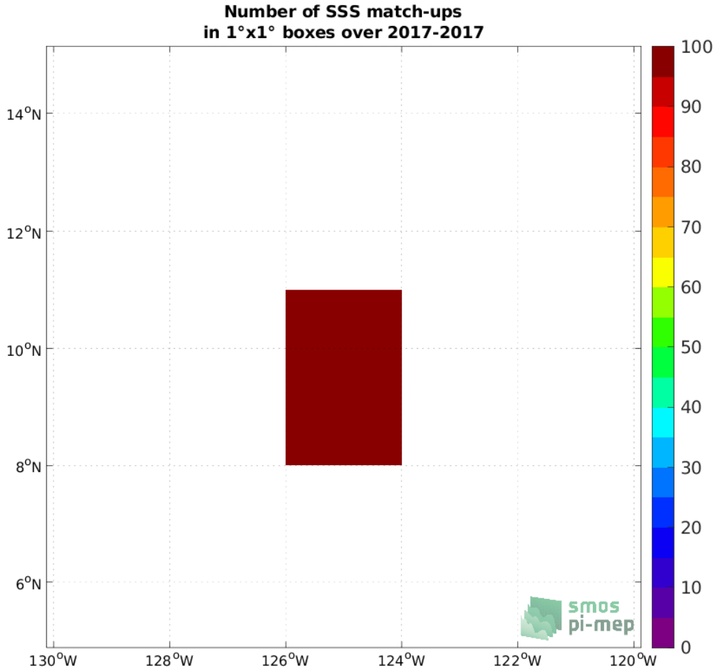
Figure 4: Number of SSS match-ups between Saildrone (SPURS 2) SSS and the CCI SSS L4 Merged-OI v3.2 - 7-day running (ESA) SSS product for the SPURS 2 Pi-MEP region over 1^\circ \times 1^\circ boxes and for the full satellite product period.
