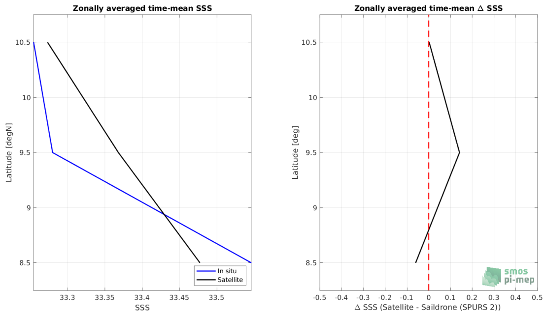
Figure 8: Left panel: Zonal mean SSS from CCI SSS L4 Merged-OI v3.2 - 7-day running (ESA) satellite product (black) and from Sairdron (SPURS 2) (blue). Right panel: Zonal mean of \Delta SSS (Satellite - Sairdron (SPURS 2)) for all the collected Pi-MEP match-up pairs estimated over the full satellite product period.
