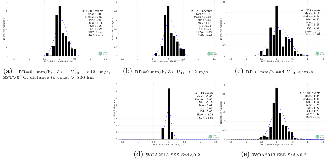
Figure 13: Normalized histogram of \Delta\text{SSS} (CCI SSS L4 Merged-OI v3.2 - 7-day running (ESA) - Saldrone (SPURS 2)) for 5 different subdatasets corresponding to: RR=0 mm/h, 3 < U_{10} < 12 m/s, SST > 5^{\circ}\text{C} , distance to coast > 800 km (a), RR=0 mm/h, 3 < U_{10} < 12 m/s (b), RR > 1\text{mm/h} and U_{10} < 4\text{m/s} (c), WOA2013 SSS Std < 0.2 (d), WOA2013 SSS Std > 0.2 (e).
