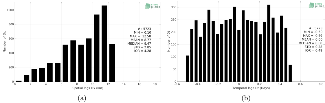
Figure 4: Histograms of the spatial (a) and temporal (b) lags between the location/time of the Saildrone measurement and the date of the corresponding CCI SSS L4 Merged-OI v3.2 - 7-day running (ESA) SSS pixel.
