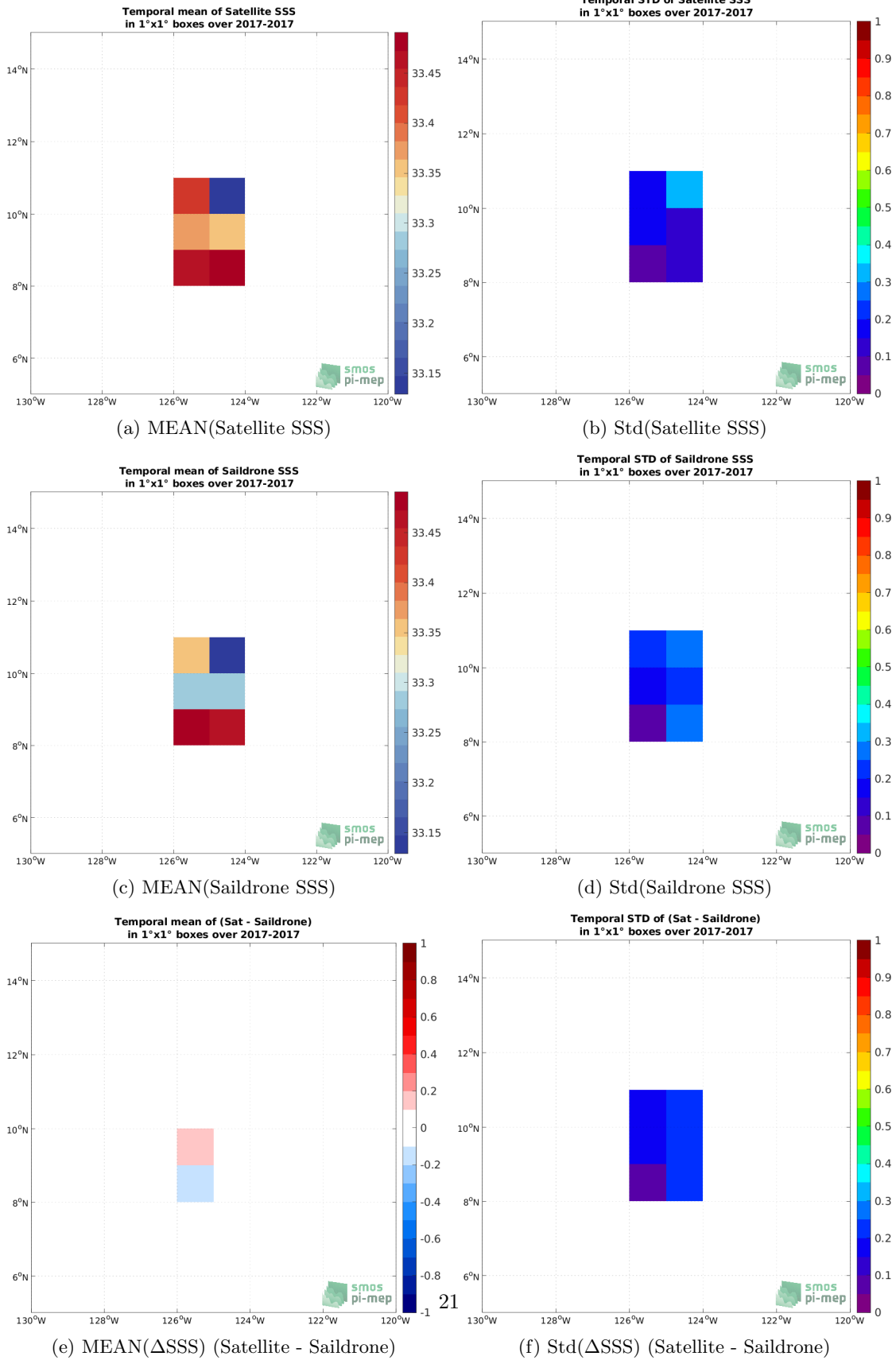
Figure 5: Temporal mean (left) and Std (right) of SSS from CCI SSS L4 Merged-OI v3.2 - 7-day running (ESA) (top), Saildrone (middle), and of \Delta SSS (Satellite - Saildrone). Only match-up pairs are used to generate these maps.
