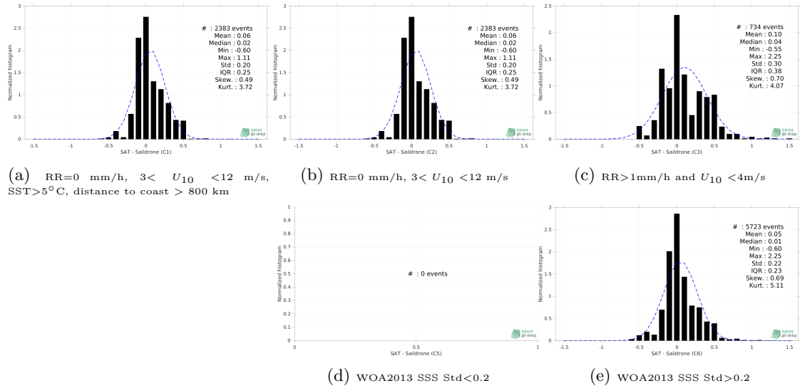
Figure 12: Normalized histogram of \Delta SSS (CCI SSS L4 Merged-OI v3.2 - 7-day running (ESA) - Saildrone) for 5 different subdatasets corresponding to: RR=0 mm/h, 3 < U_{10} < 12 m/s, SST > 5°C, distance to coast > 800 km (a), RR=0 mm/h, 3 < U_{10} < 12 m/s (b), RR > 1mm/h and U_{10} < 4 m/s (c), WOA2013 SSS Std < 0.2 (d), WOA2013 SSS Std > 0.2 (e).
