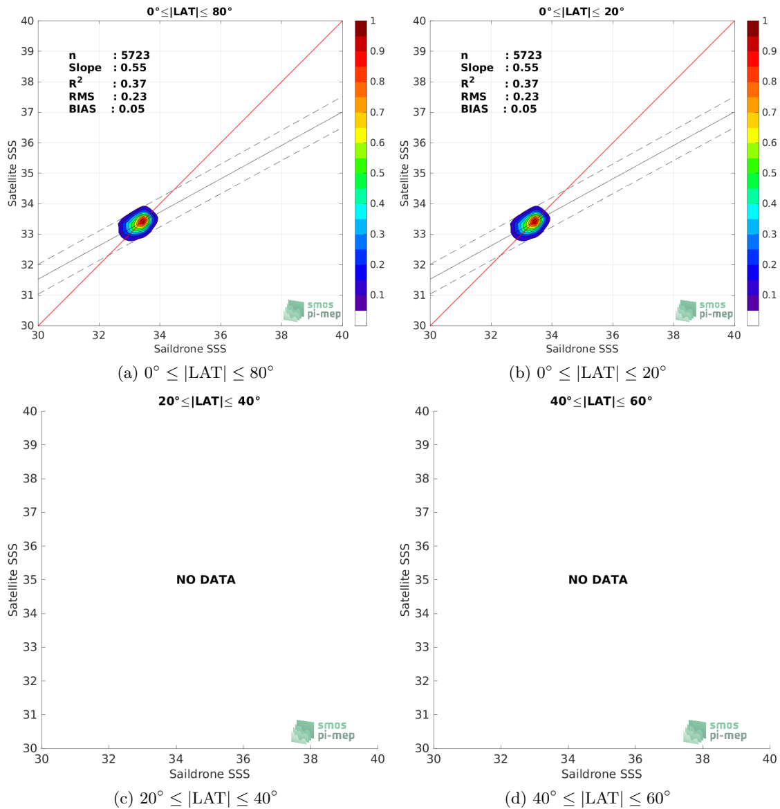
Figure 8: Contour maps of the concentration of CCI SSS L4 Merged-OI v3.2 - 7-day running (ESA) SSS (y-axis) versus SAILDRONE SSS (x-axis) at match-up pairs for different latitude bands. For each plot, the red line shows x=y . The black thin and dashed lines indicate a linear fit through the data cloud and the \pm 95\% confidence levels, respectively. The number match-up pairs n , the slope and R^2 coefficient of the linear fit, the root mean square (RMS) and the mean bias between satellite and in situ data are indicated for each latitude band in each plots.
