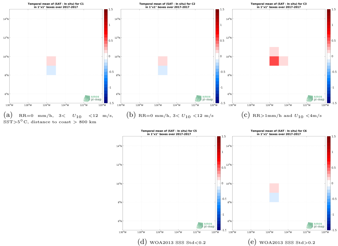
Figure 11: Temporal mean gridded over spatial boxes of size 1^\circ \times 1^\circ of \Delta SSS (CCI SSS L4 Merged-OI v3.2 - 7-day running (ESA) - Saildrone) for 5 different subdatasets corresponding to:RR=0 mm/h, 3 < U_{10} < 12 m/s, SST >5^\circ C, distance to coast > 800 km (a), RR=0 mm/h, 3 < U_{10} < 12 m/s (b), RR >1 mm/h and U_{10} < 4 m/s (c), WOA2013 SSS Std <0.2 (d), WOA2013 SSS Std >0.2 (e).
