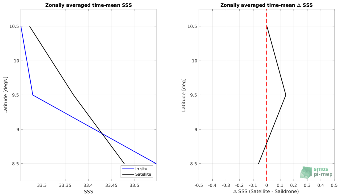
Figure 7: Left panel: Zonal mean SSS from CCI SSS L4 Merged-OI v3.2 - 7-day running (ESA) satellite product (black) and from Sairdrone (blue). Right panel: Zonal mean of \Delta SSS (Satellite - Sairdrone) for all the collected Pi-MEP match-up pairs estimated over the full satellite product period.
