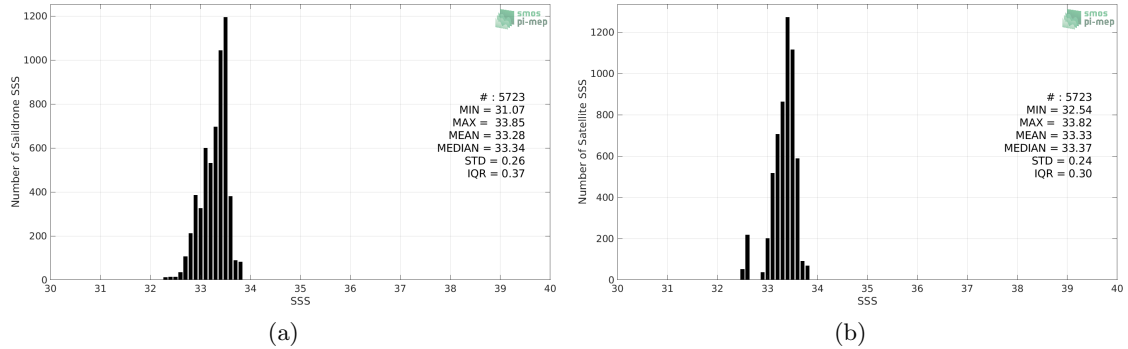
Figure 2: Histograms of SSS from Sairdrone (a) and CCI SSS L4 Merged-OI v3.2 - 7-day running (ESA) (b) considering all match-up pairs per bins of 0.1 over the SPURS 2 Pi-MEP region and for the full satellite product period.
